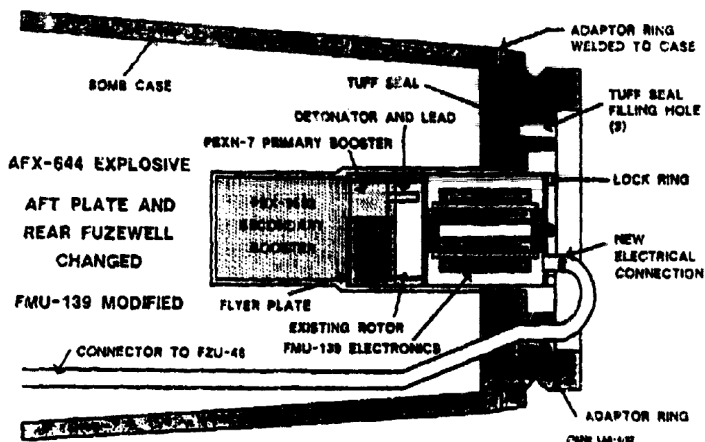
Figure 69: Mk-82 Bomb Modifications.
