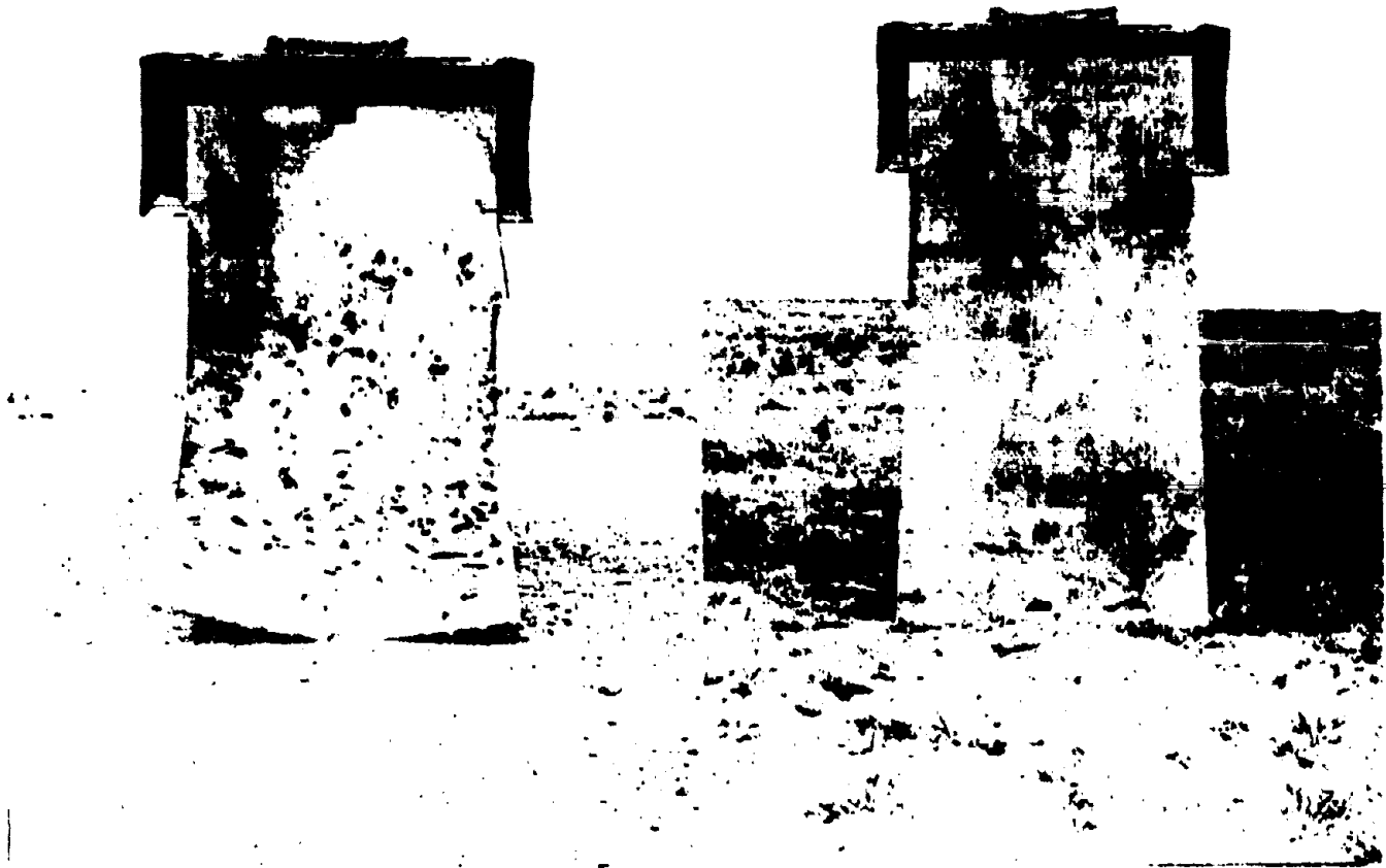
Figure 64: Side Witness Plates from AFX-644 Low Wax Asymmetrical Pallet Sympathetic Detonation Test
