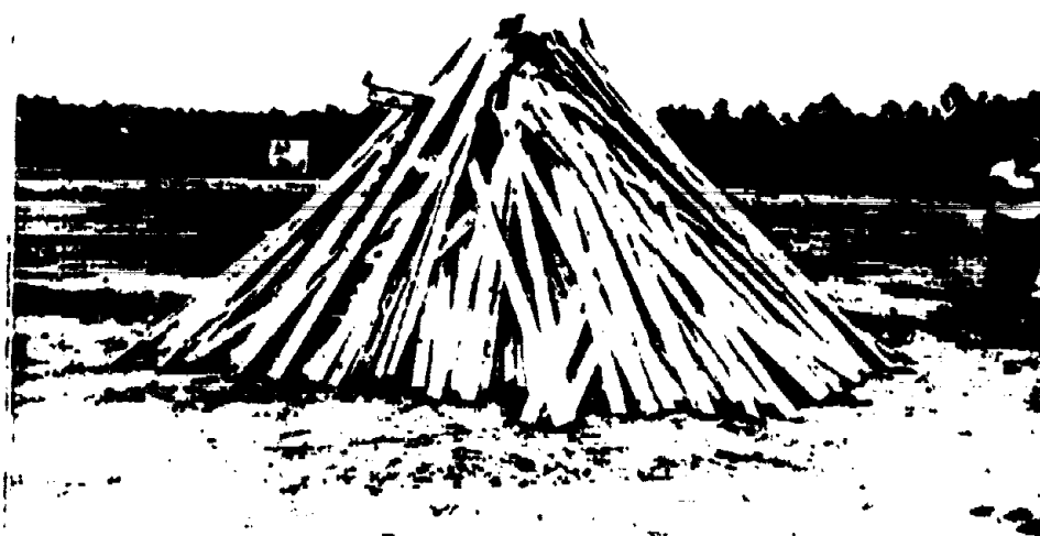
Figure 5: Wood Bonfire (Fast Cook-off) Test Before Ignition
