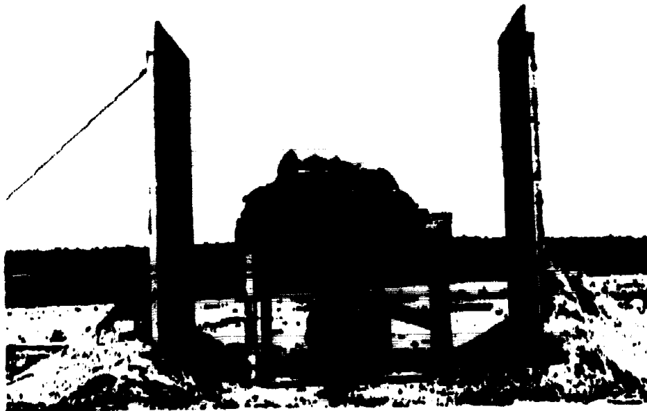
Figure 17: Sympathetic Detonation Test Set-Up
