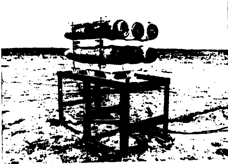
Figure 72: Three Bomb FIGPB Fuzed Fast Cook-off Test Set Up
