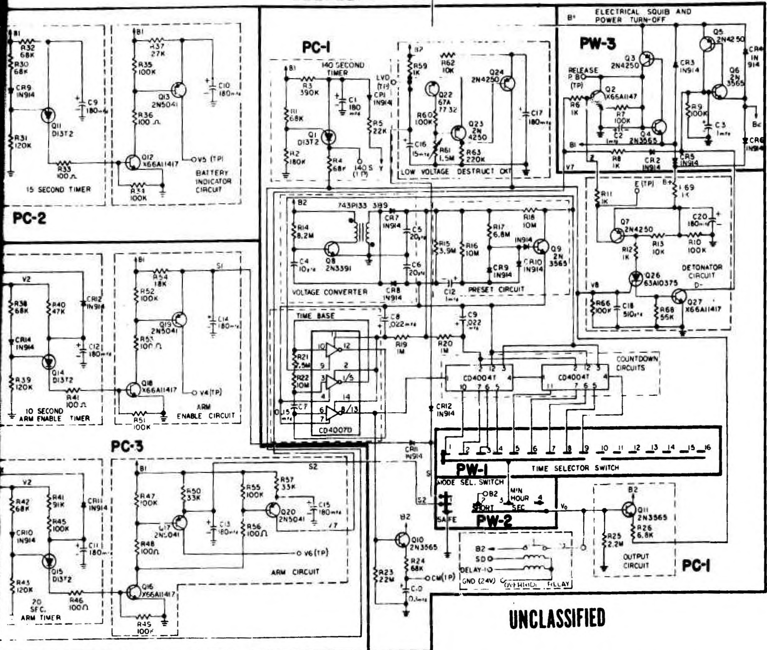
Figure 7. Schematic of VLD (Ground-Settable)
