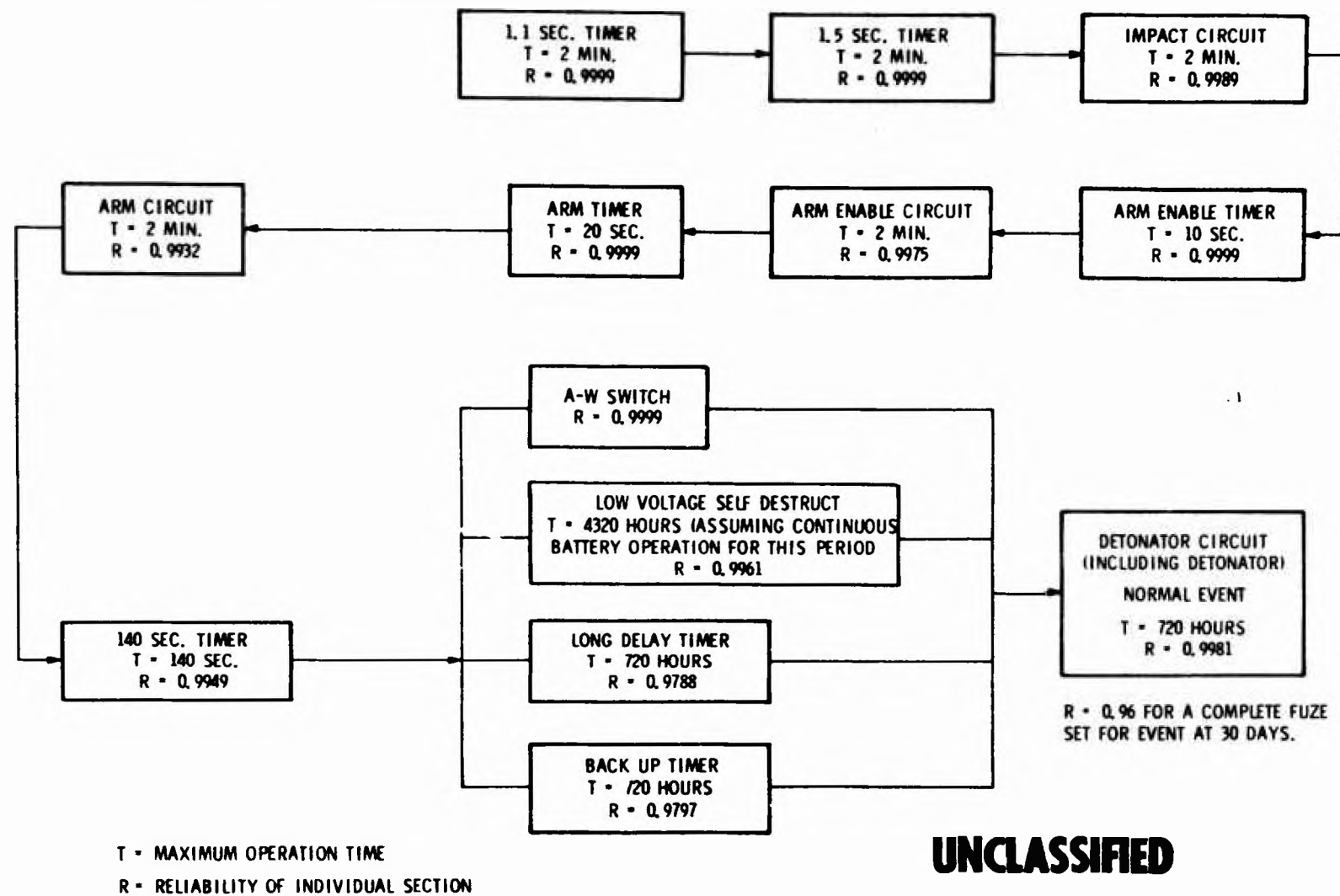
Figure 26. Reliability Diagram
