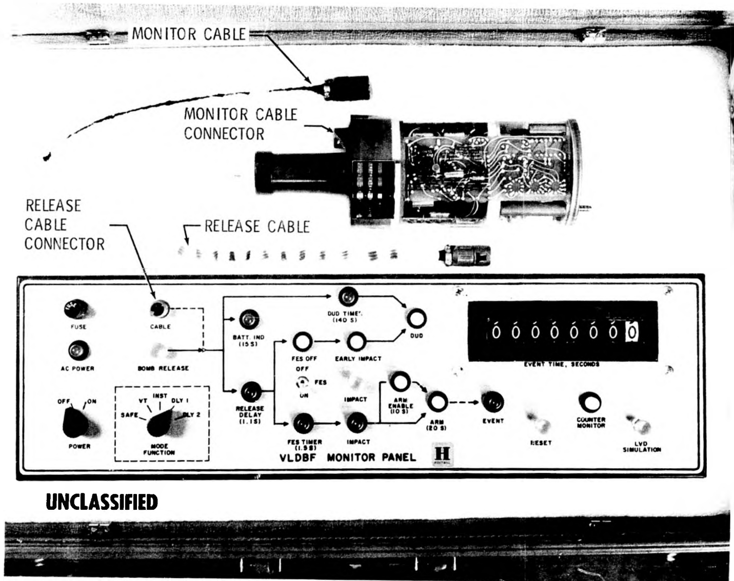
Figure 23. Cockpit-Settable Fuze Demonstration Unit, Showing Monitor Panel Layout
