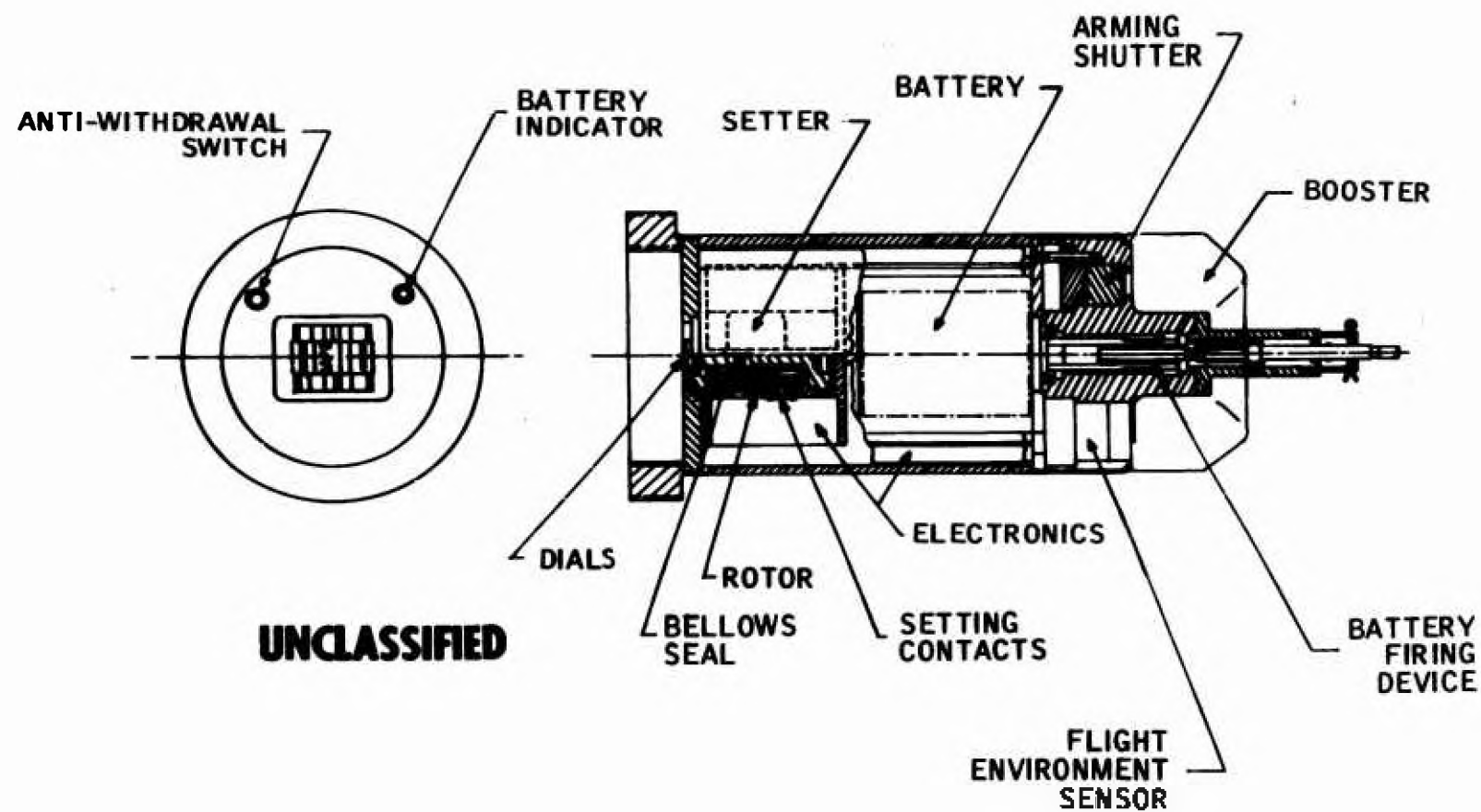
Figure 4. Ground-Settable Fuze, Overall Design
