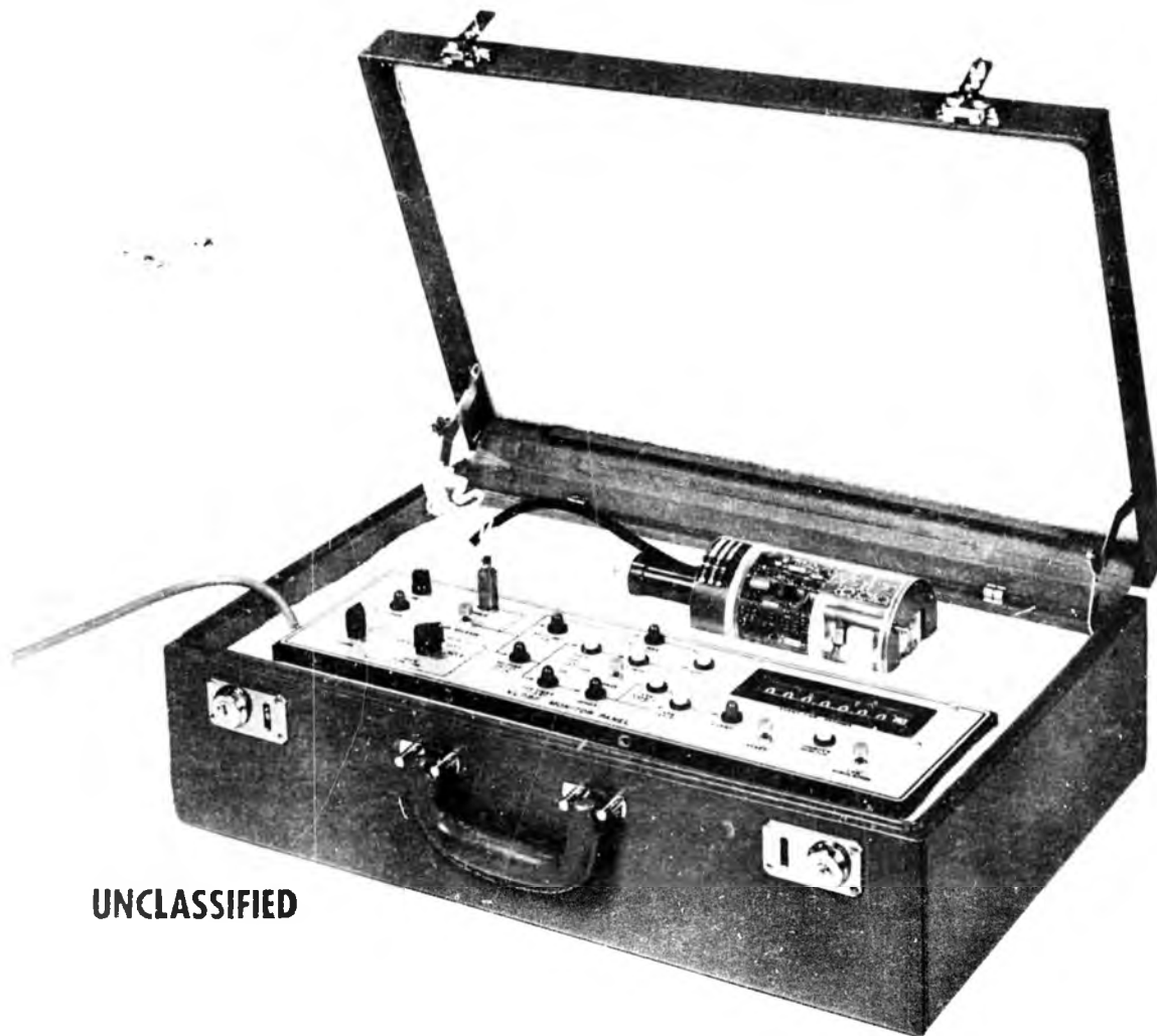
Figure 2. Very Long Delay Fuze, Cockpit Settable Model (Including Special Test Equipment)
