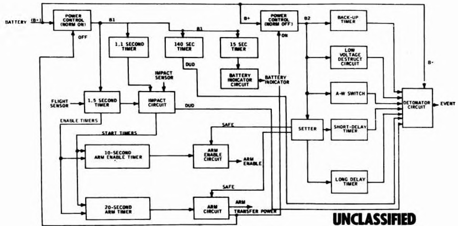
Figure 6. Block Diagram, Ground-Settable Fuze
