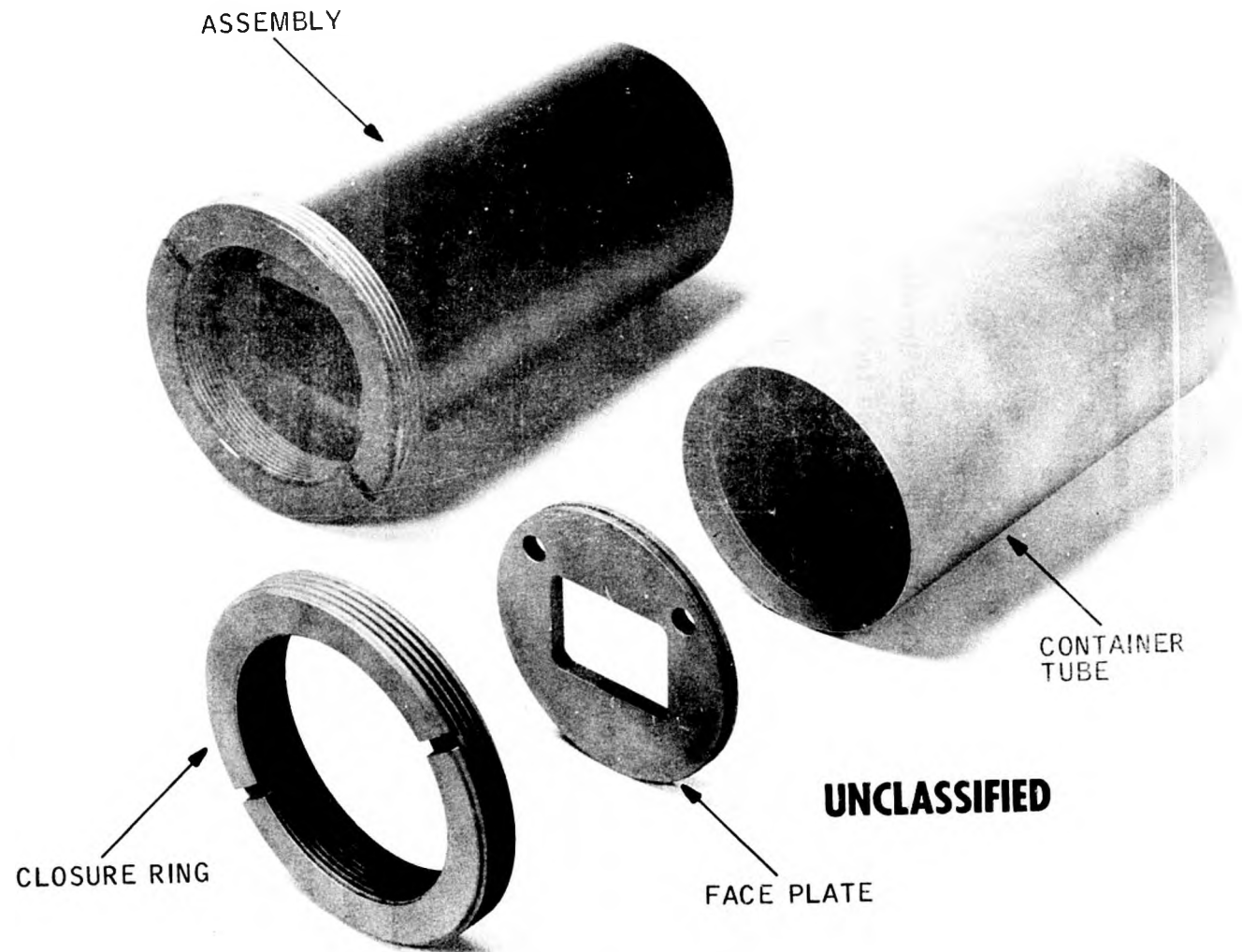
Figure 22, Container
