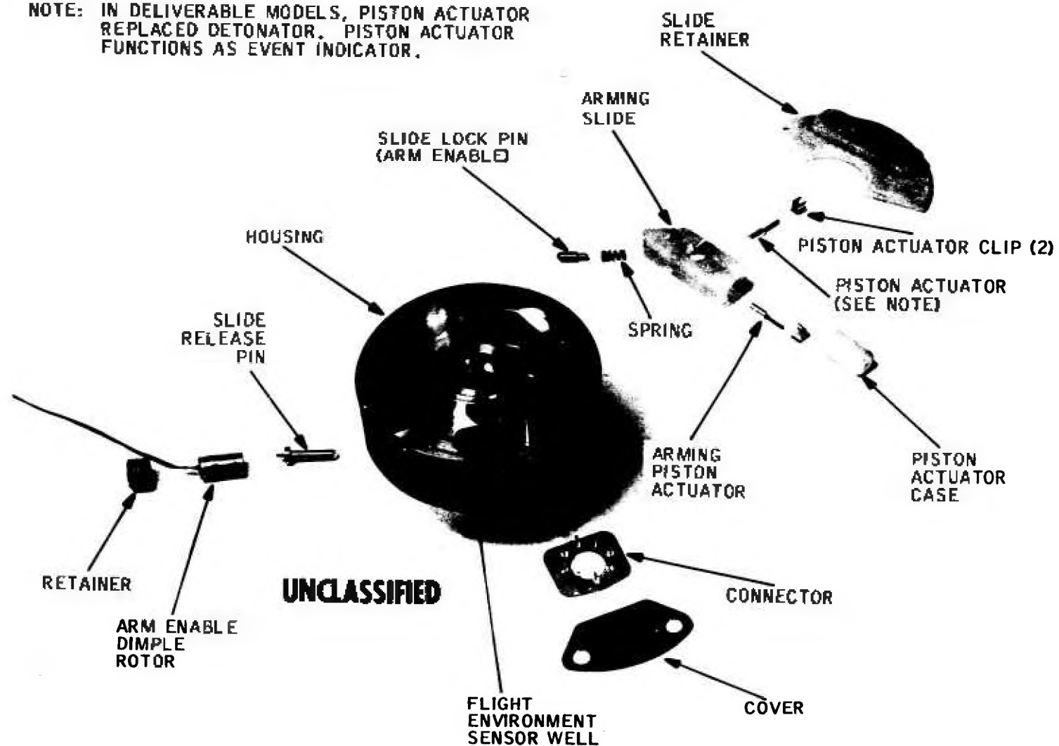
Figure 15. Safing and Arming Mechanism
