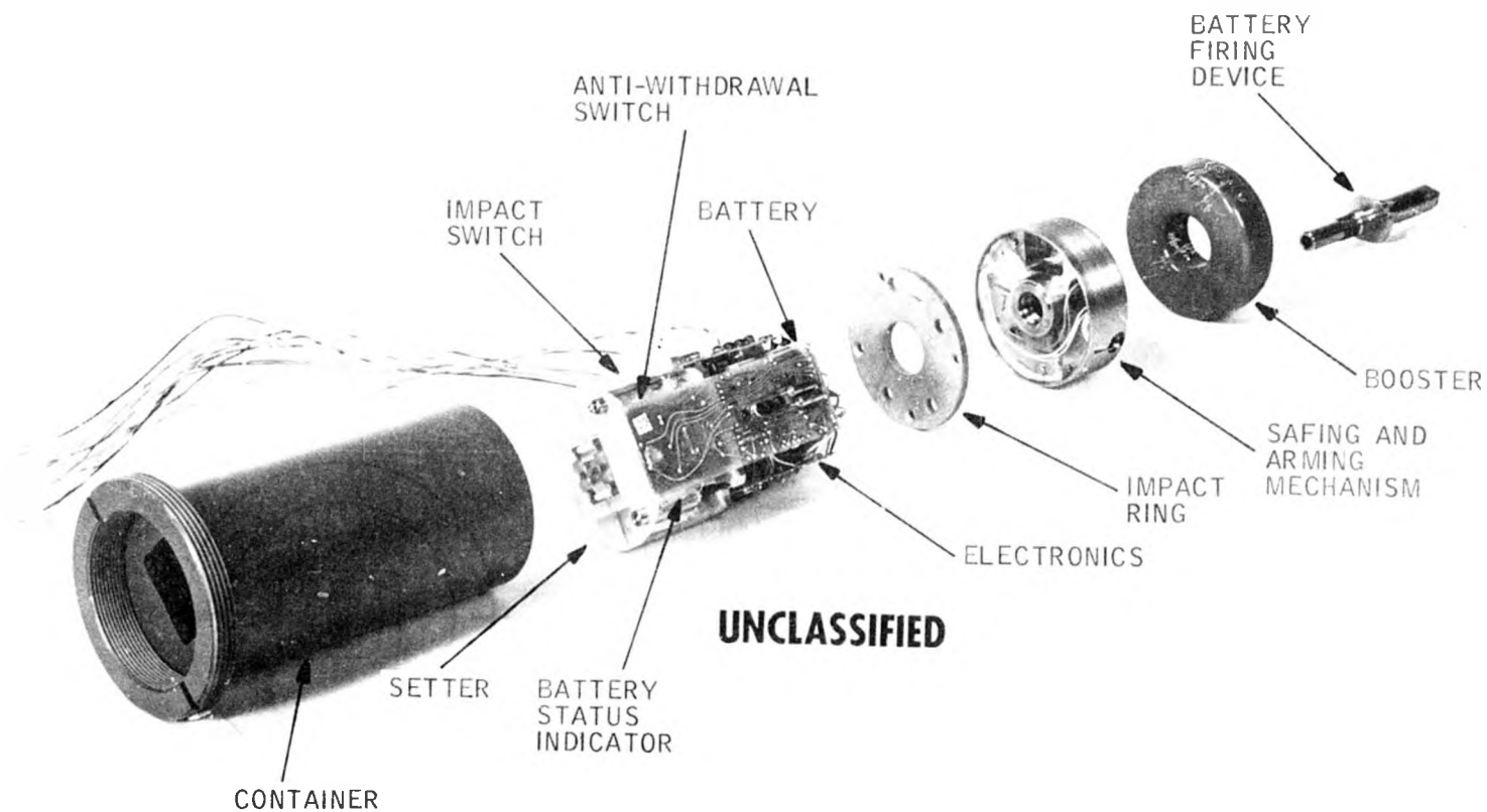
Figure 5. Very Long Delay Fuze, Ground-Settable Model, Major Components Shown in Order of Assembly
