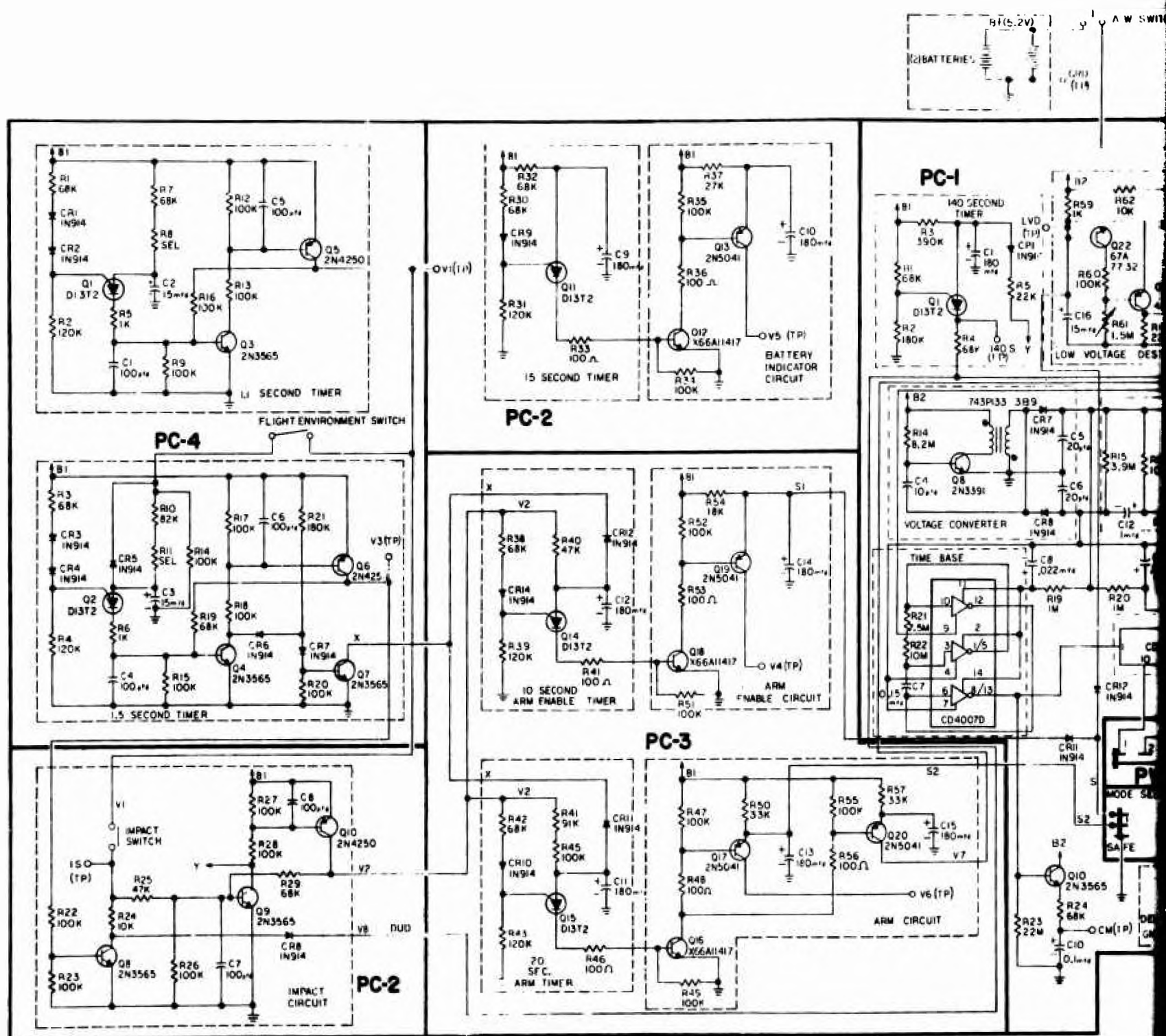
Figure 7. Schematic
