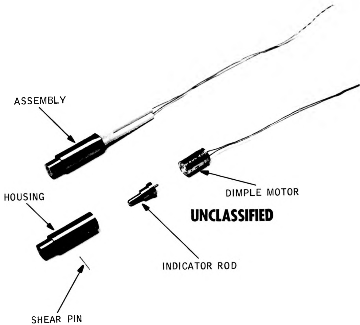
Figure 20. Battery Status Indicator
