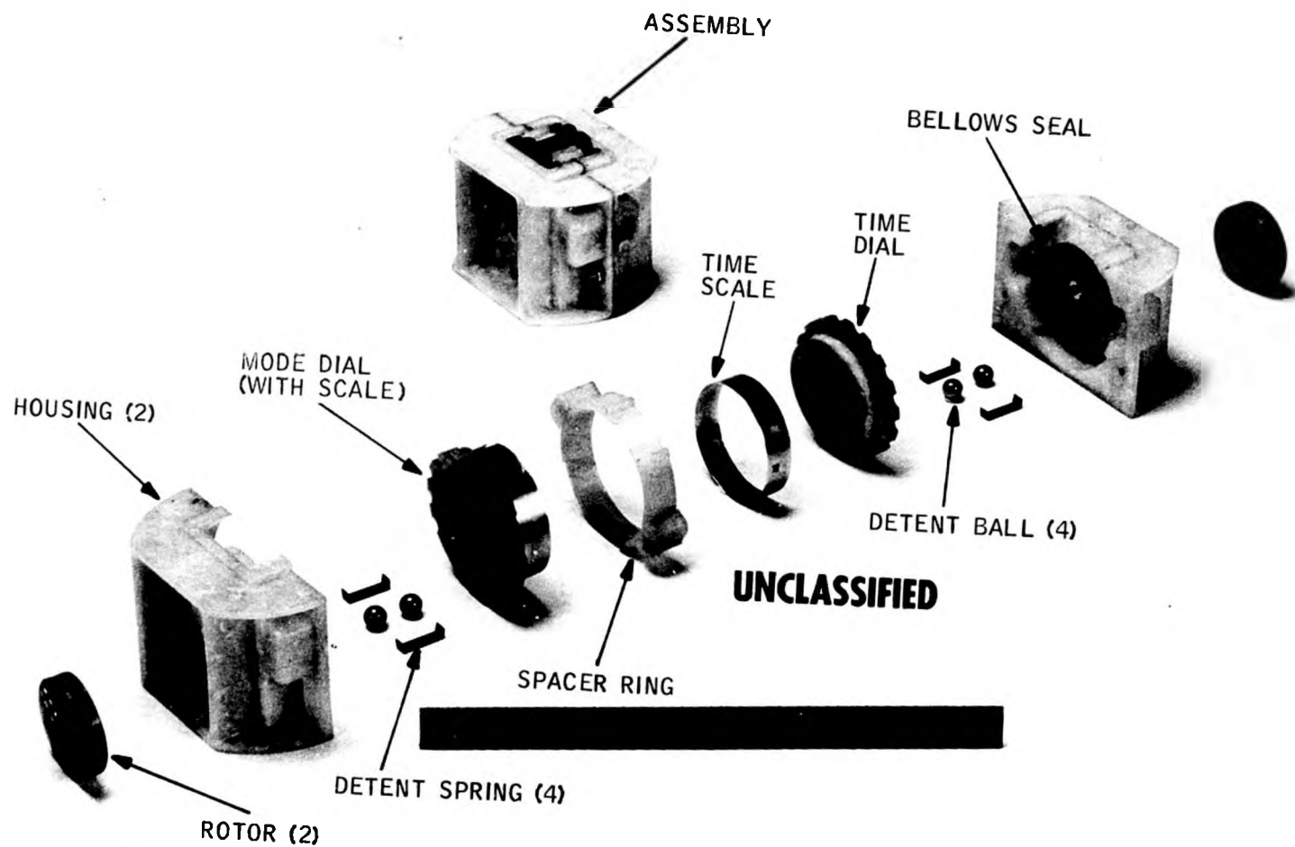
Figure 9. Setter
