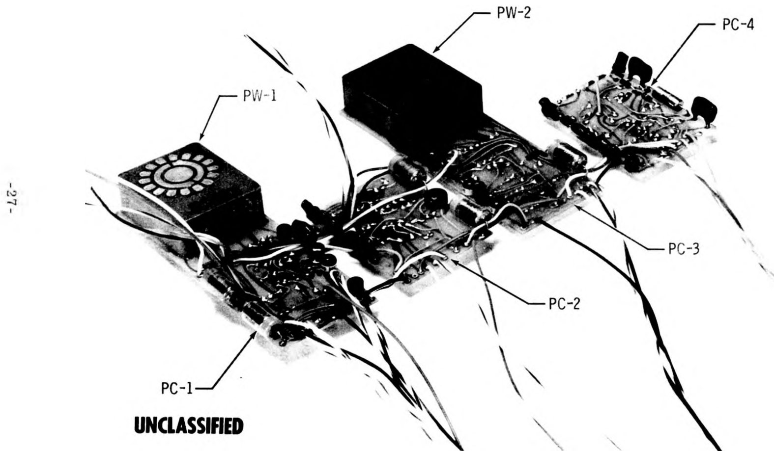
Figure 8. Packaging Concept, Electronic Circuits for Ground-Settable Fuze
