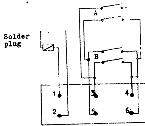
Figure 36 Wiring Diagram for Pausenuhr
