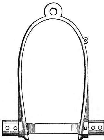
Dahlgren breech strap for 7 \frac{1}{2} -in. rifle. Scale, \frac{1}{16} in. to 1 ft.
