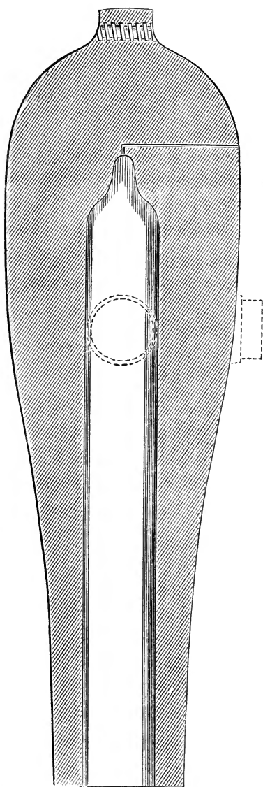
U. S. Navy 15-in. gun. Scale, \frac{7}{16} in. to 1 ft.
