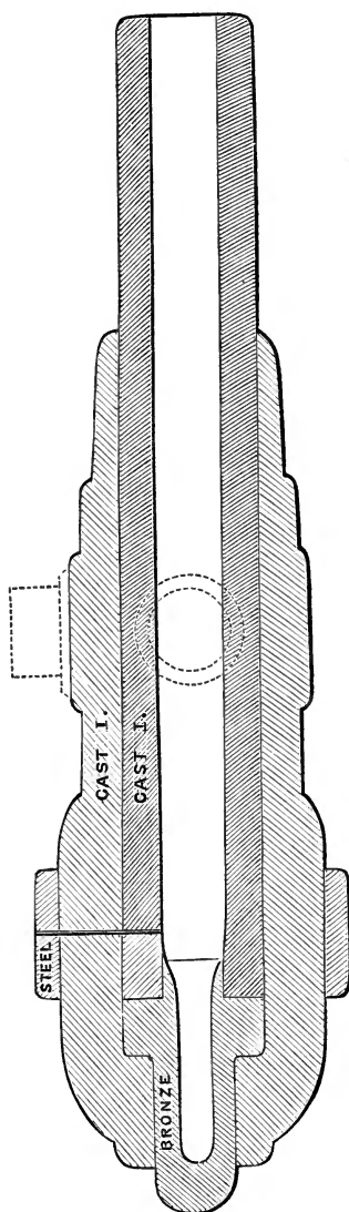
FIG. 34.—Blakely 900-pdr. ( 12\frac{3}{4} in.) rifle, sent to Charleston. Scale, \frac{7}{16} in. to 1 ft.
