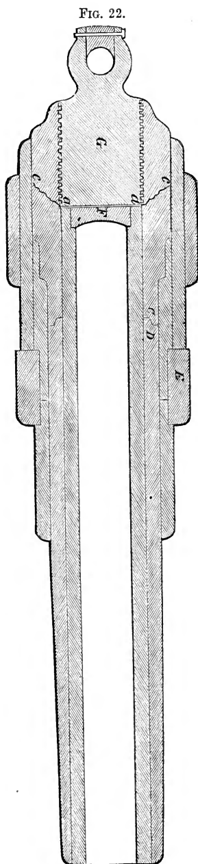
Armstrong 10\frac{1}{2} in. gun. \frac{7}{16} in. to 1 ft.
