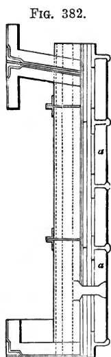
Section of Mr. Scott Russell's target. Scale, \frac{1}{4} in. to 1 ft.
