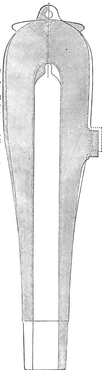
FIG. 78.—U. S. Army and Navy 13-in. guns. Half section of each. Scale, \frac{7}{16} in. to 1 ft.
