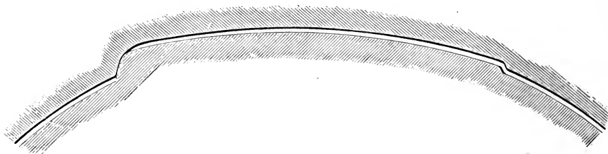
Full-sized section Scott's rifling; projectile leaving the gun.
