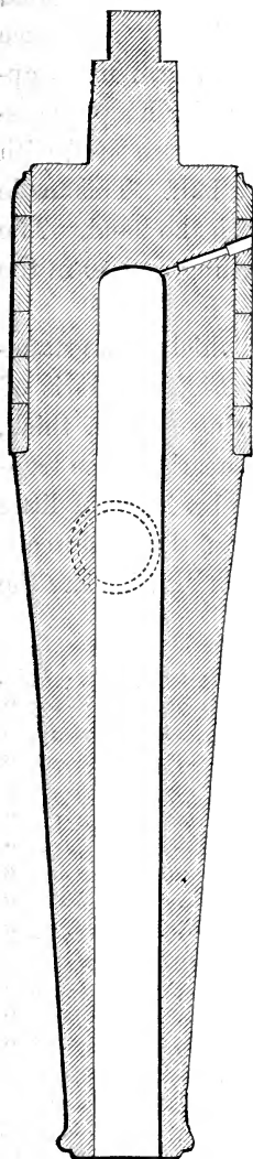
Spanish steel hooped gun. Scale, \frac{1}{10} in. to 1 foot.
