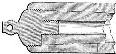
Section of breech of Whitworth muzzle-loader.
