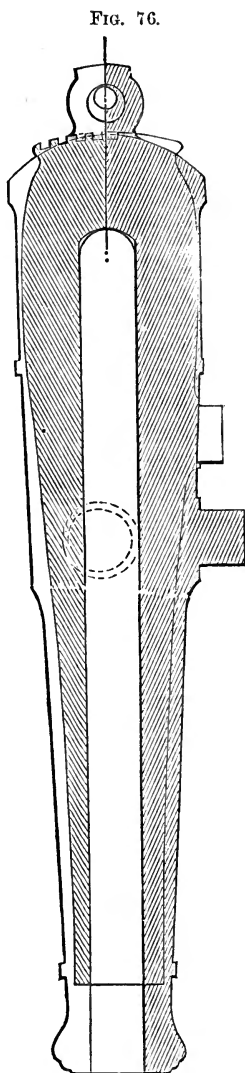
Section of British 8-in. (68-pdr.) laid over section of U. S. 8-in. Columbiad. Scale, \frac{1}{16} in. to 1 ft.
