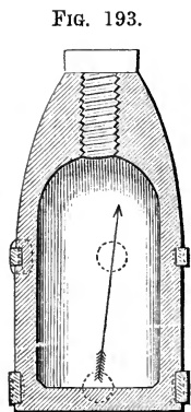
Beaulieu's, or first French service rifle shot.
