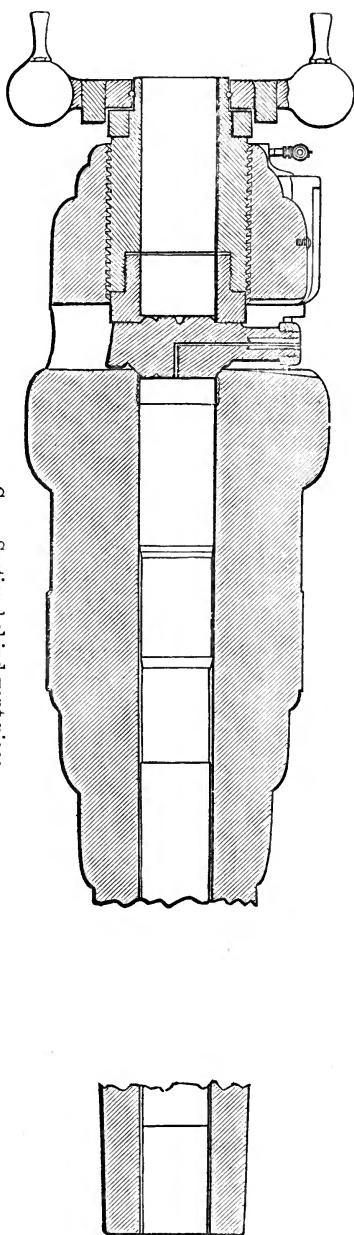
Fig. 18. Section of breech of 110-pounder—scale \frac{1}{4} in. to 1 ft.
