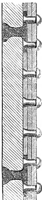
FIG. 107.—Section of Mr. Scott Russell's armor.
