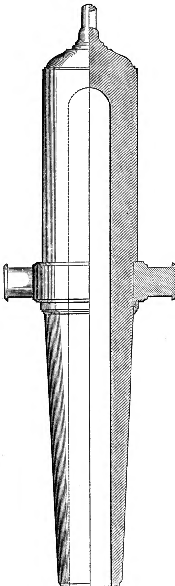
The Mersey 12-inch gun in the Brooklyn Navy Yard. Scale, \frac{1}{8} in. to 1 ft.
