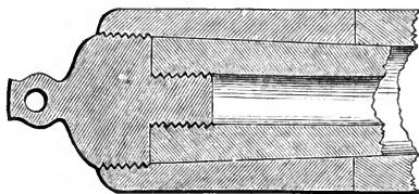
Breech-screw of Whitworth gun.
