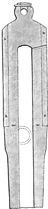
Armstrong hooped cast-iron naval gun. Scale, \frac{6}{10} in. to 1 ft.
