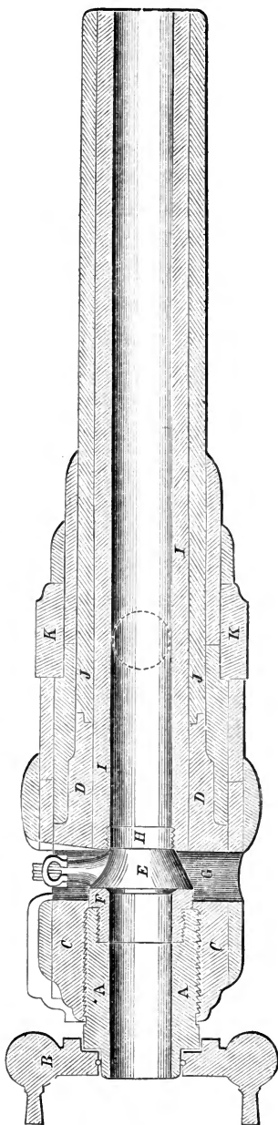
FIG. 344.—Longitudinal section of Armstrong 110-pounder. Scale, \frac{7}{8} in. to 1 ft.
