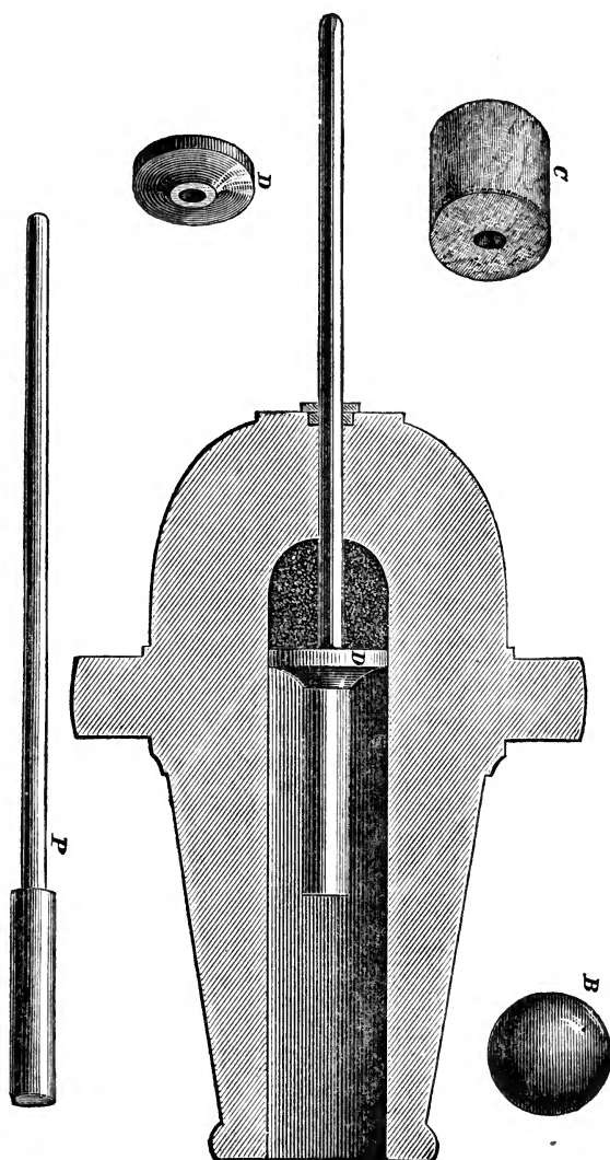
FIGS. 287 A to 287 E.—Bates and Macy's ordnance and projectiles.
