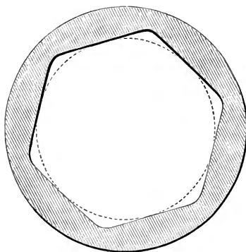
Whitworth's rifling.
