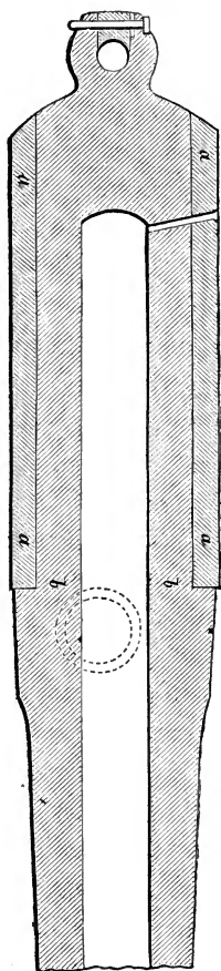
Armstrong hooped cast- iron naval gun. Scale, \frac{6}{10} in. to 1 ft.
