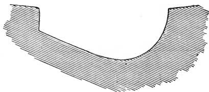
Groove of Blakely 12 \frac{3}{4} -in. gun. Full size.
