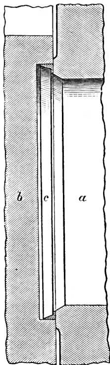
Krupp's gas-check.
