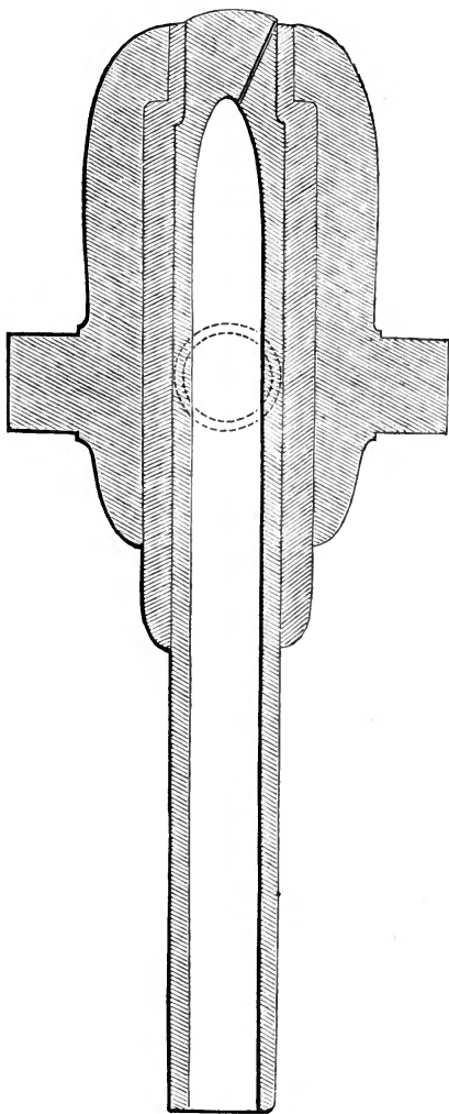
Blakely 9-inch high and low steel and cast-iron gun. Scale, \frac{7}{16} in. to 1 ft.
