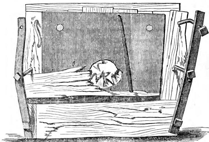
Front of 4\frac{1}{2} -in. plate, with 12-in. oak facing, after one 11-inch shot.
