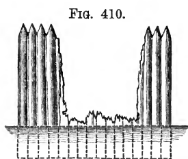
12 and 8-in. palisade cut down by 25 lbs. of gun-cotton.
