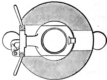
Cross section behind vent-piece.
