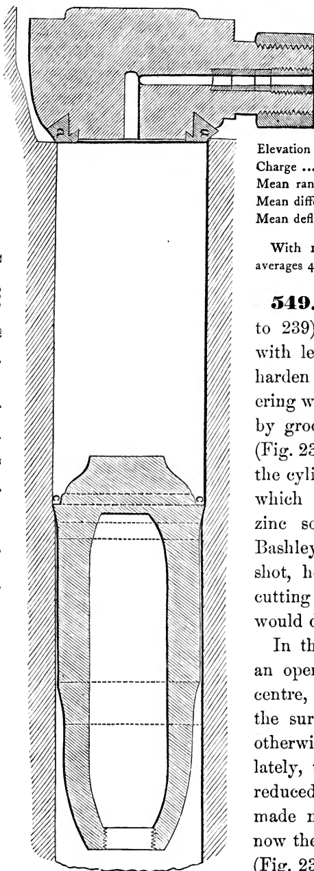
FIG. 236.—Chamber and projectile of 12-pounder. \frac{1}{2} size.
