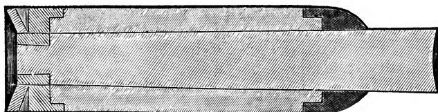
Stafford's sub-calibre shot.
