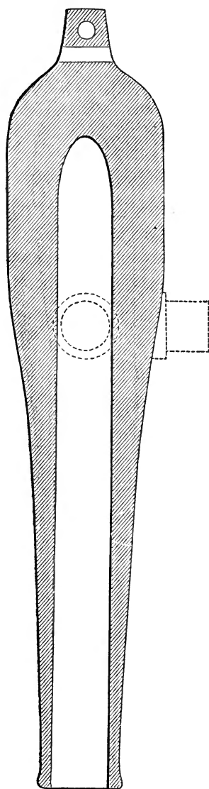
U. S. Navy 11-in. Dahlgren gun. Scale, \frac{7}{16} in. to 1 ft.
