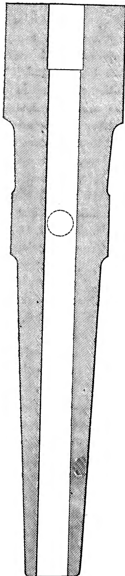
FIG. 69.—Section of Krupp's 9-inch solid steel gun in the Exhibition of 1862. Scale, \frac{1}{16} in. to 1 ft.
