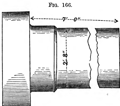
Forging for Mallet's mortar-chamber.
