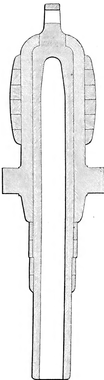
Fig. 32 D. Blakely's steel 8-inch 200-pounder. Scale, \frac{1}{16} in. to 1 ft.
