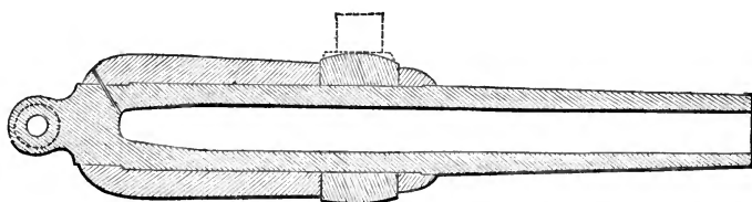
Blakely 5.8 inch steel rifle. Scale, \frac{7}{16} in. to 1 ft.
