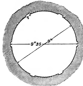
FIGS. 248 to 251.—Shunt rifling of Russian 9-in. gun. Scale, 1\frac{1}{2} in. to 1 ft.
