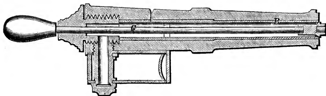
Adams's loading and cooling from the breech.
