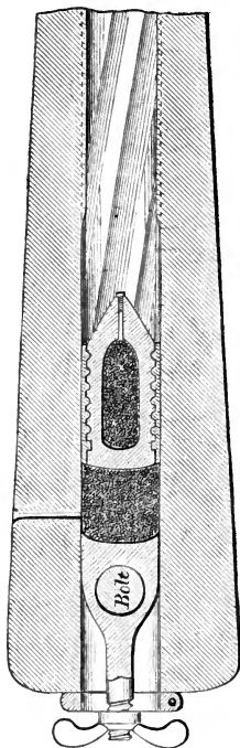
Fig. 367 and 368.—The Warendorf breech-loader.
