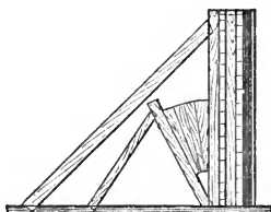
Side of 10-in. target for 15-in. gun. Scale, \frac{1}{16} in to 1 ft.
