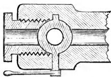
Alger's breech-loader.
