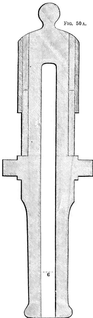
Armstrong cast-iron 70-pounder of 1860. Scale \frac{1}{16} in. to 1 ft.
