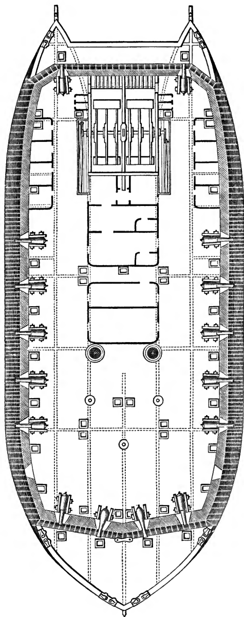
THE MISSISSIPPI IRON-CLAD "BENTON."
