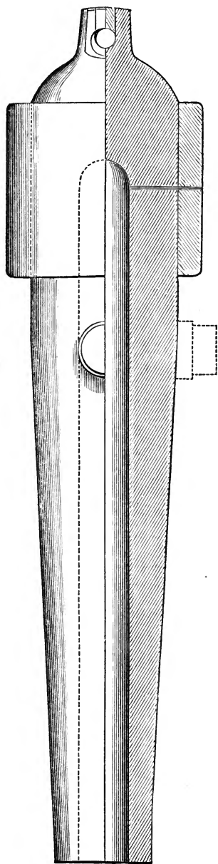
FIG. 44. Parrott 10-inch rifle. \frac{7}{8} in. to 1 ft.
