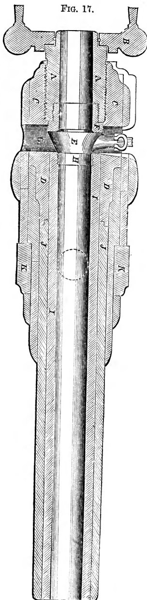
Armstrong 110-pounder. \frac{6}{10} in. to 1 ft.
