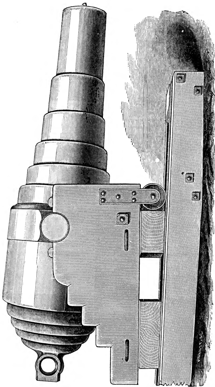
ARMSTRONG 600-POUNDER.
