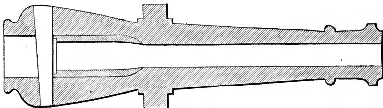
Cavalli breech-loader.
