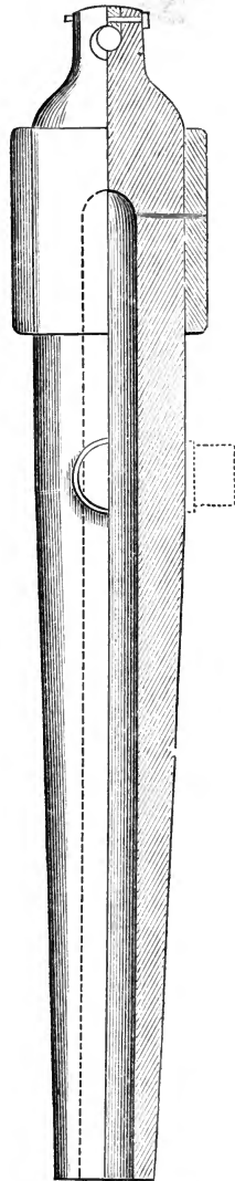
Parrott 6.4 inch "100-pounder" rifle, \frac{7}{16} in. to 1 ft.
