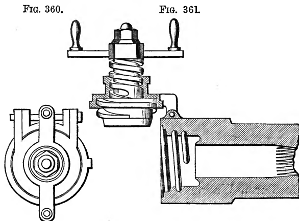
Screw breech-loader.
