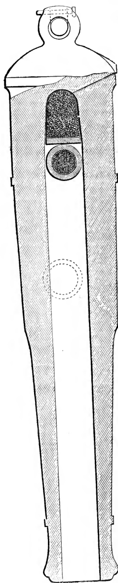
British 8-in. shell gun. Scale, \frac{1}{16} in. to 1 ft.
