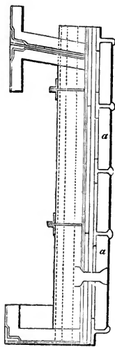
Scott Russell's target. Section. Scale, \frac{1}{4} in. to 1 ft.
