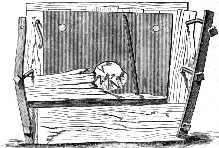
4\frac{1}{2} in. plate, with wood backing and facing.
