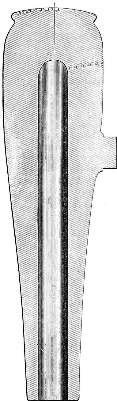
FIG. 77.—U. S. Army 15-in. Columbiad. Scale, \frac{7}{16} in. to 1 ft.
