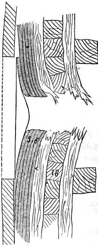
Section of 6\frac{1}{2} -in. laminated target.
