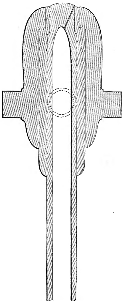
Blakely's 9-inch rifle. Low steel bore, hooped by high steel and cast iron. Scale, \frac{7}{8} in. to 1 ft.
