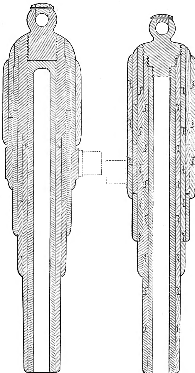
FIG. 27. 7-in. gun as built at Woolwich and rifled for Mr. Whitworth. Scale \frac{6}{10} in. to 1 ft.
