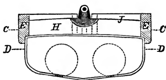
Cross section of the Naugatuck .
