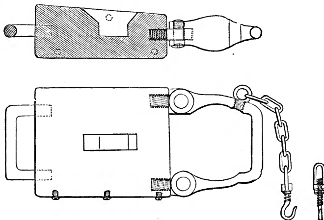
Cavalli breech-loader.
