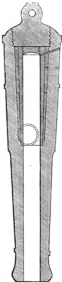
68-pounder, strengthened by Parsons's internal tube. Scale, \frac{7}{16} in. to 1 ft.
