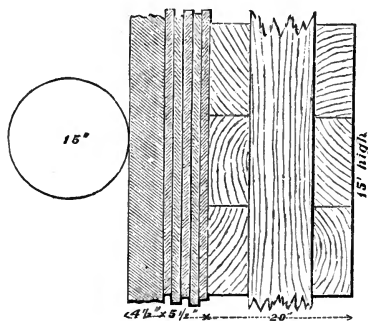
Section of 10-in. target and backing.
