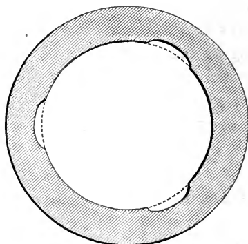
French rifling, 1860.
