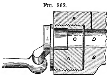
Clay's breech-loader.
