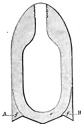
Britten's early projectile.
