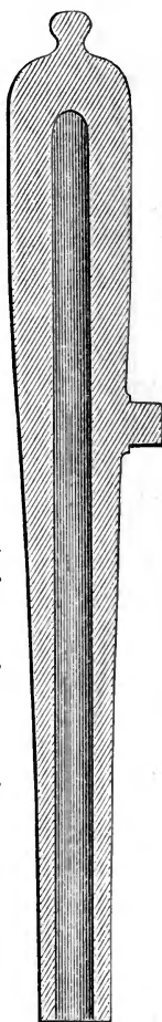
U. S. A. 4.2 in. siege-rifle. Scale, \frac{1}{16} in. to 1 ft.
