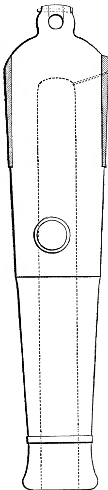
68-pounder, hooped at Woolwich. Scale, \frac{6}{10} in. to 1 ft.
