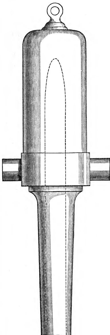
The "Prince Alfred" 10-in. wrought-iron hollow-forged gun. Scale, \frac{1}{8} in. to 1 ft.
