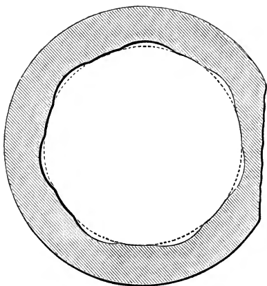
Jeffery's rifling.
