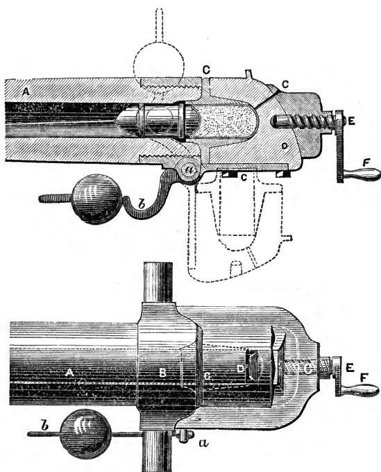
Storm's breech-loader.
