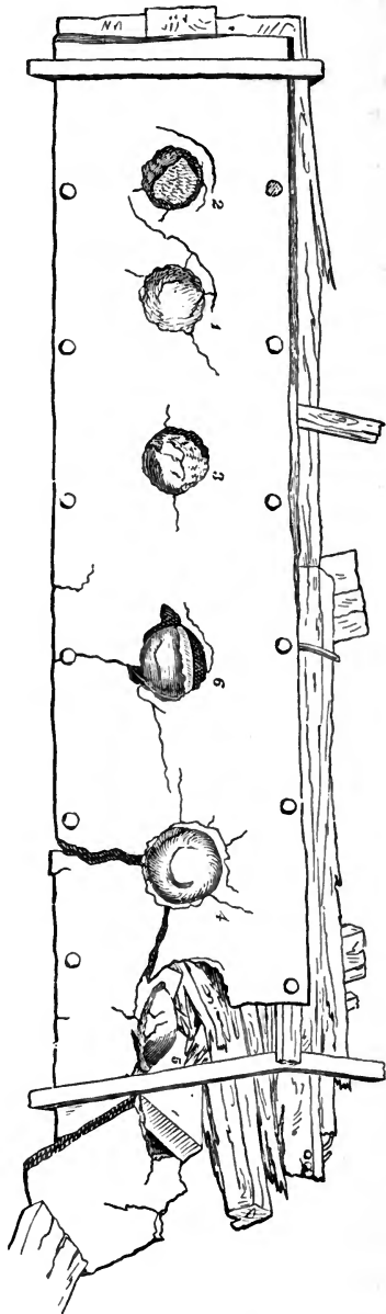
Nashua 4½-in. plate, after six 11-in. shot.
