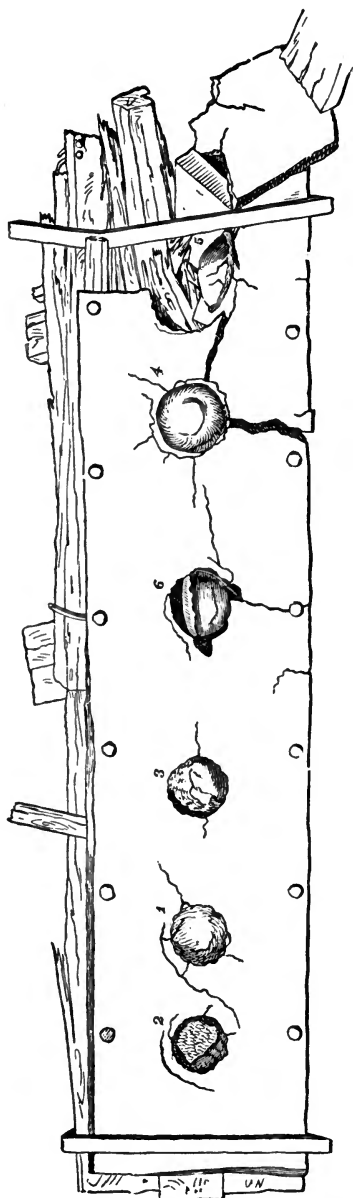
Front of Nashua target after six 11-in. shot with 30 lbs. powder at 30 yards.
