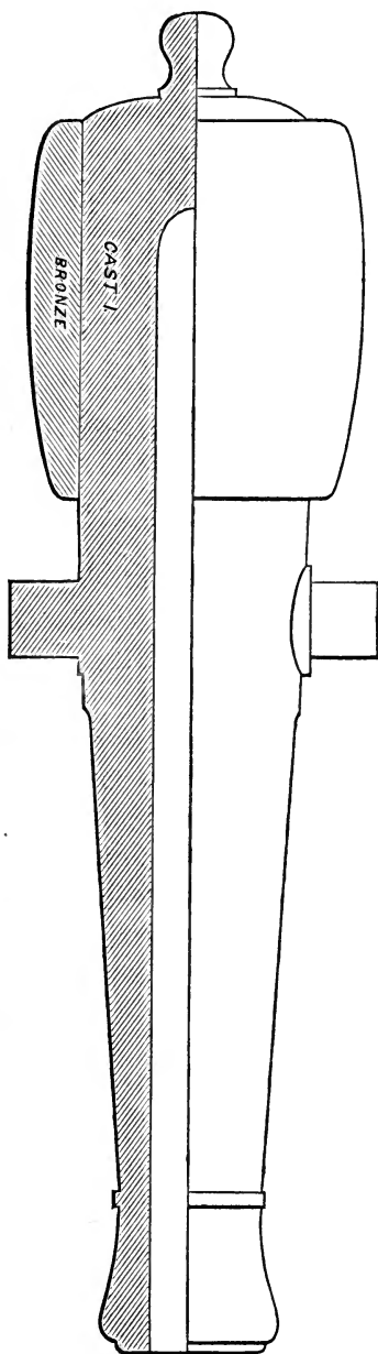
FIG. 59.—Attick's bronze reinforce. 100-pounder Scale \frac{1}{10} in. to 1 ft.
