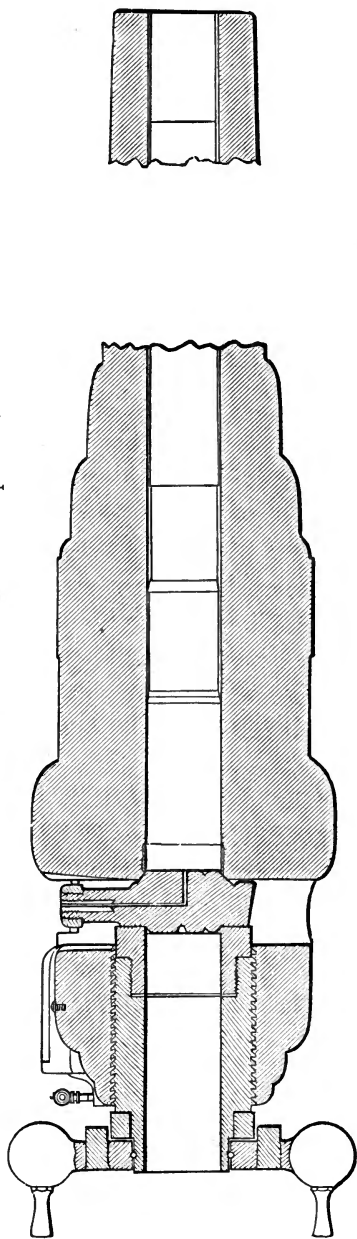
Fig. 340.—Section of breech of 110-pounder.
