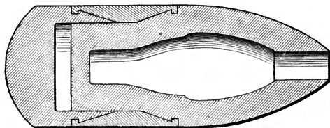
Section of the Hotchkiss shell
