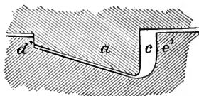
Scott's groove and rib.
