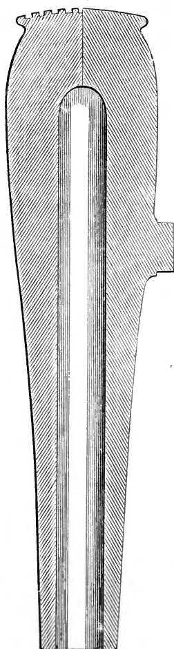
U. S. Army 10-in. Columbiad. Scale, \frac{1}{16} in. to 1 ft.
