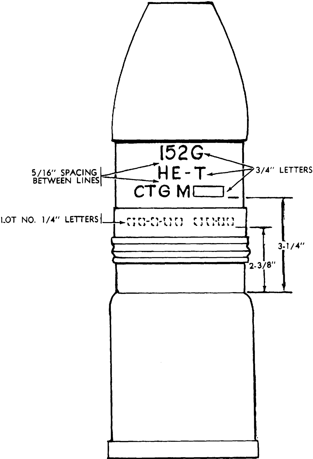
Figure E-79. Typical marking for 152mm gun cartridge M657.
