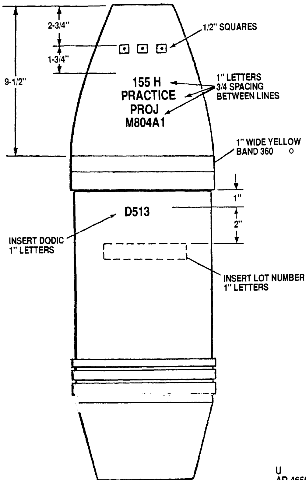
Figure E-83. Typical marking for 155mm howitzer projectile M804A1.
