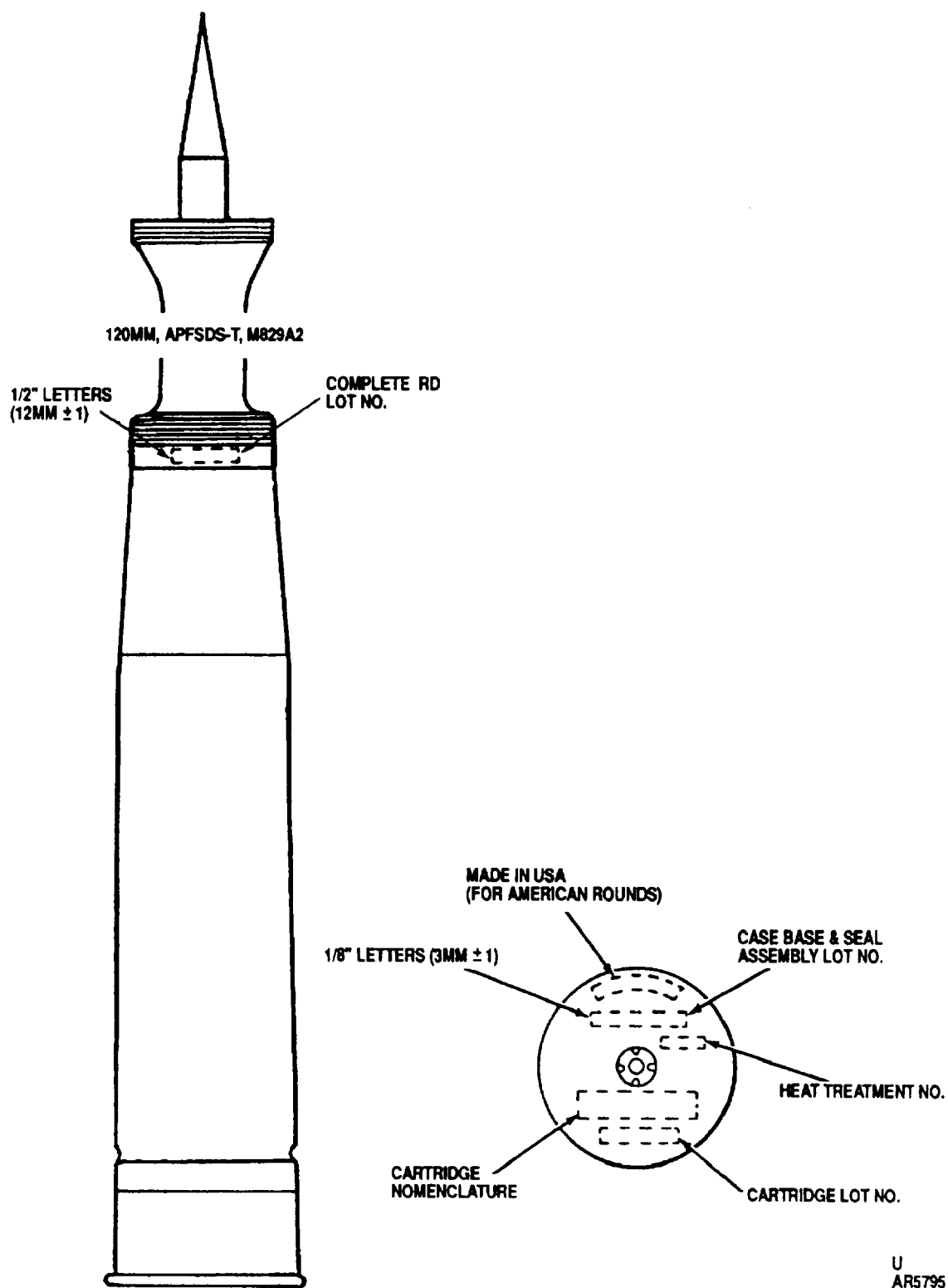
E-67. Typical marking for 120mm gun cartridges M829A2.
