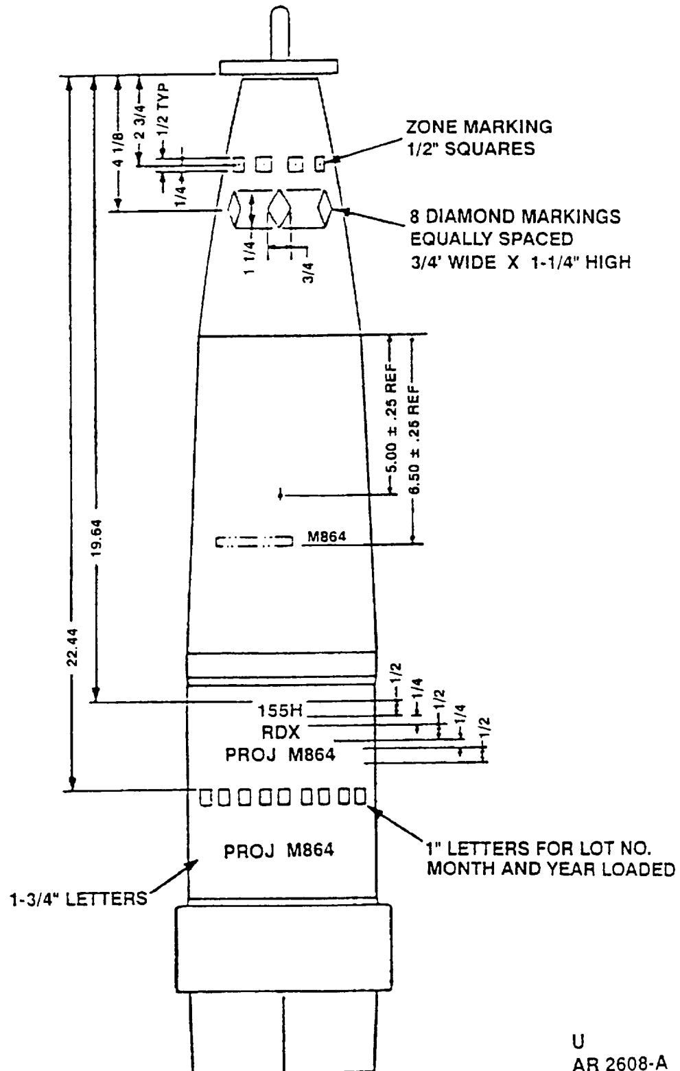
Figure E-104. Typical marking for 155mm howtizer projectile, M864.
