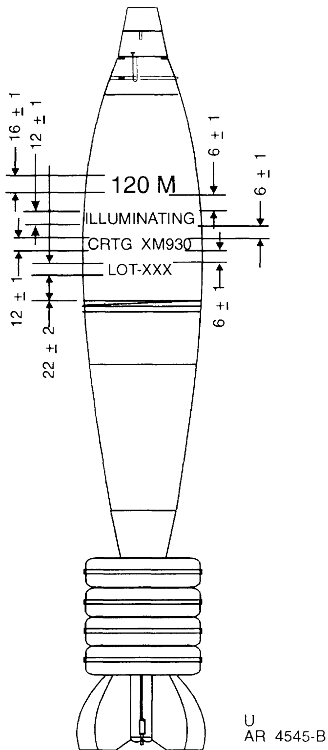
Figure E-76. Typical marking for 120mm mortar cartridge XM930.
