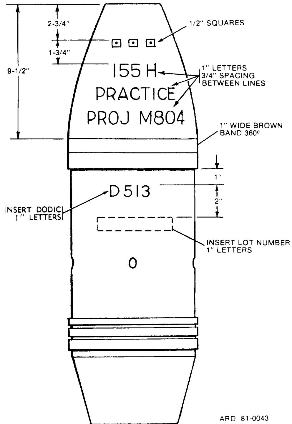
Figure E-82. Typical marking for 155mm howitzer projectile M804.
