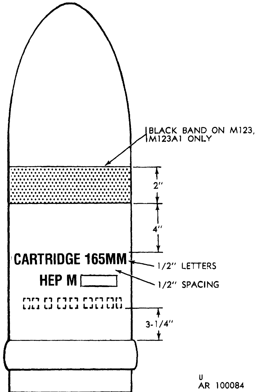
Figure E-97. Typical marking for 165mm gun projectiles M123 series and M623.
