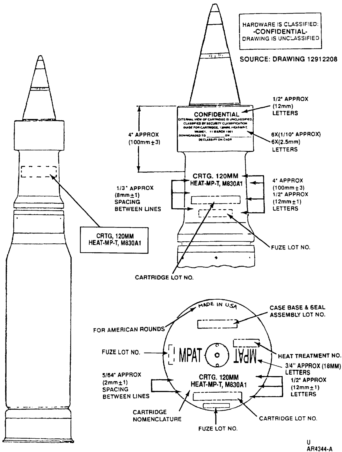
Figure E-69. Typical marking for 120mm gun cartridge HEAT-MP-T, M830A1.
