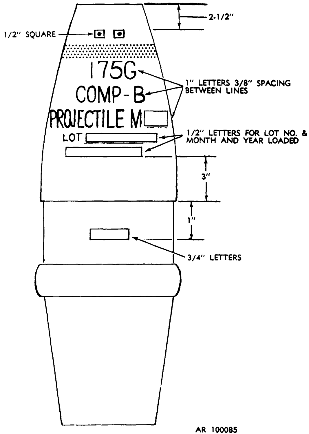
Figure E-98. Typical marking for 175mm gun projectile.
