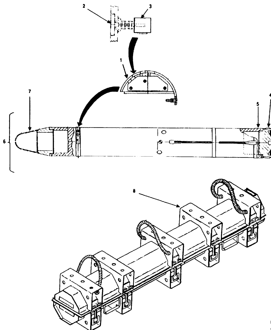
FIGURE C1. PROJECTILE, 155MM:
