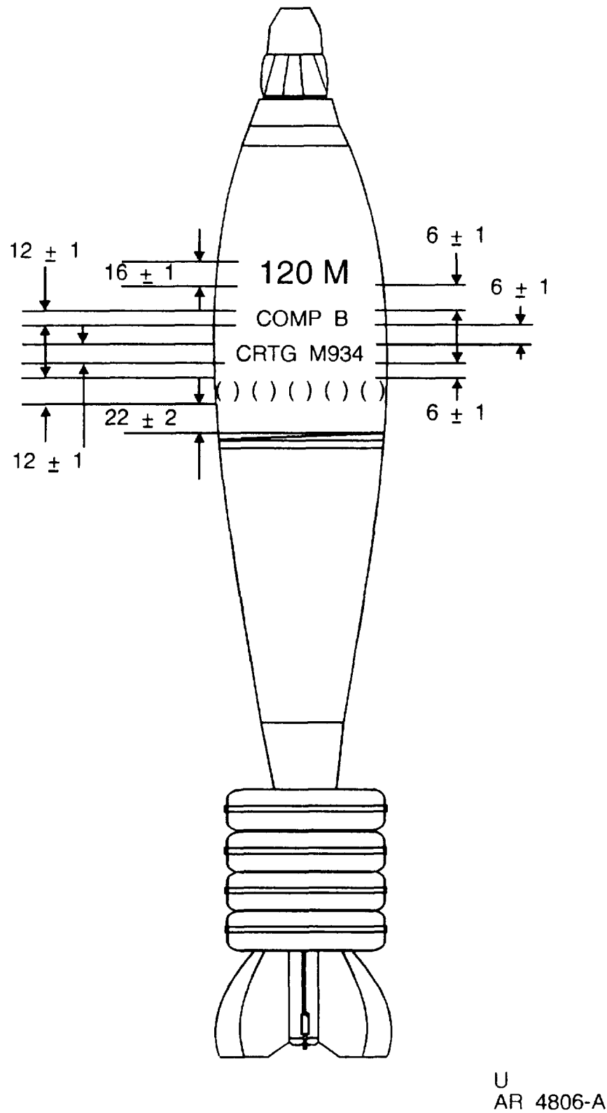
Figure E-75. Typical marking for 120mm mortar cartridge M934.
