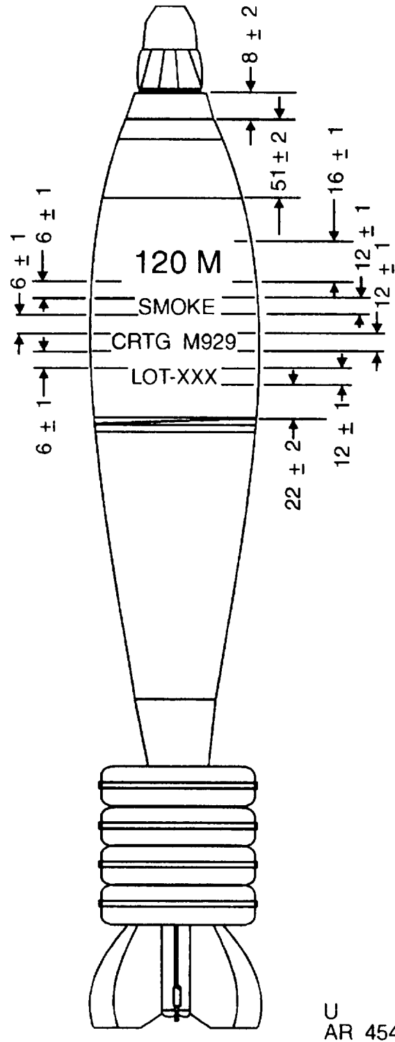
Figure E-77. Typical marking for 120mm mortar cartridge XM929.
