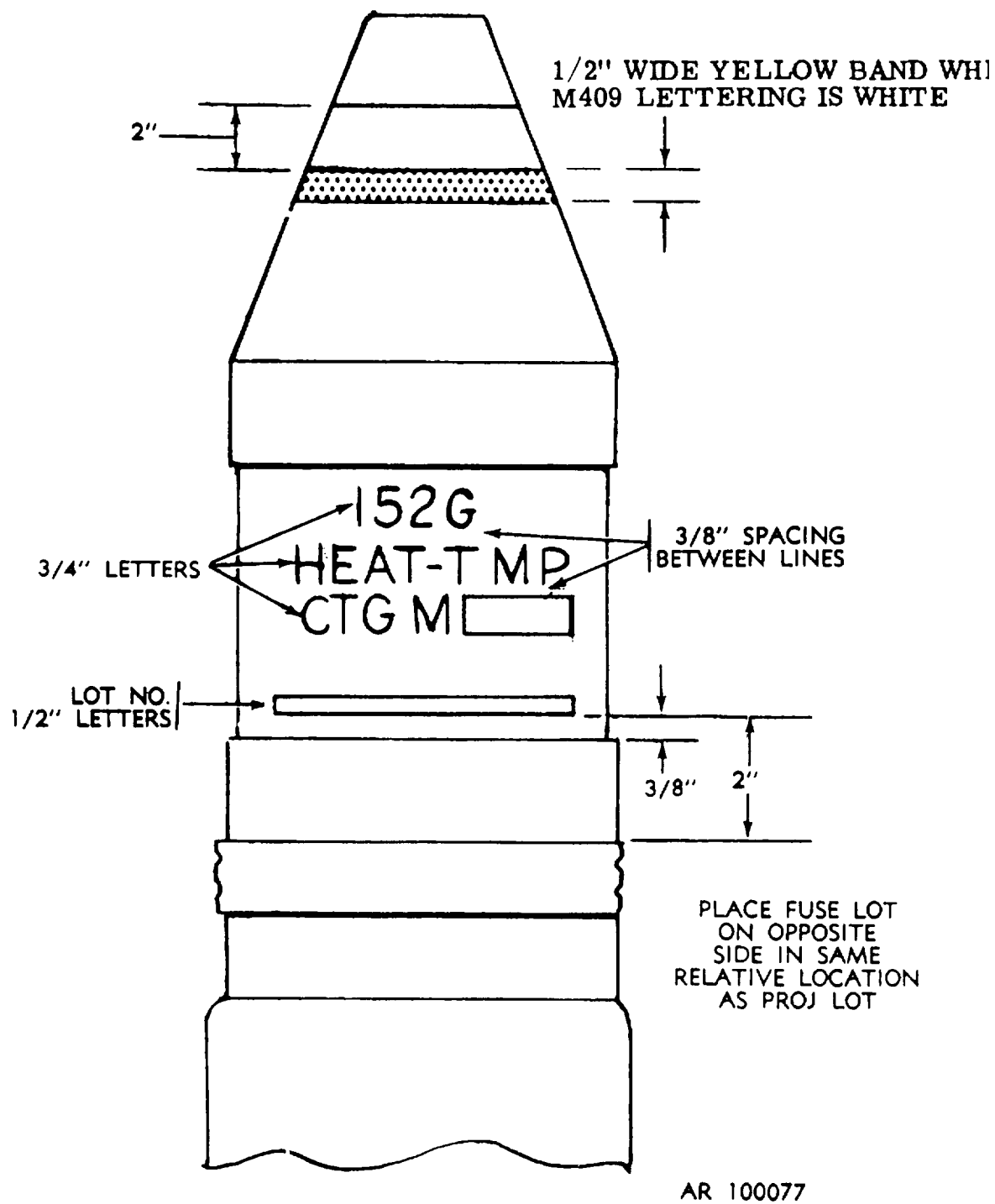
Figure E-78. Typical marking for 152mm gun cartridges M409 series and M411 series.
