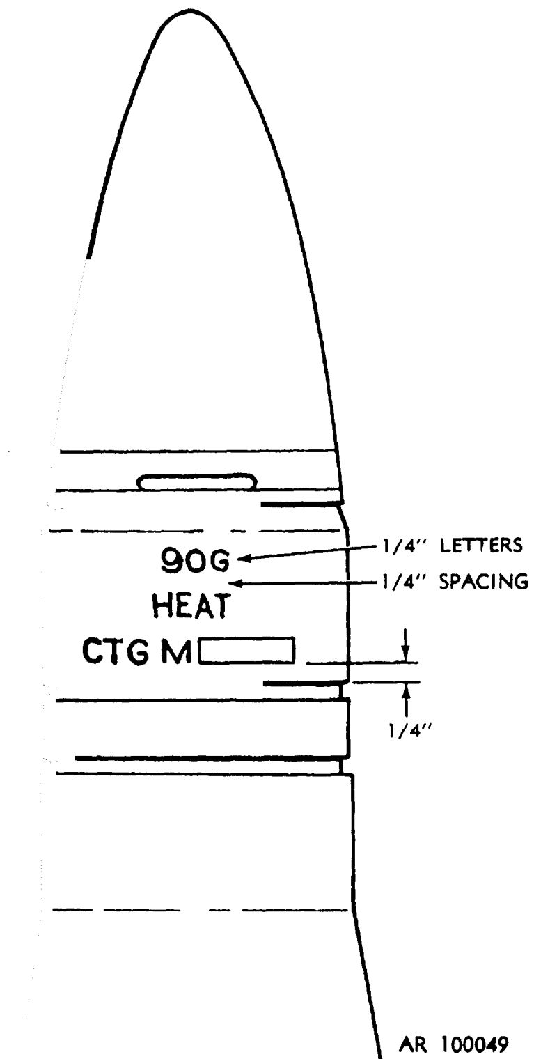
Figure E-37. Typical marking for 90mm gun cartridge M348A1.
