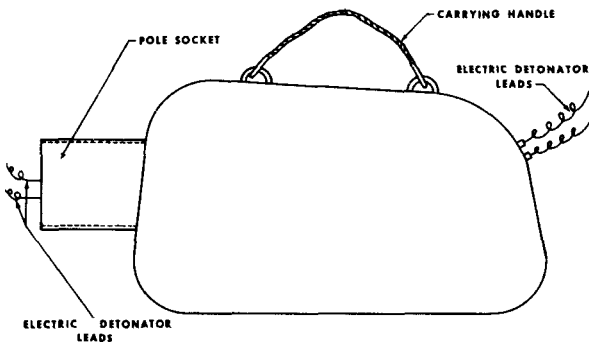
Figure 11. Concrete mound mine.
