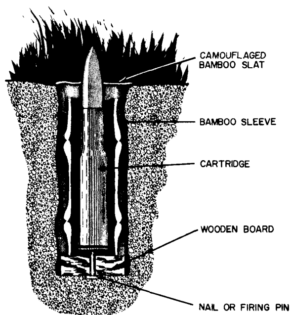
Figure 59. Cartridge trap.
