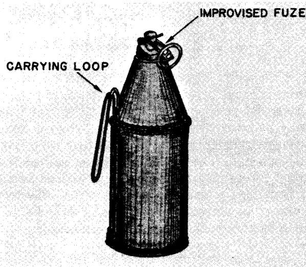
Figure 9. Tin can antipersonnel mine.
