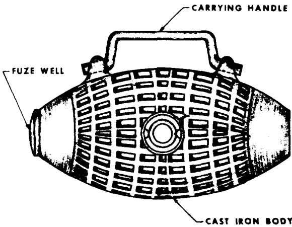
Figure 12. Cast iron fragmentation antitank mine.
