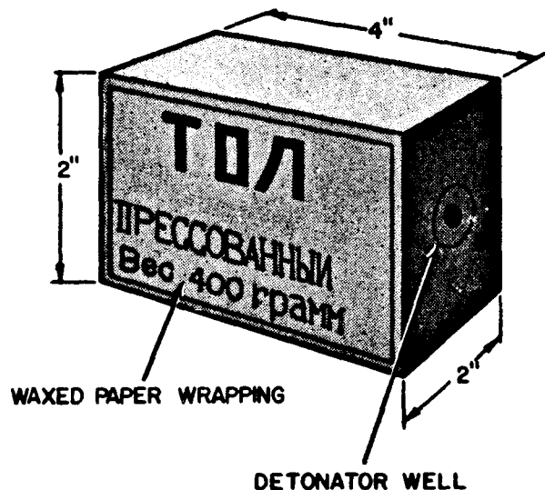
Figure 29. Soviet TNT demolition block.
