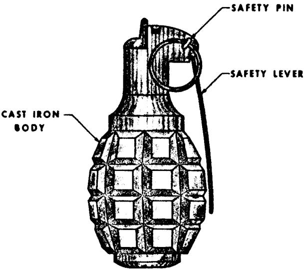
Figure 44. Defensive hand grenade.
