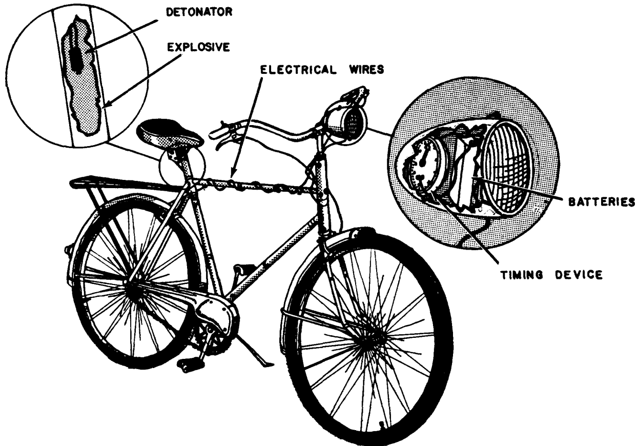
Figure 60. Bicycle mine.
