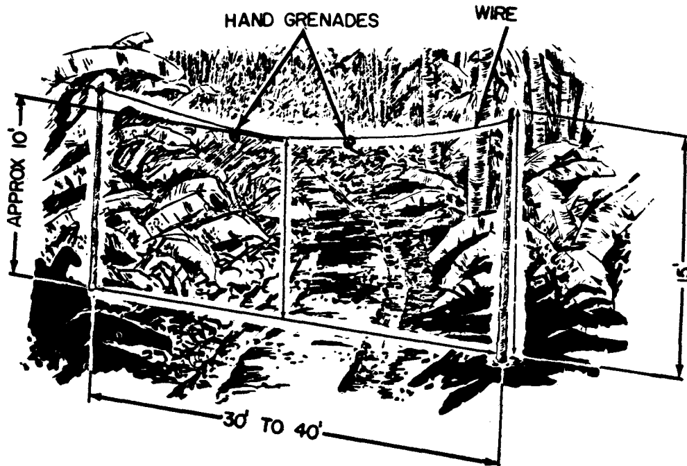
Figure 56. Tank boobytrap.
