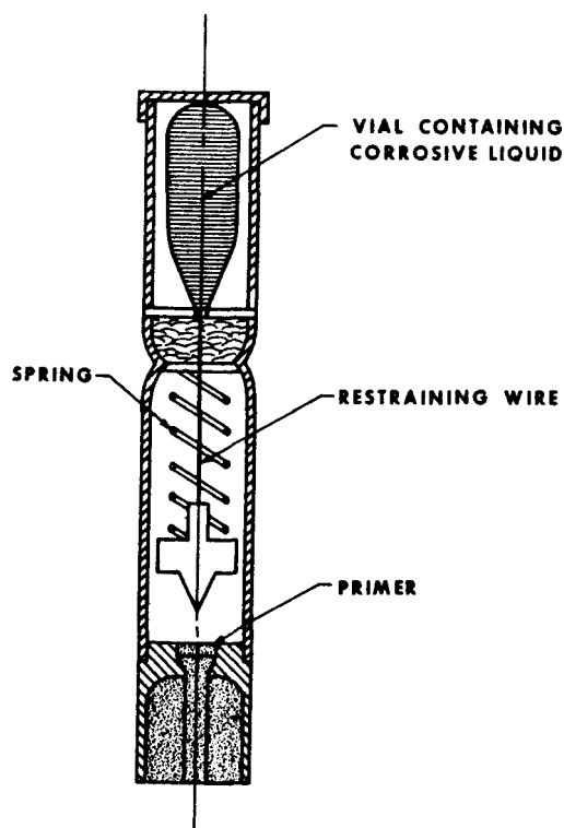
Figure 34. Chemical fuze.
