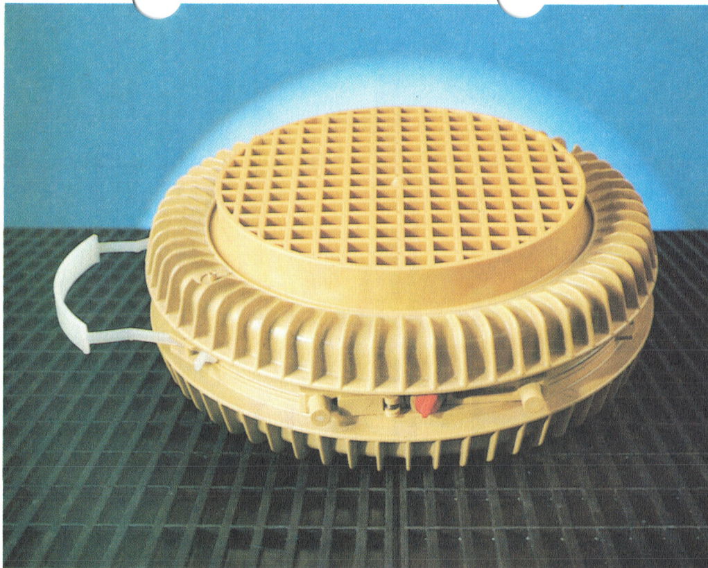
MATS/2 SCATTERABLE ANTITANK MINE
