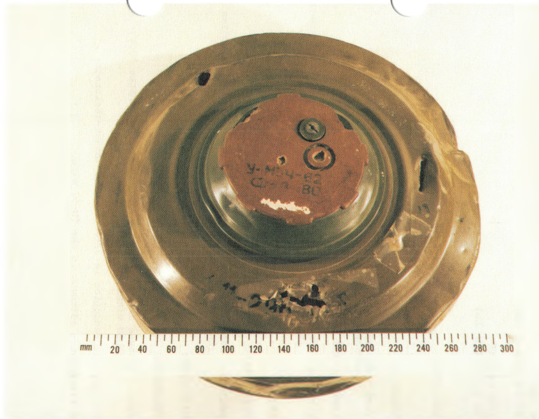
TM-62M ANTITANK MINE
