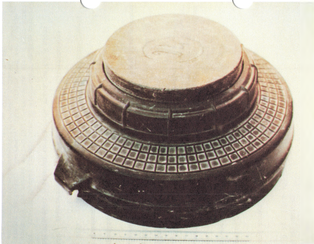
SH-55 ANTITANK MINE
