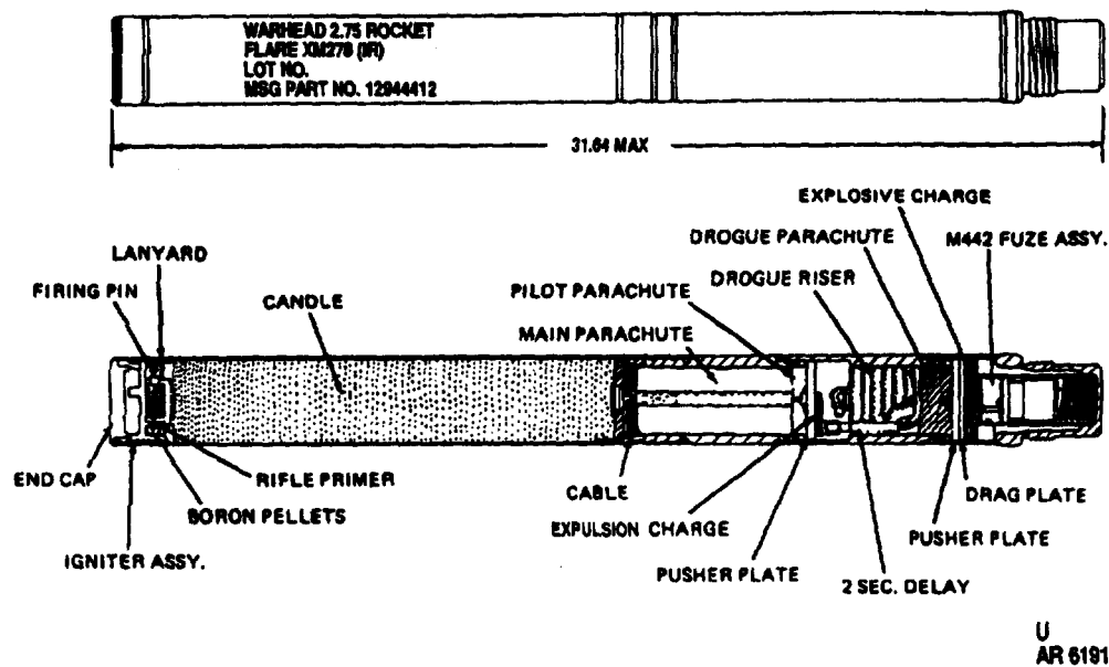
Figure 1. Rocket, flare, 2.75-inch, w/XM278 illuminating warhead.
