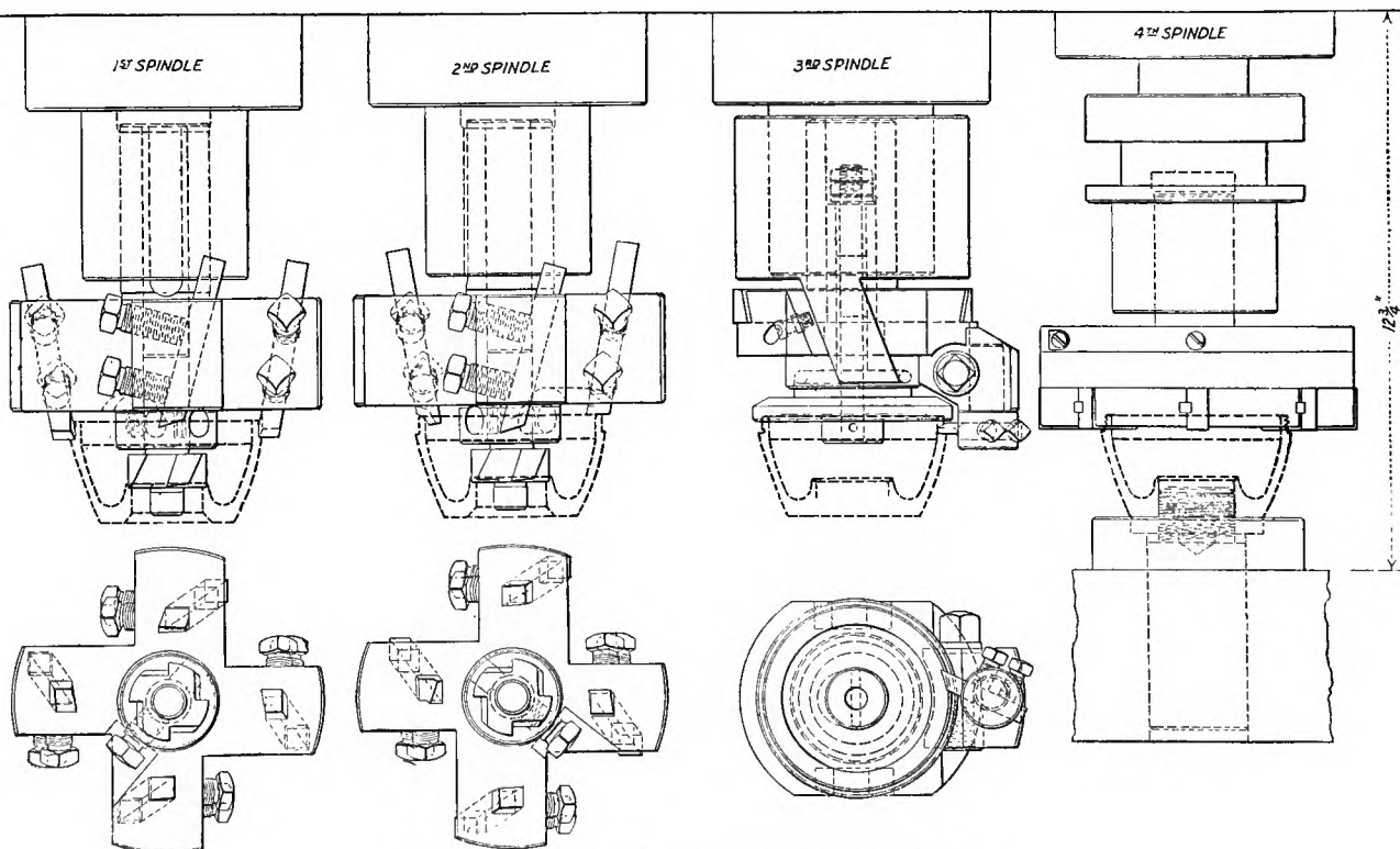
FIG. 8. SECOND SETTING FOR SHRAPNEL HEAD
