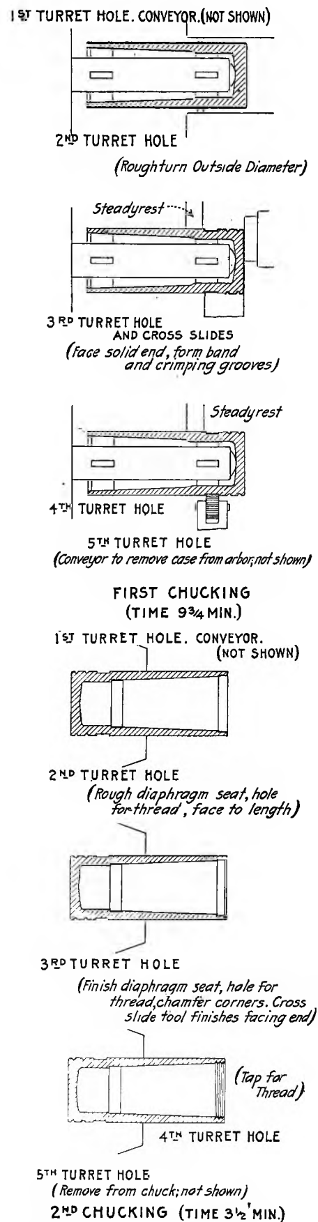
FIG. 6 - MACHINING A 3-IN. FORGED SHRAPNEL CASE
