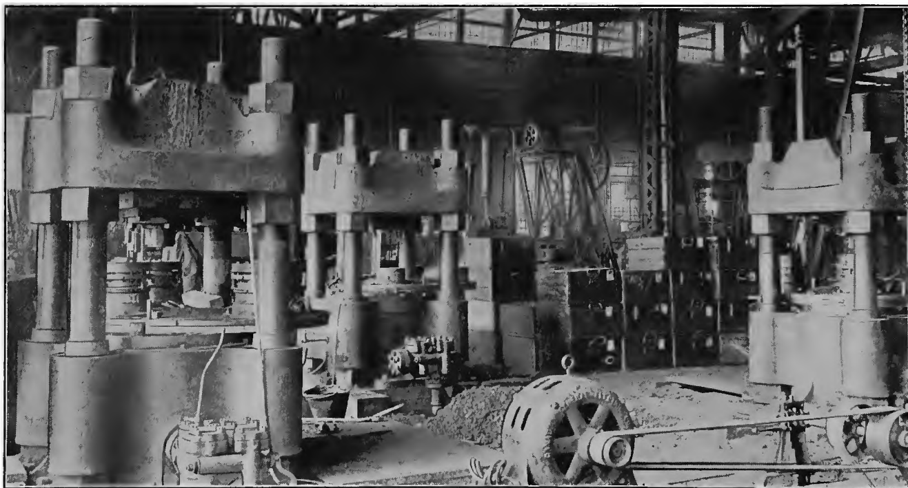
FIG. 6. GROUP OF 800-TON HEADING PRESSES
