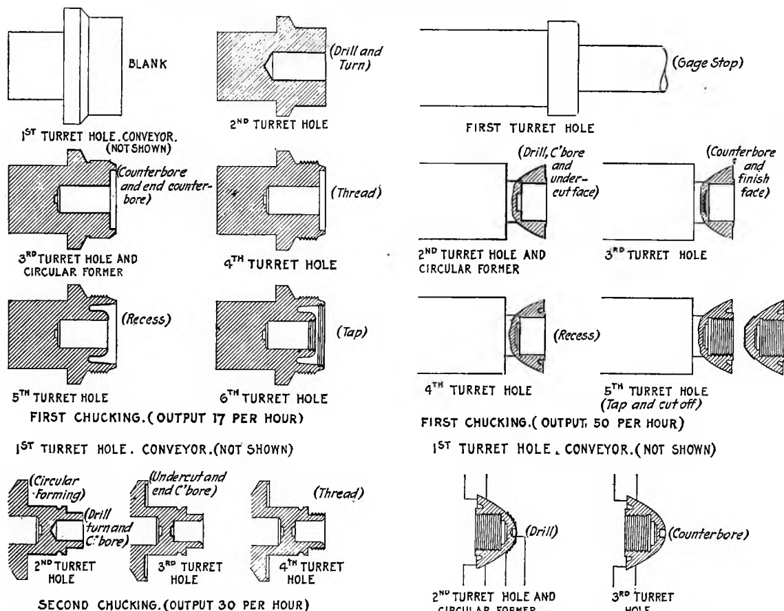
FIG. 7- MACHINING A 3.8-INCH, 30 POUND SHRAPNEL HEAD. (MATERIAL, 20 CARBON, C.R. STEEL. TOTAL TIME 12 MINUTES)
