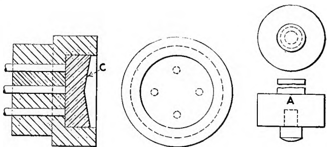
FIG. 1. STEPS IN THE PROCESS OF MAKING A TIN POWDER CUP
