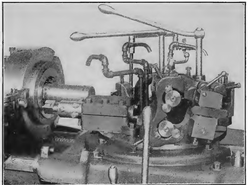
FIG. 9. CUTTING THE WAVE
