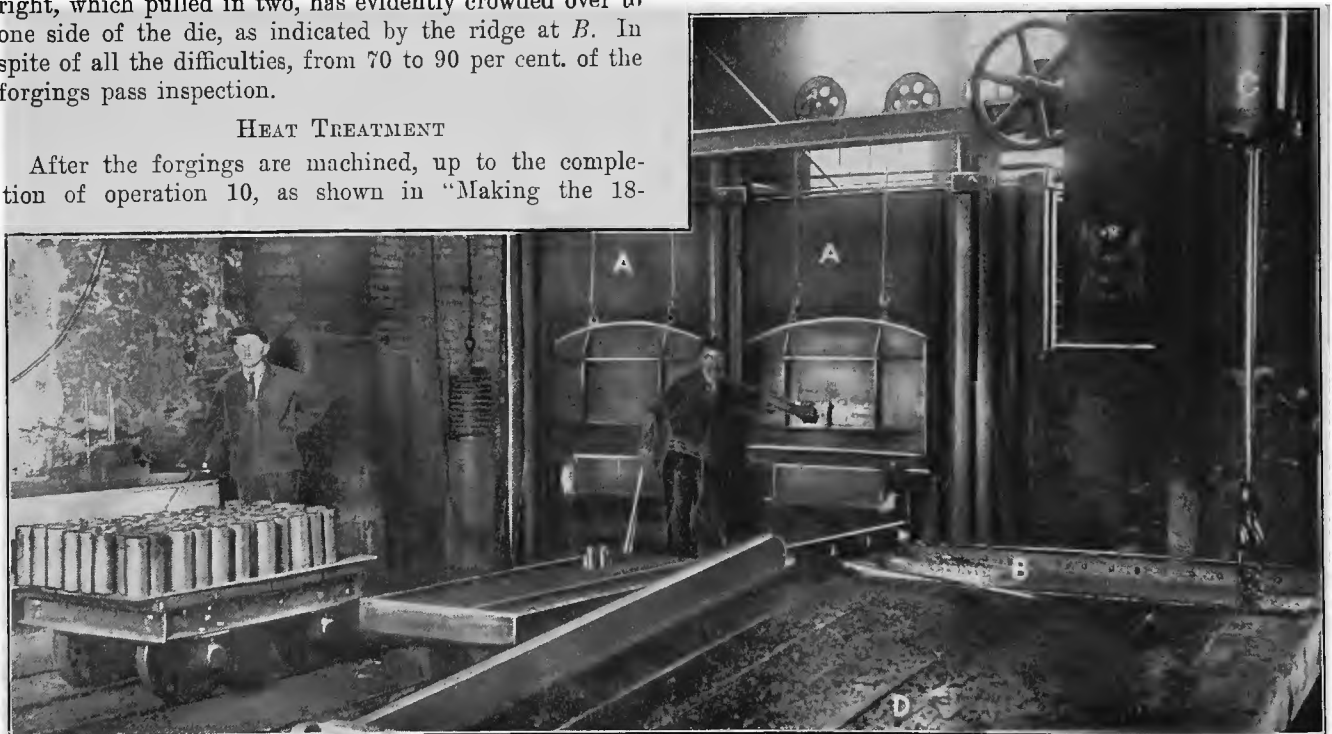
FIG. 21. HEAT-TREATING DEPARTMENT
