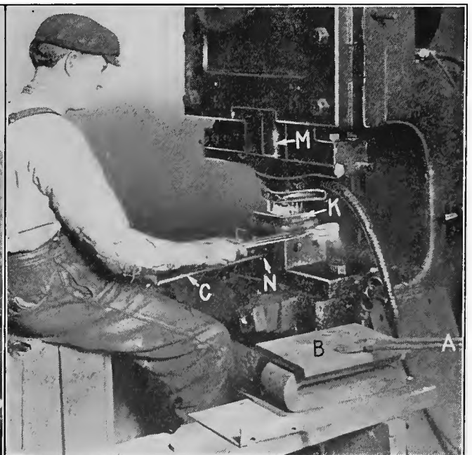
FIG. 4. COINING OPERATION
