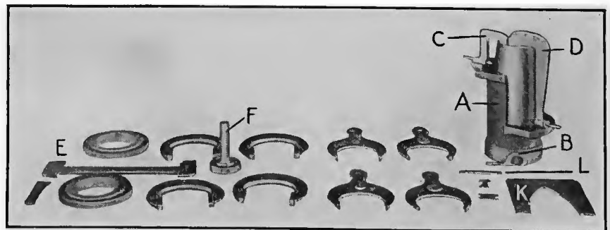
FIG. 17. GAGES USED IN THE SECOND INSPECTION
