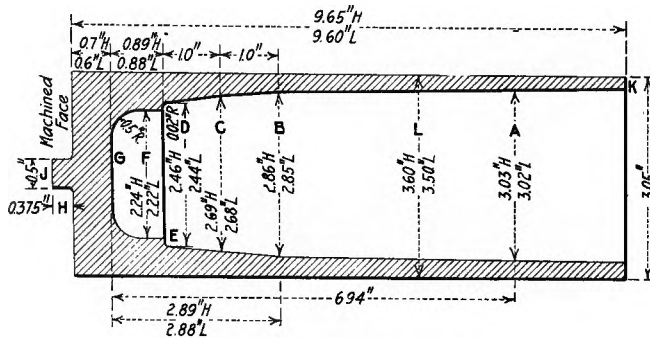
FIG. 9. SHELL SHRAPNEL
