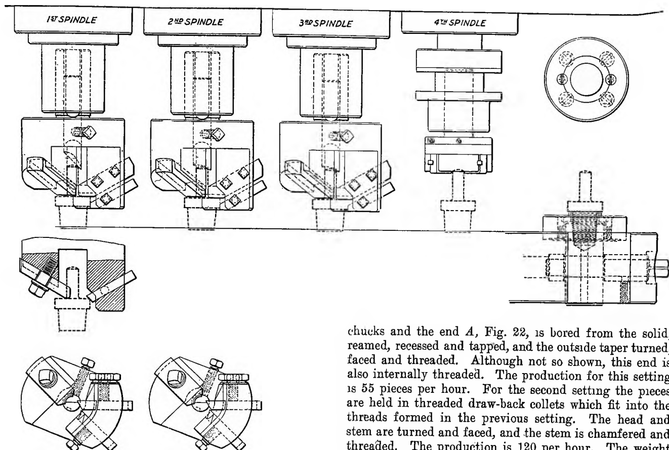
FIG. 24. SECOND SETTING ON TIME-FUSE BODIES
