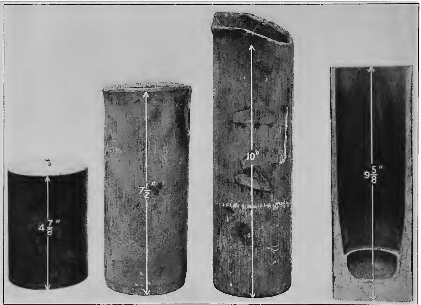
FIG. 1. THE STAGES OF EVOLUTION FROM THE BAR-STOCK BLANK TO THE FORGING TRIMMED TO LENGTH
