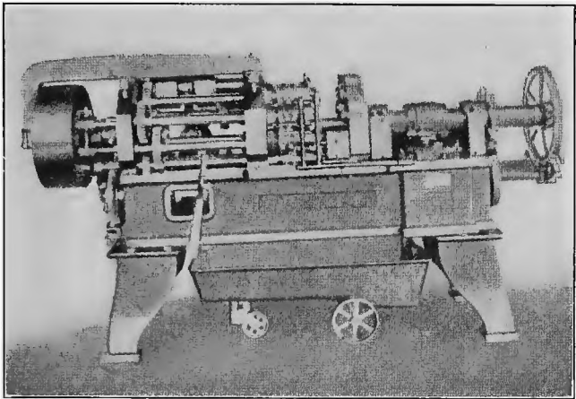
FIG. 1. SEVEN-SPINDLE AUTOMATIC
