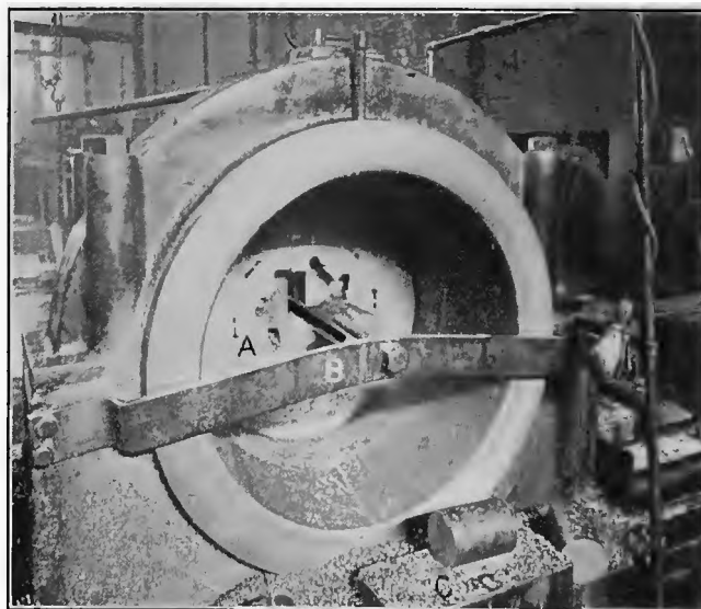
FIG. 4. GORTON COLD-SAW
