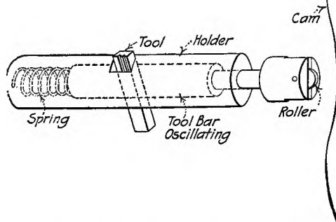
FIG. 7. THE WAVING TOOL AND HOLDER
