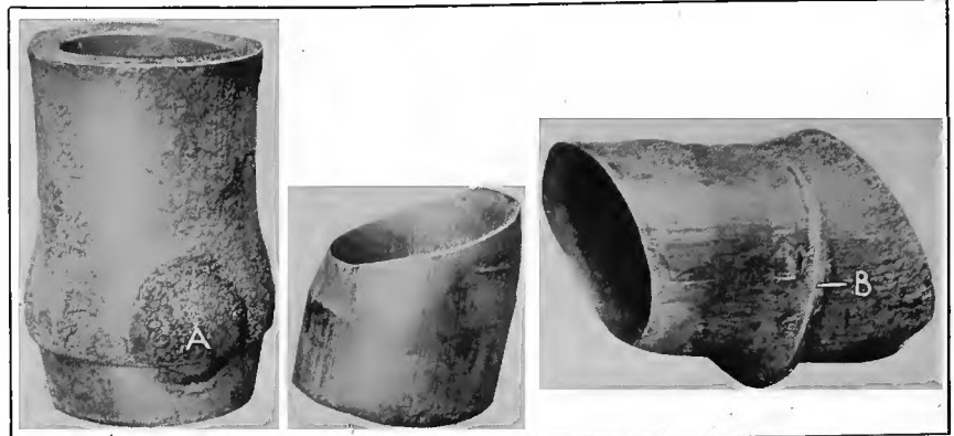
FIG. 19. EXAMPLES OF SPOILED FORGINGS
