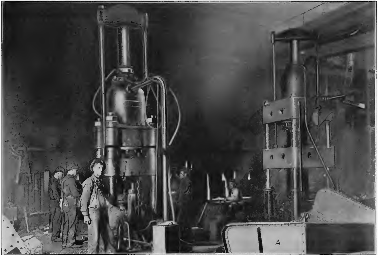
FIG. 13. R. D. WOOD & CO. PRESS TO LEFT AND NILES PRESS TO RIGHT
