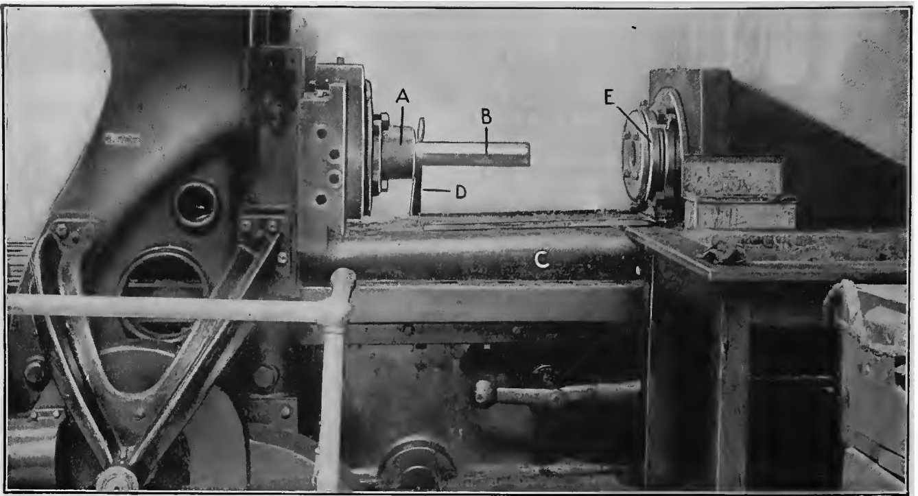
FIG. 10. FROG PLANER USED FOR THE LAST DRAW
