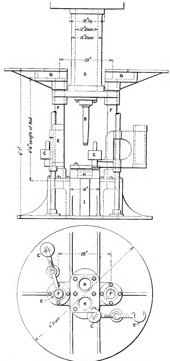
FIG. 11. EQUIPMENT SHOWN FOR SECOND OR DRAWING OPERATION
