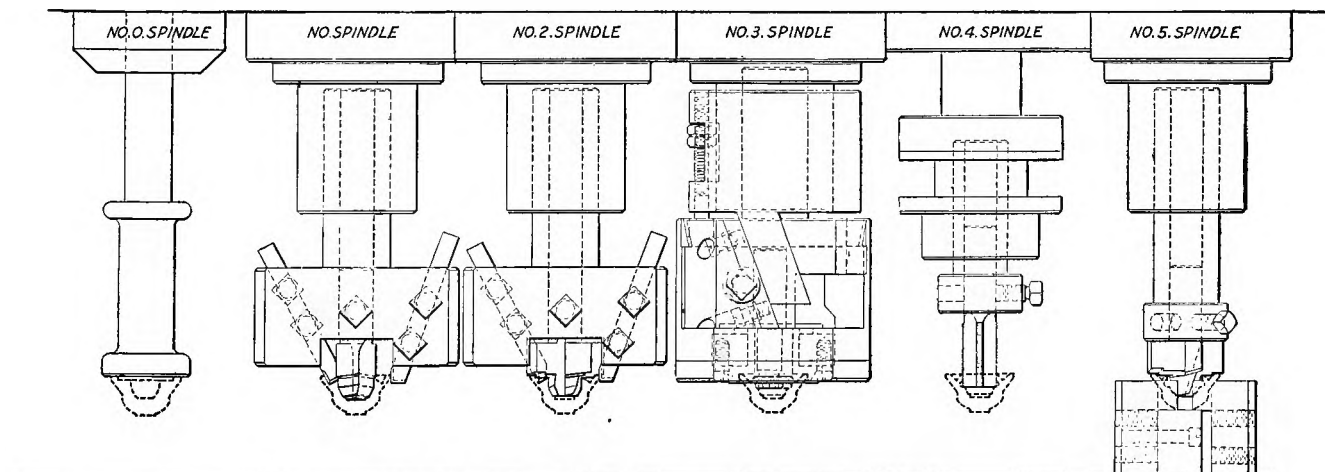
FIG. 18. TOOLING FOR MACHINING TIME-FUSE NOSES
