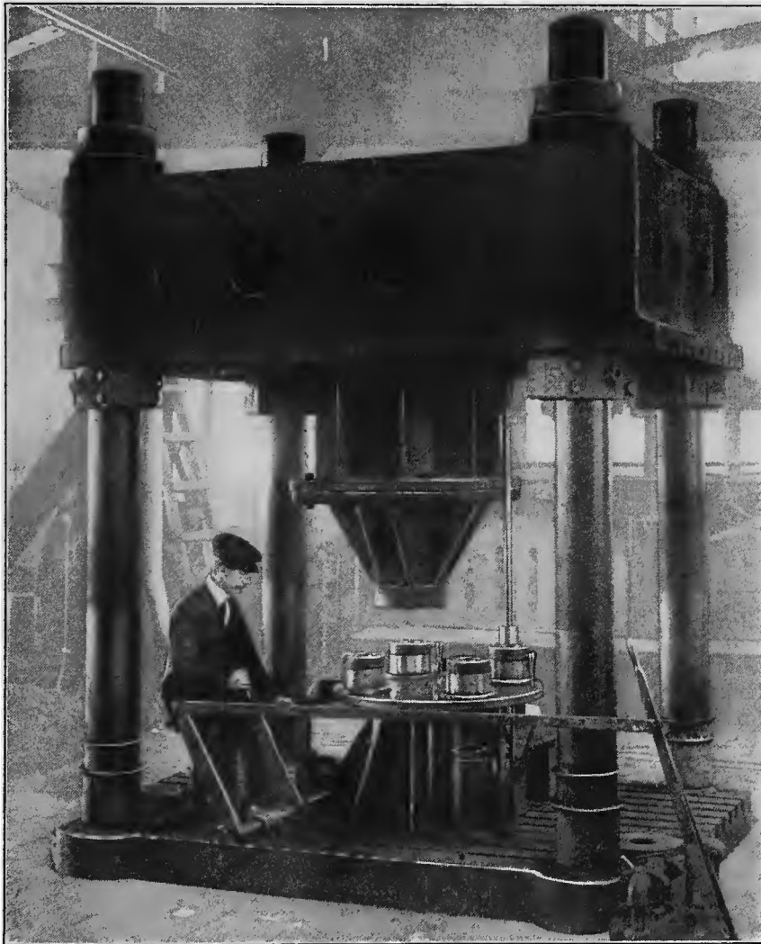
FIG. 1. A STATION-TYPE INDENTING PRESS BUILT AT ANGUS
