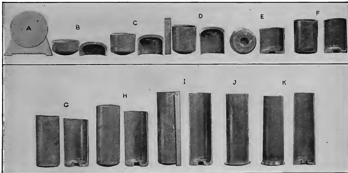
FIG. 1. THE EVOLUTION OF A CARTRIDGE CASE
