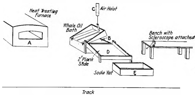
FIG. 20. HEAT-TREATING ARRANGEMENT
