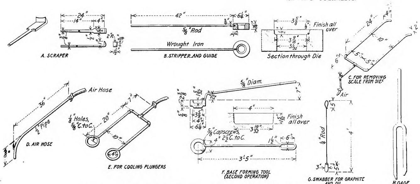
FIG. 12. ACCESSORIES IN CONNECTION WITH HYDRAULIC FORGING PRESS
