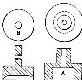
FIG. 3. PUNCH USED IN DRAWING POWDER-CUP BOTTOM
