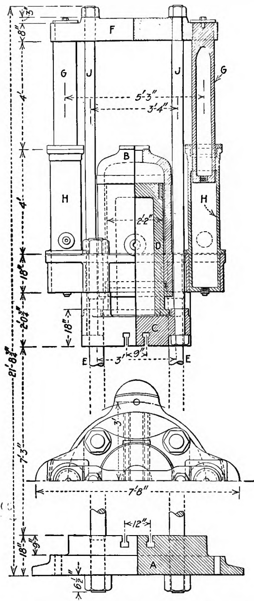
FIG. 3. ASSEMBLED CROSS-SECTIONAL VIEW OF 26x45-IN. SHELL-FORGING PRESS
