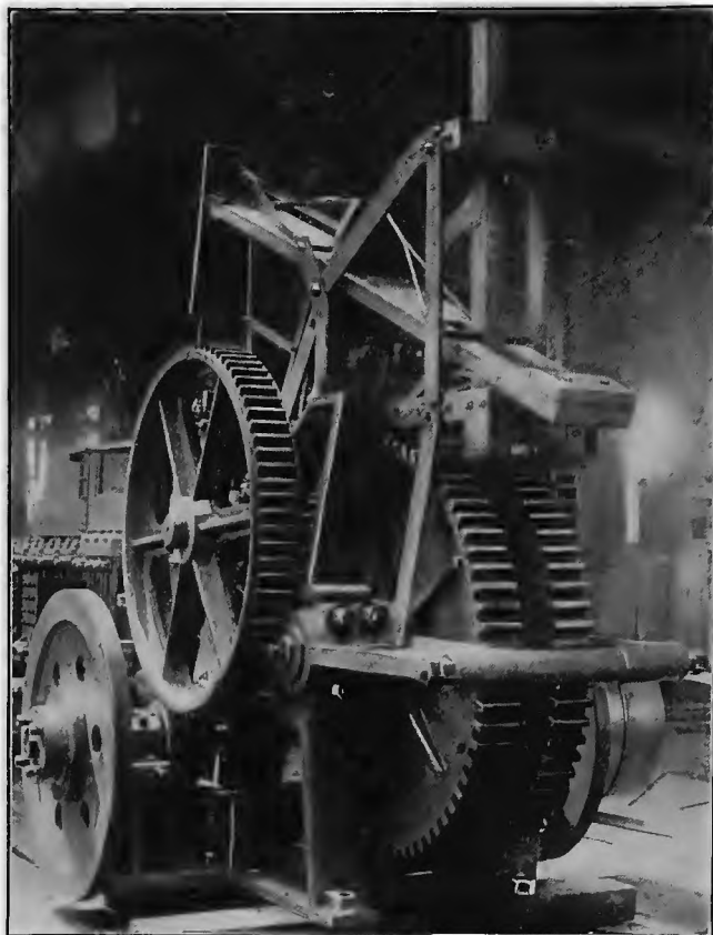
FIG. 4. REAR VIEW OF THE HAY-BALING PRESS
