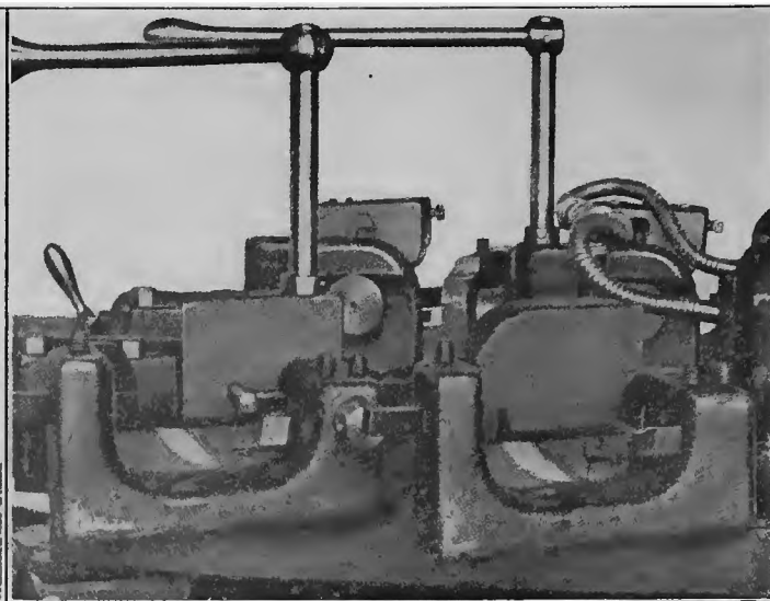
FIG. 6. TOOLS FOR UNDERCUTTING THE RECESS
