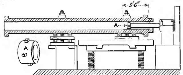
FIG. 9. BORING ACCUMULATOR CYLINDER ON BERTRAM HORIZONTAL MACHINE
