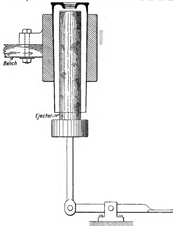
FIG. 10. SPECIAL BENCH VISE FOR HOLDING CARTRIDGE CASES
