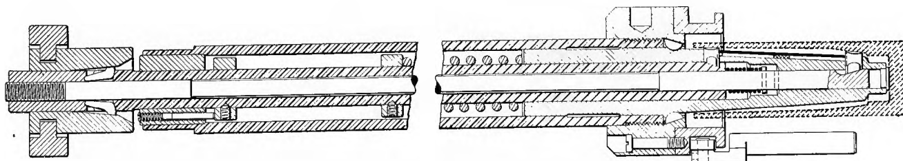
FIG. 3. DETAILS OF THE CENTERING MANDREL
