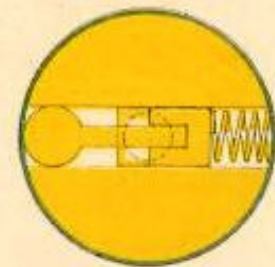
SECTIONAL PLAN OF SHUTTER, CLOSED.
