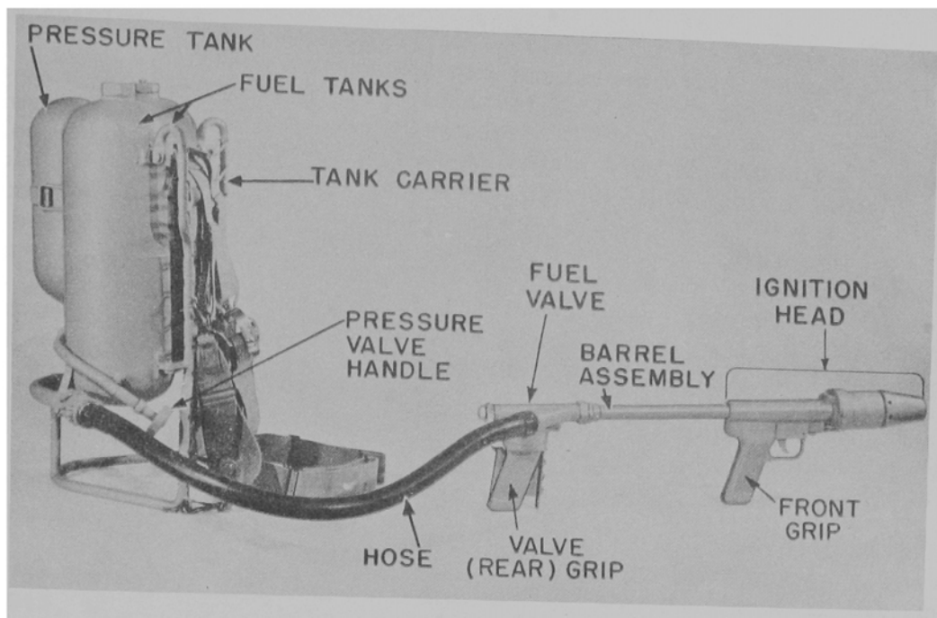
Figure 4. The M2-2 Portable Flame Thrower.
