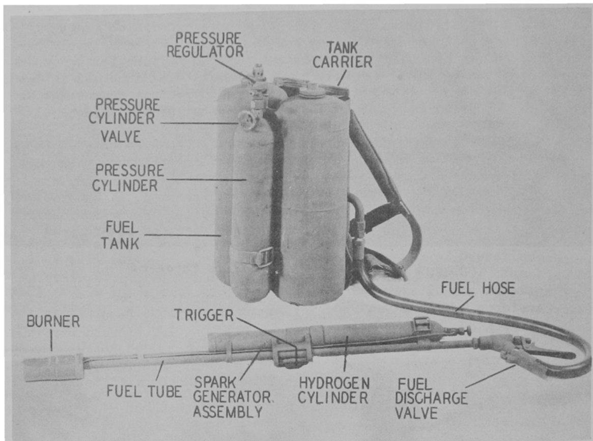
Figure 3. The M1A1 Portable Flame Thrower.
