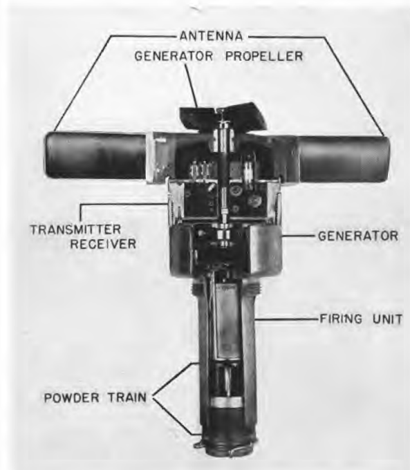
FIGURE 3. Cutaway of bar-type, radio, bomb fuze (T-51).
