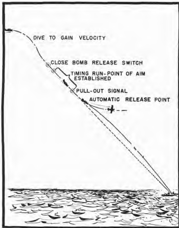
FIGURE 7. Diagram of typical toss-bombing maneuver.
