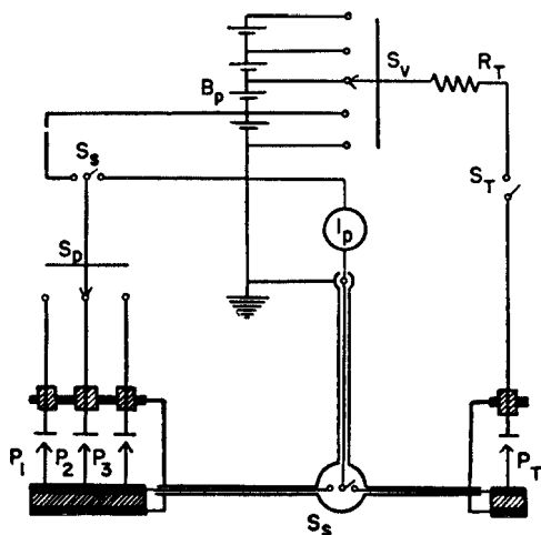
PHOTOCELL CIRCUIT
