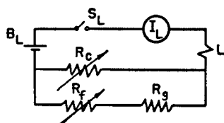
LAMP CIRCUIT
