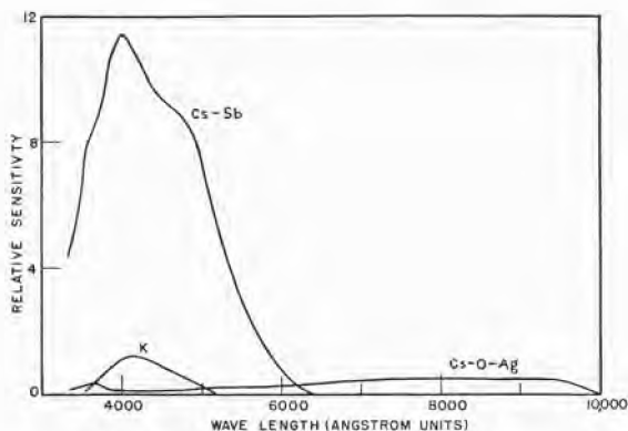
FIGURE 20. Spectral response curves of three typical photosensitive surfaces.
