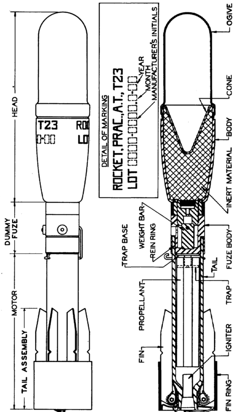
FIGURE 23. - ROCKET, PRACTICE, 2.36", T23
