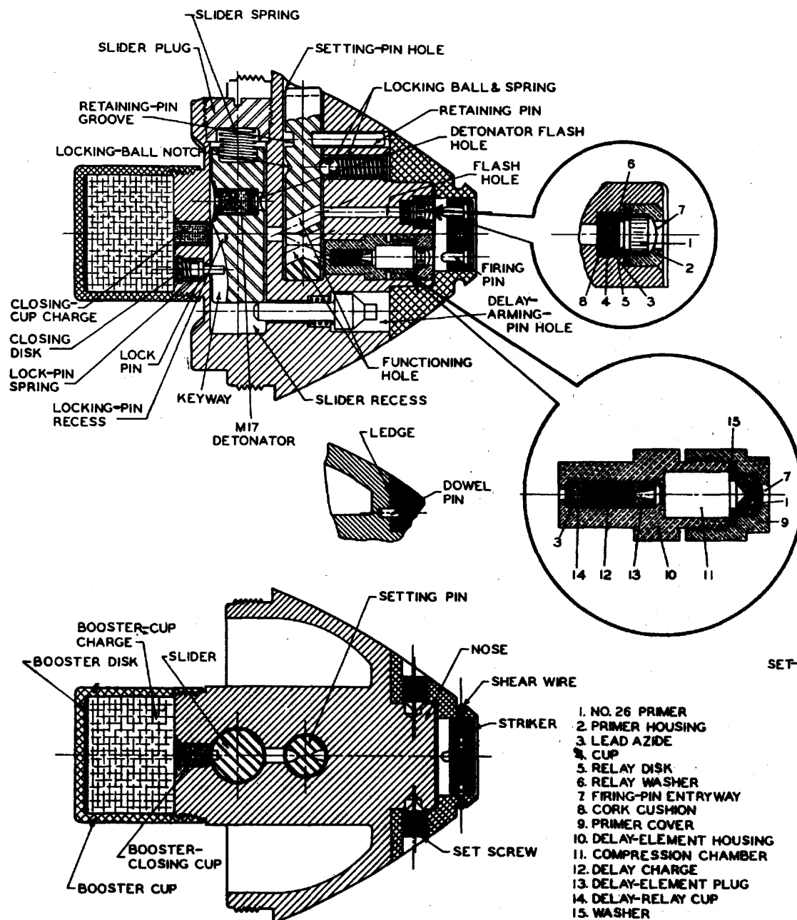
FIGURE 37. - FUZE, POINT DETONATING, M4
