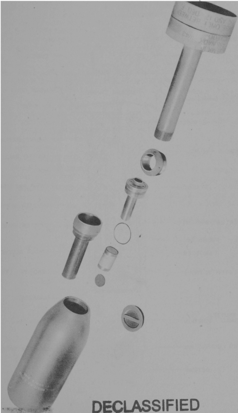
FIGURE 75. - ROCKET, H.E., 7.2" DISASSEMBLED
