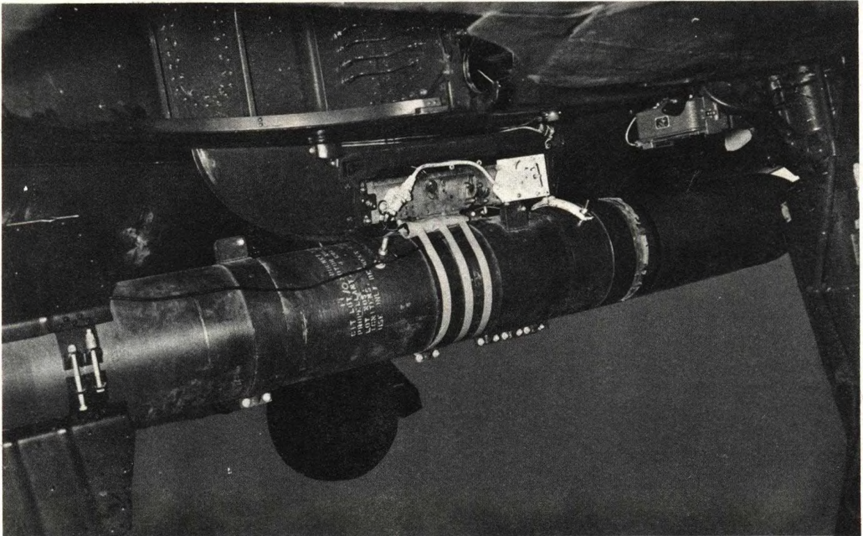
Figure 26—11.75-inch Aircraft Rocket Secured to Bomb Rack on F6F-5 Aircraft (Note that electrical connector does not pass over sway brace. An obsolete type of firing line is shown in this photograph. Also note lanyard installed, secured, and reel pointer near 6-foot mark).
