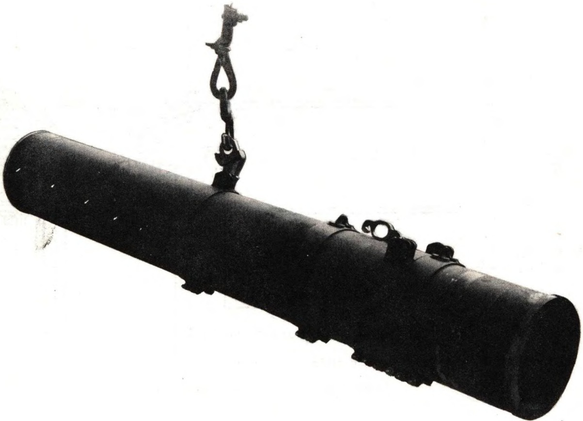
Figure 10—Hoisting Motor with Carrier Mk 17 Mod 0 Attached to Handling Band
