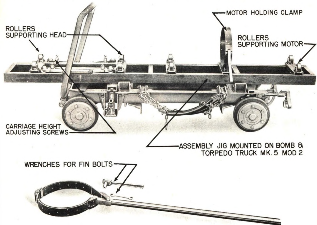
Figure 8—Assembly Equipment
