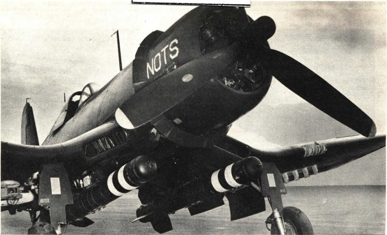
Figure 17—Two 11.75-inch Aircraft Rockets (with Dummy Heads) Loaded on F4U-1D Aircraft
