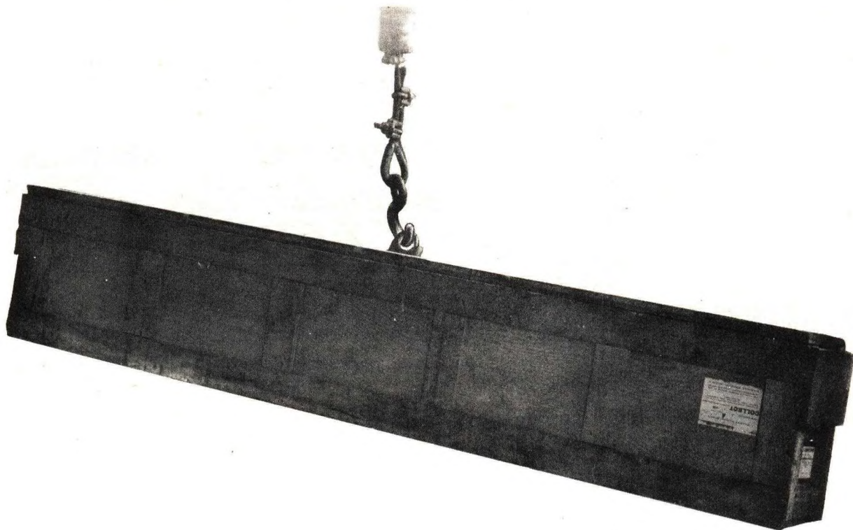
Figure 9—Hoisting Crated Motor with Carrier Mk 17 Mod 0 Attached to Handling Band
