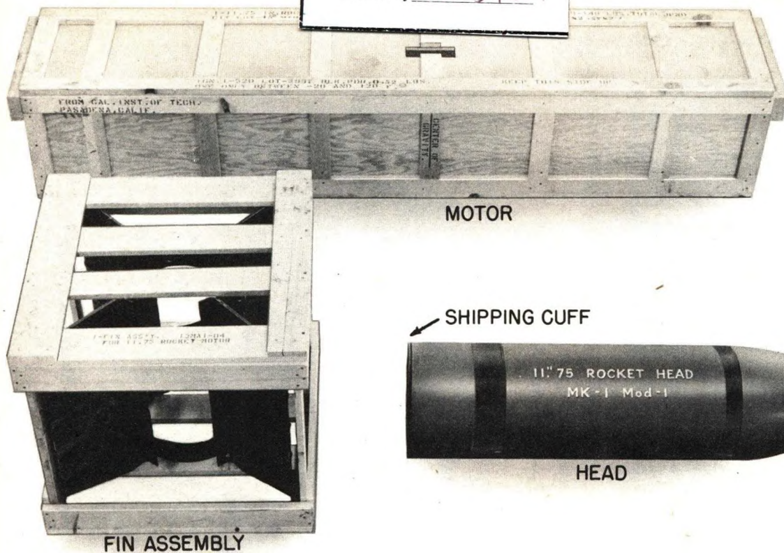
Figure 14—Rocket Components as Shipped (Note: The fin assembly is to be shipped in a steel box instead of the crate as shown.)
