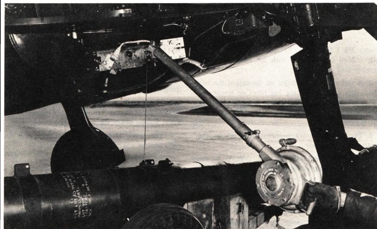
Figure 25—Hoisting Rocket onto Bomb Rack on F6F-5 Aircraft
