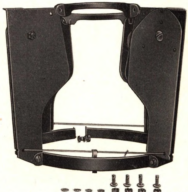
Figure 12.—Tail Assembly with Four Bolts and Nuts Removed from After Band
