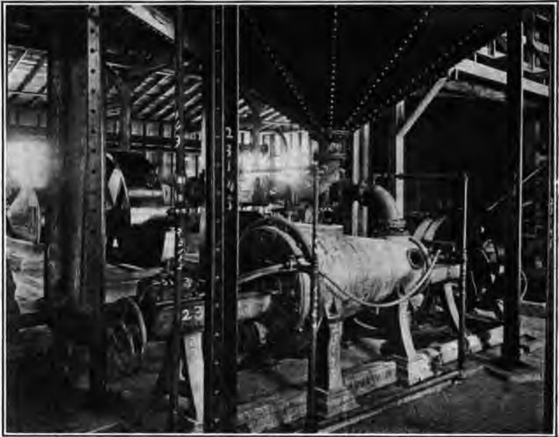
PLATE 9.—JORDAN PULFING ENGINE UNIT, OLD HICKORY SMOKELESS POWDER PLANT, NASHVILLE, TENN.
