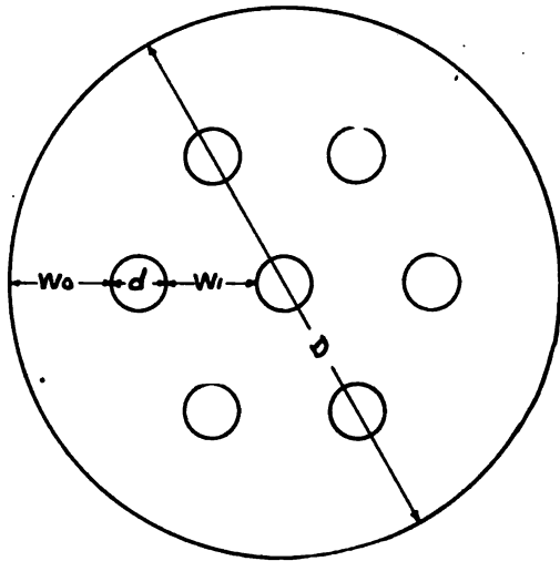
CYLINDRICAL GRAINS. 7 PERFORATIONS.
