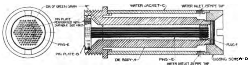
POWDER DIE ASSEMBLY USED FOR CYLINDRICAL GRAINS
