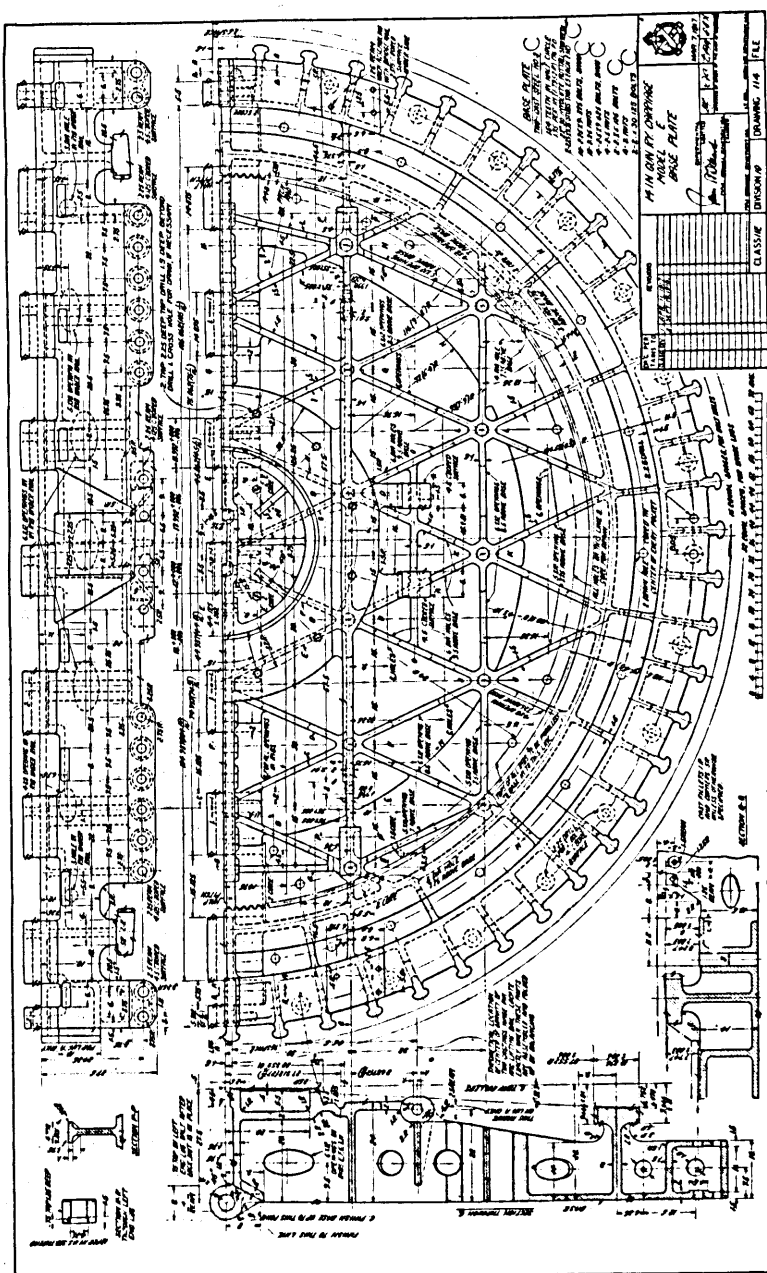
ONE-HALF SECTION OF THE 14-INCH MODEL E BASE.
