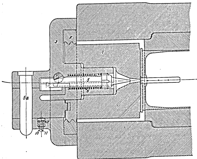
FIRING MECHANISM OF THE 3-INCH GUN, MODEL OF 1898.
