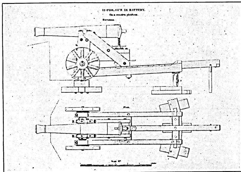
SEACOAST CARRIAGE OF THE LATE EIGHTEENTH CENTURY.
