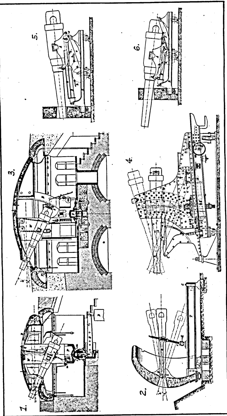
PLATE OF EARLY SEACOAST AND DISAPPEARING CARRIAGES.
