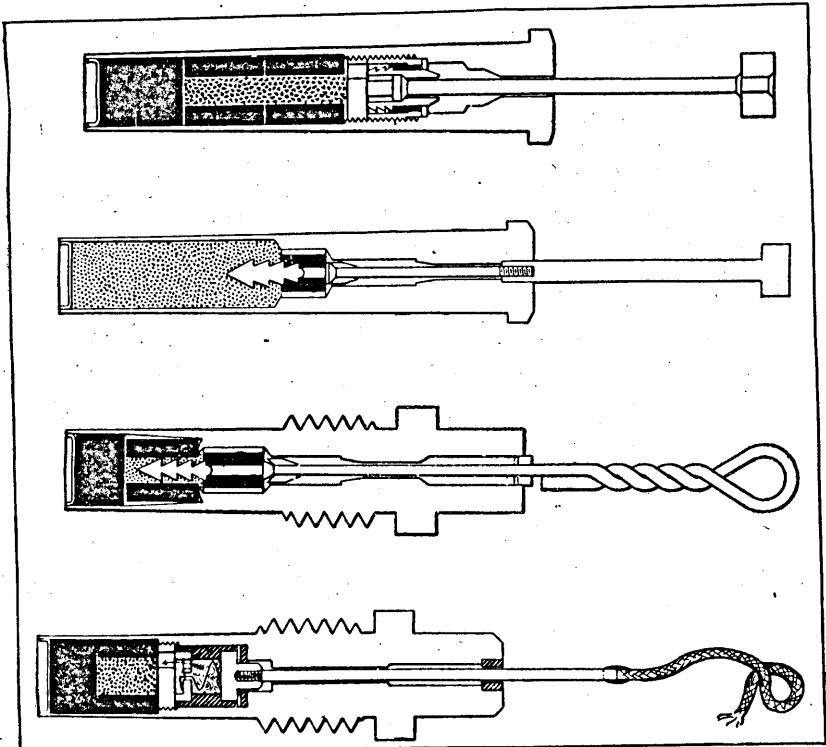
FRICTION AND ELECTRICAL PRIMER TYPES.
