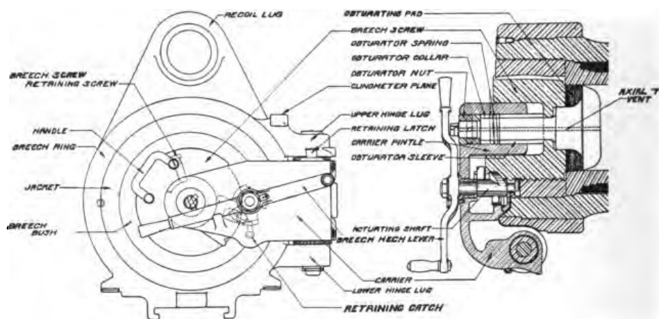
BREECH MECHANISM (MARK II).
