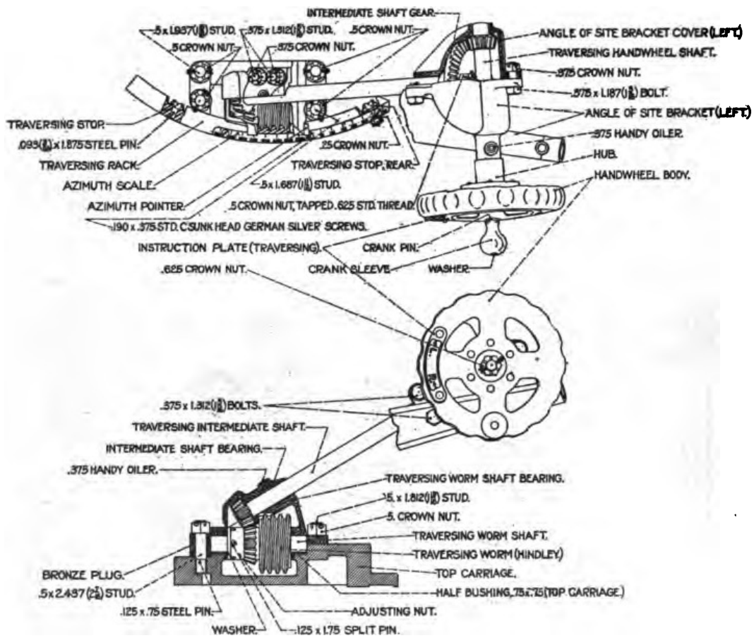
75 M M. GUN CARRIAGE, MODEL OF 1916. TRAVERSING MECHANISM.
