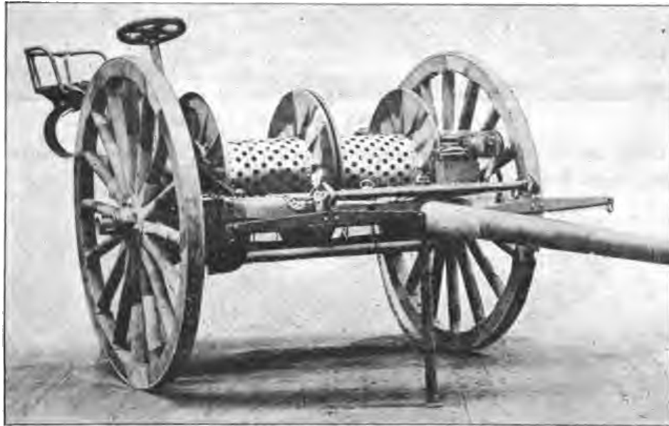
FRONT VIEW OF REEL.
