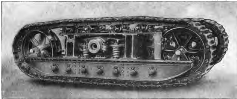
SIDE ELEVATION OF TRACK LAYER.
