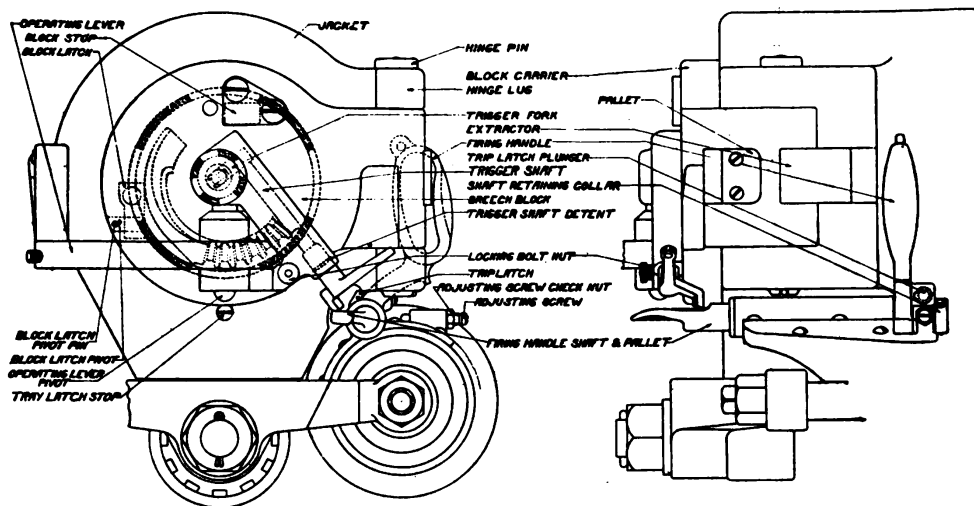
BREECH MECHANISM.
