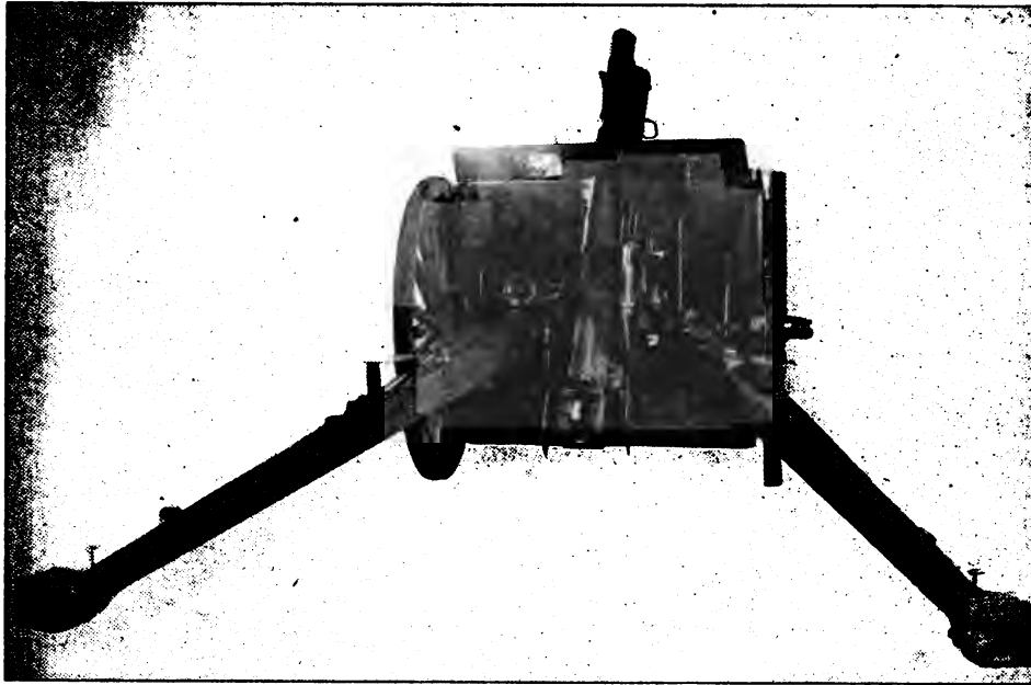
GUN AT MAXIMUM ELEVATION.
