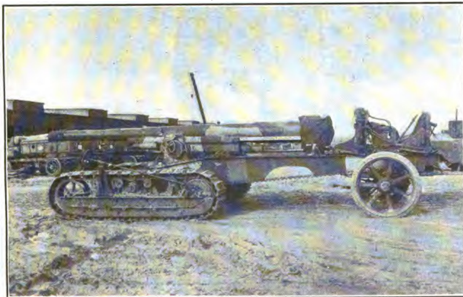
CATERPILLAR ADAPTER FOR 155-MM. GUN, G. P. F., MODEL 1918.
