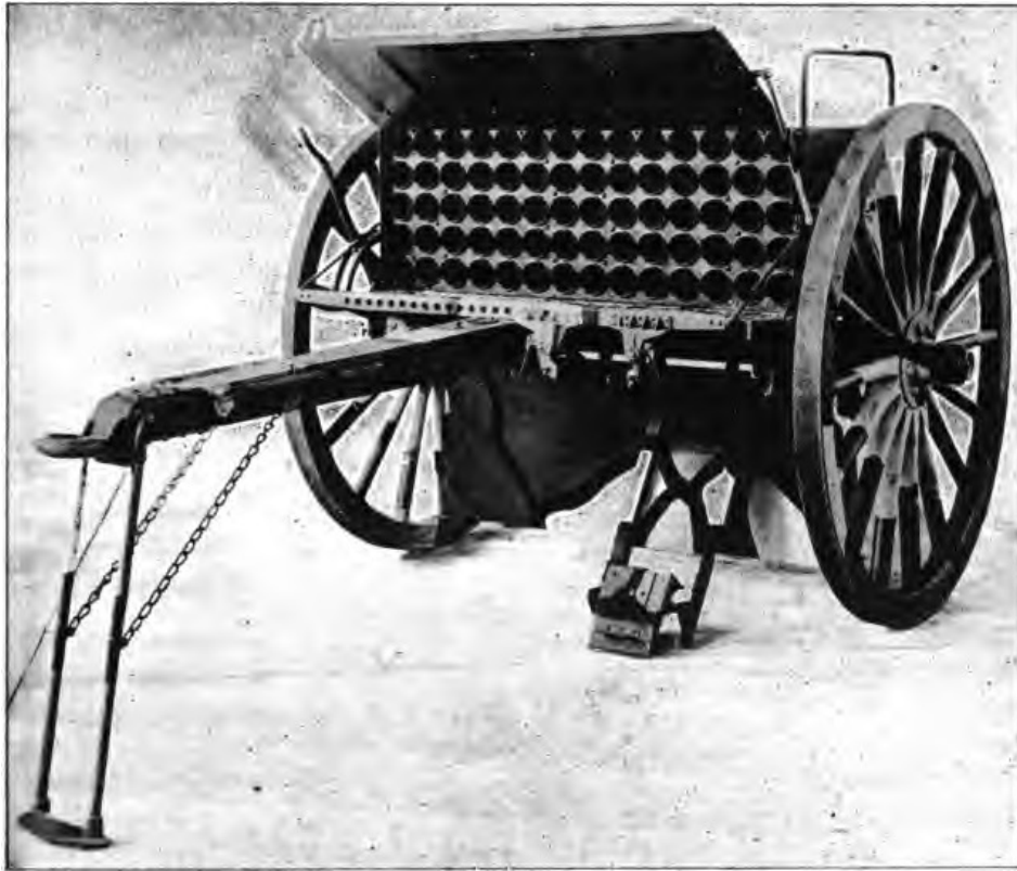
FRONT VIEW OF CAISSON.
