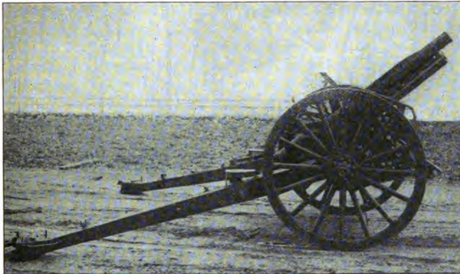
RIGHT SIDE VIEW OF CARRIAGE IN BATTERY POSITION.
