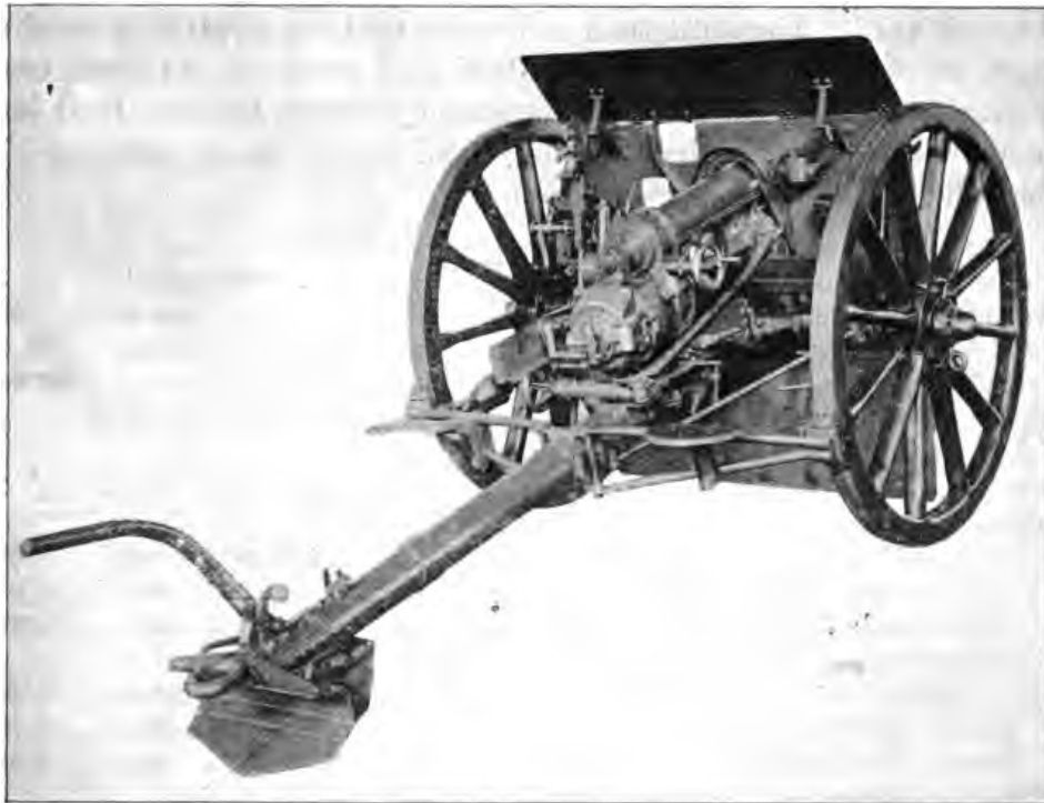
REAR VIEW OF CARRIAGE.
