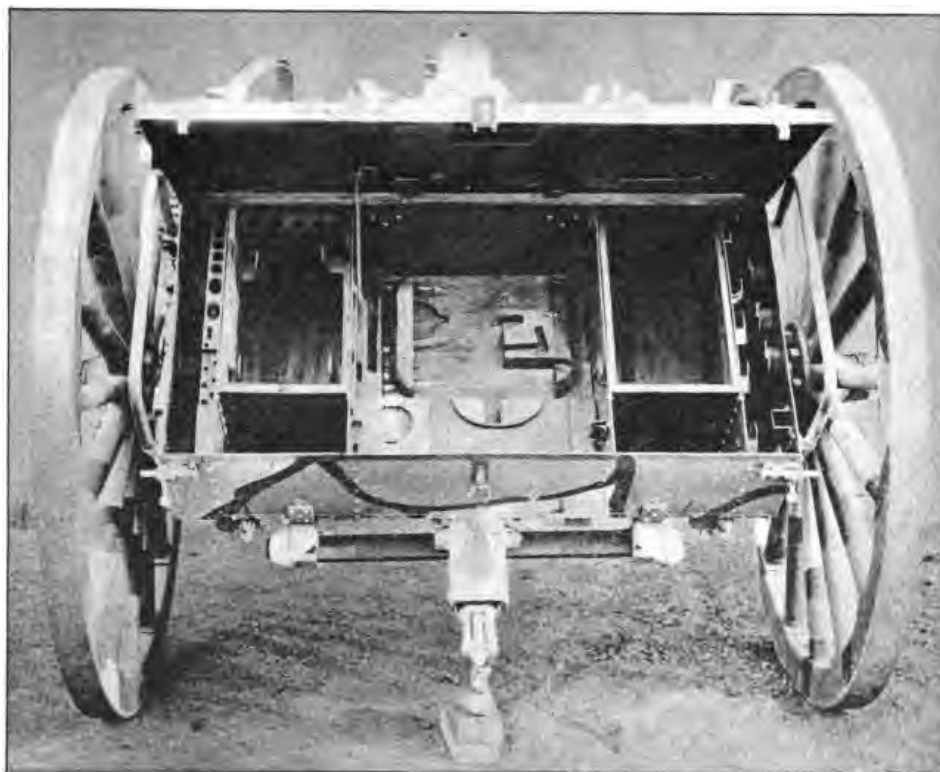
TOP VIEW SHOWING INTERIOR OF FORGE LIMBER.
