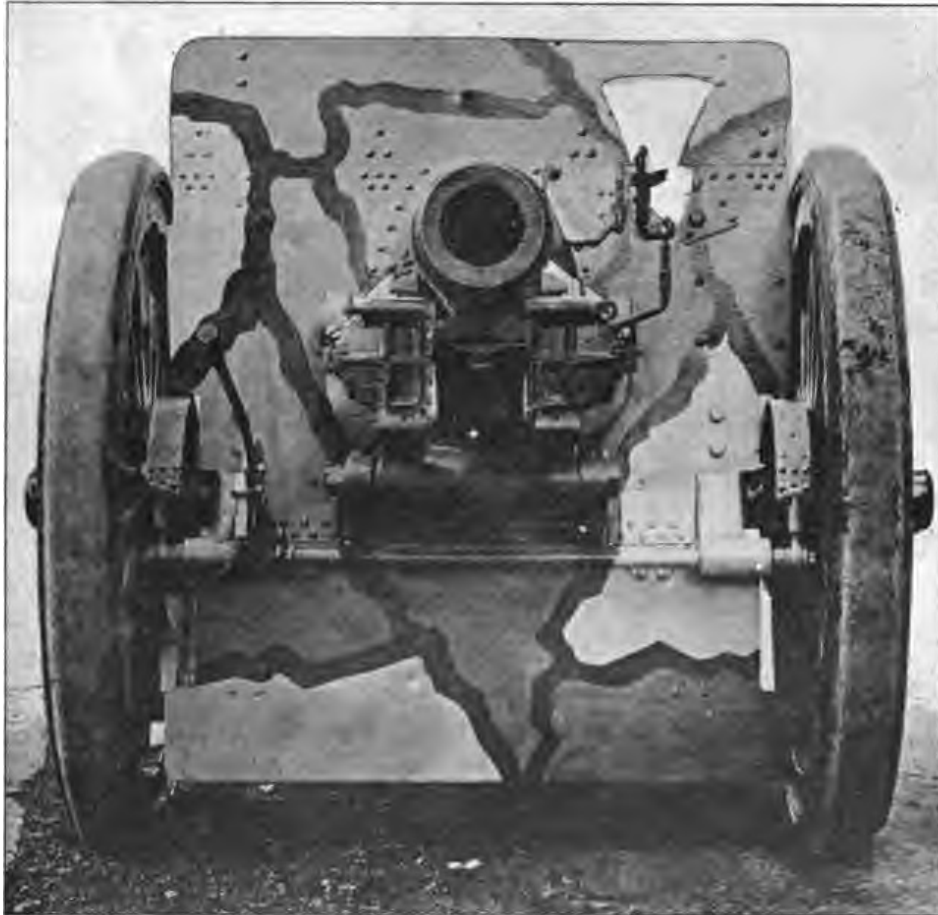
FRONT VIEW OF CARRIAGE EQUIPPED WITH BAND BRAKES.
