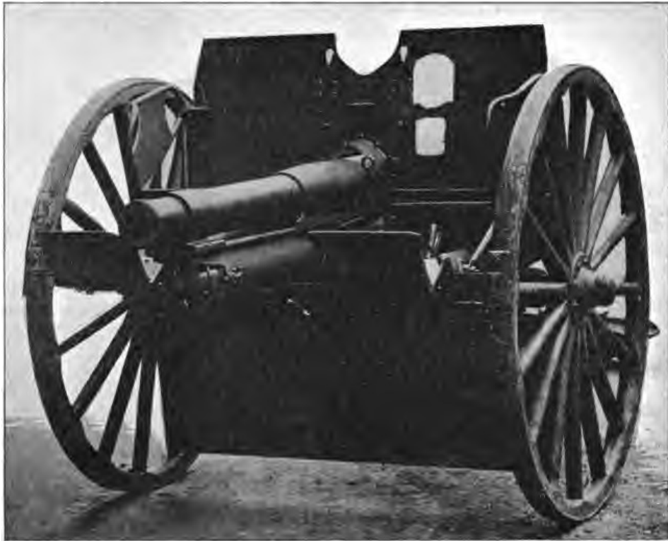
FRONT VIEW OF CARRIAGE.
