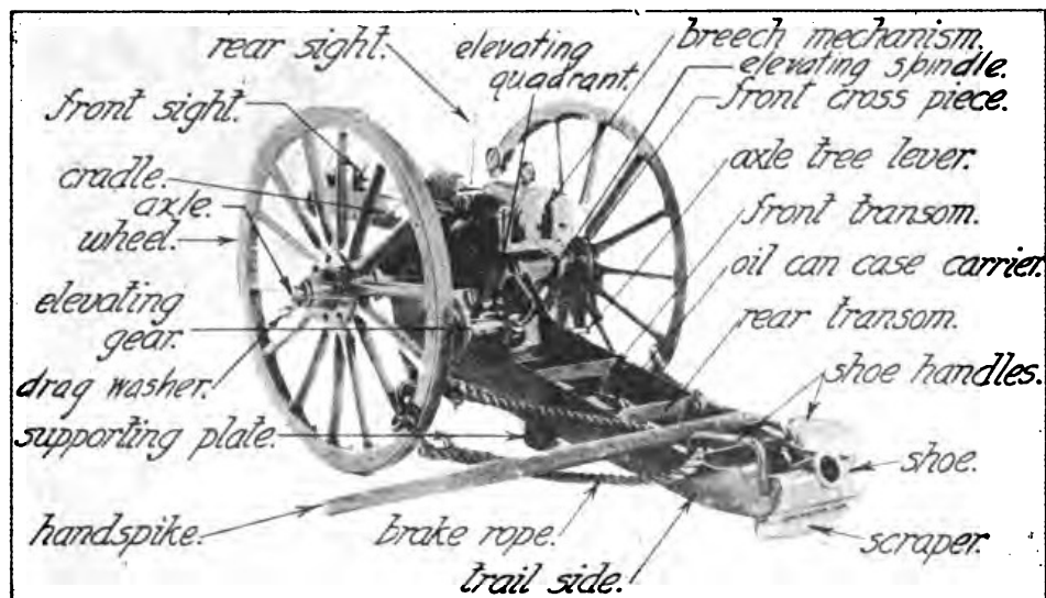
SIDE VIEW OF CARRIAGE IN BATTERY.
