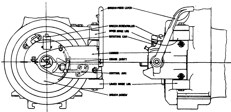
BREECH MECHANISM (MARK I).
