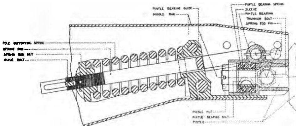
SECTIONAL DIAGRAM OF POLE SUPPORT.
