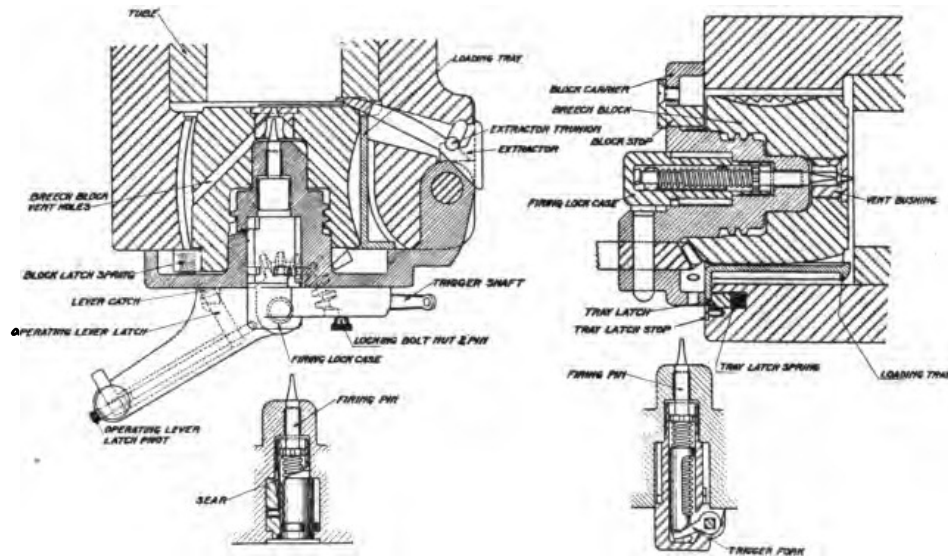
FIRING MECHANISM.
