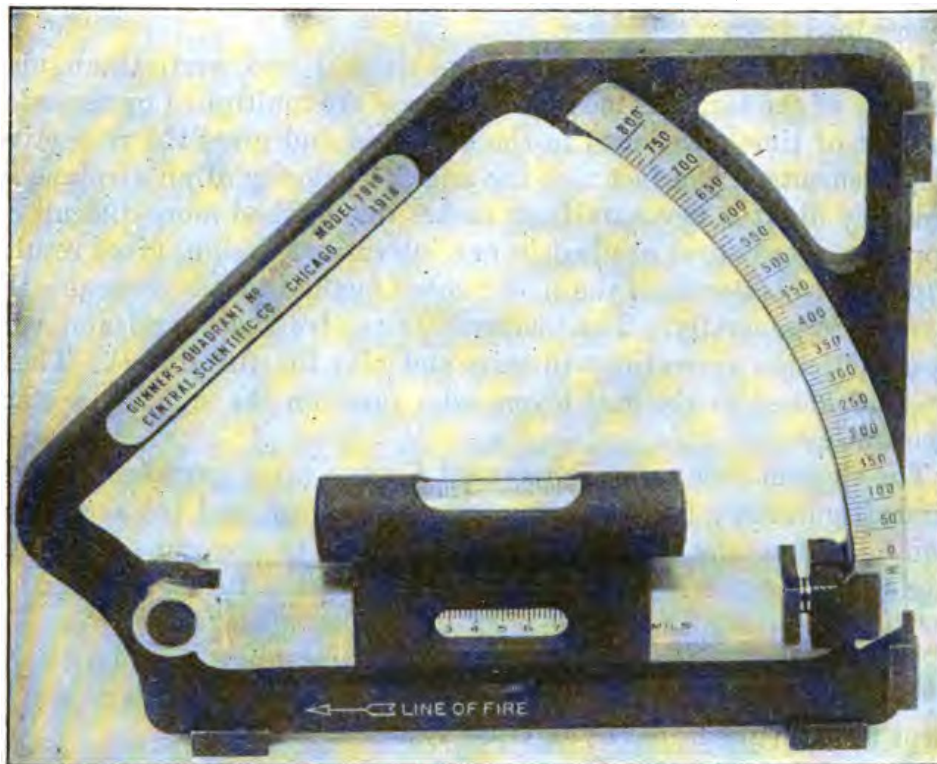
GUNNER'S QUADRANT, MODEL OF 1918.
