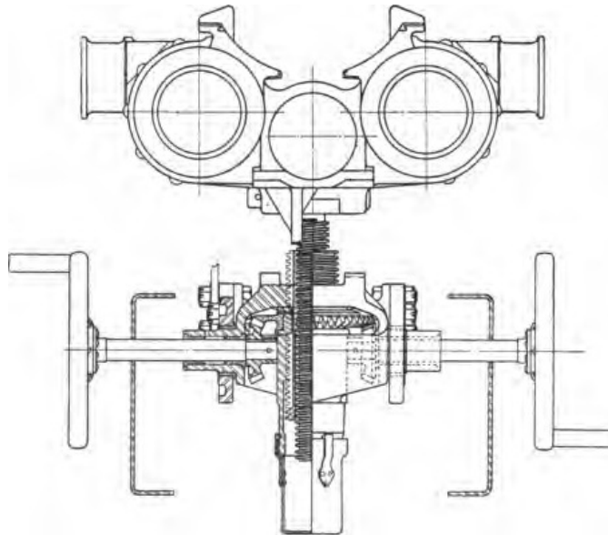
ELEVATING AND TRAVERSING MECHANISMS.
