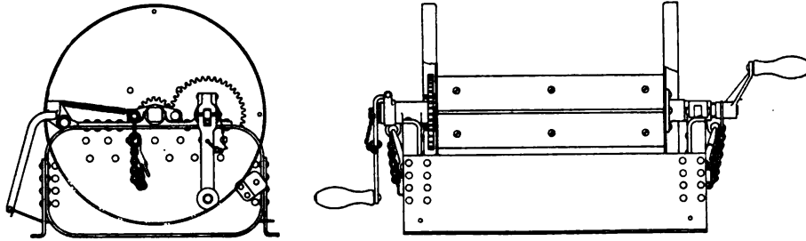
REEL FOR CAISSON, MODEL OF 1917.
