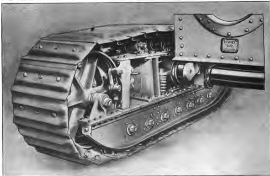
VIEW OF AXLE MOUNTED IN TRACK LAYER.
