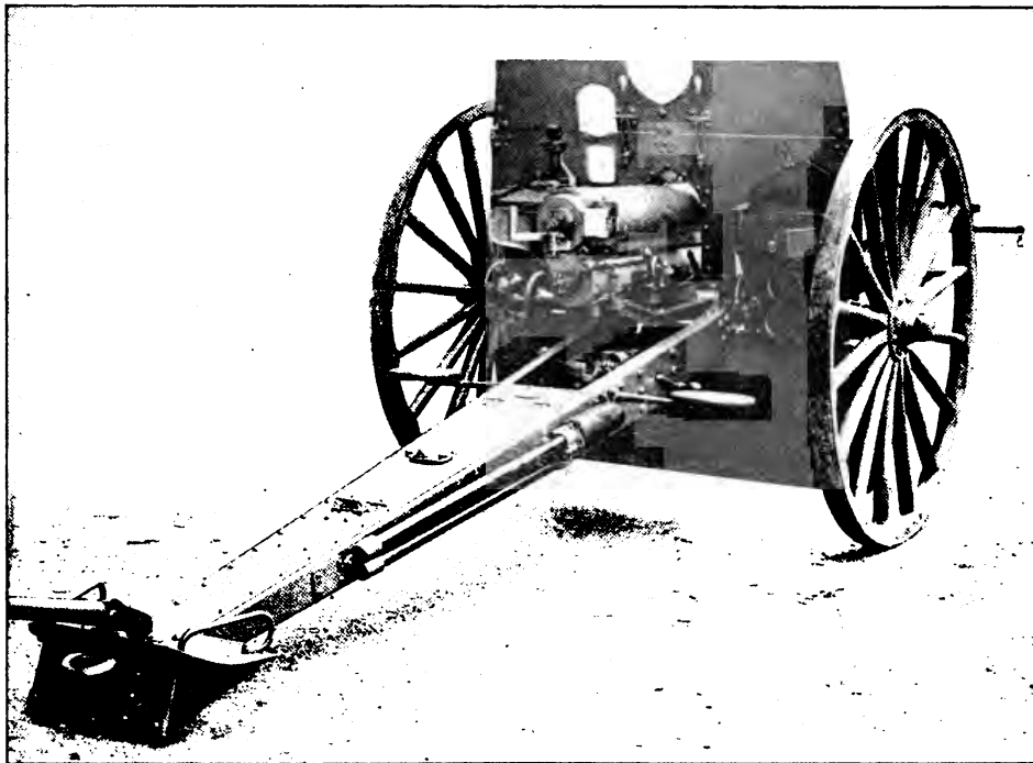
REAR VIEW OF CARRIAGE.
