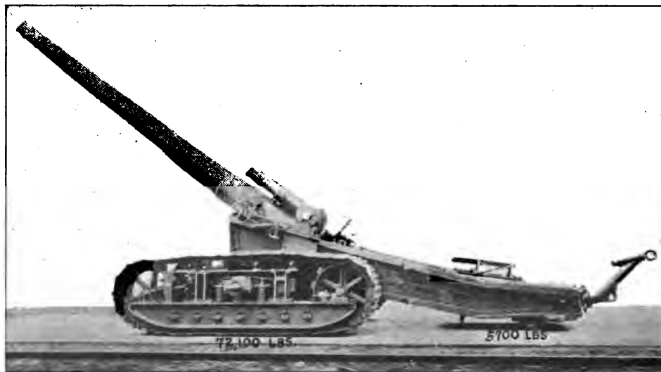
CARRIAGE IN BATTERY POSITION, SHOWING MAXIMUM ELEVATION OF GUN.
