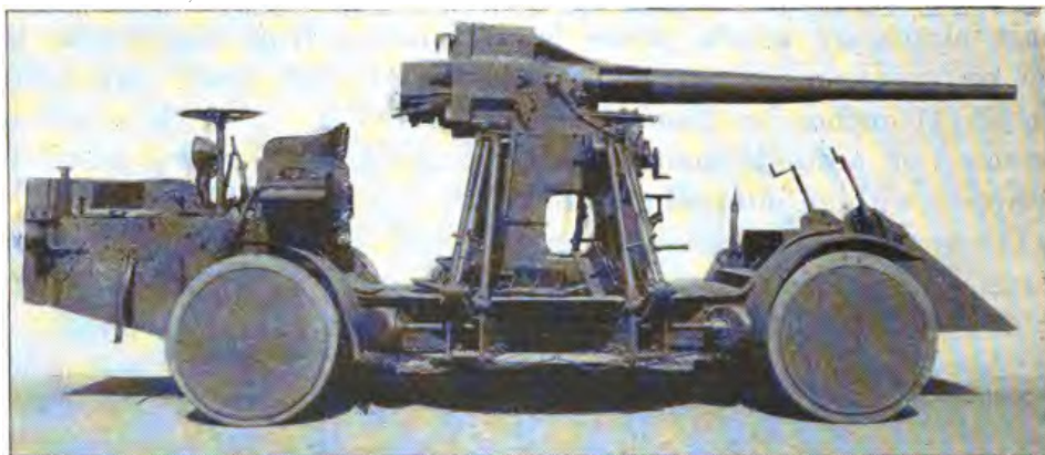
LEFT-SIDE VIEW OF MOUNT IN TRAVELING POSITION.
