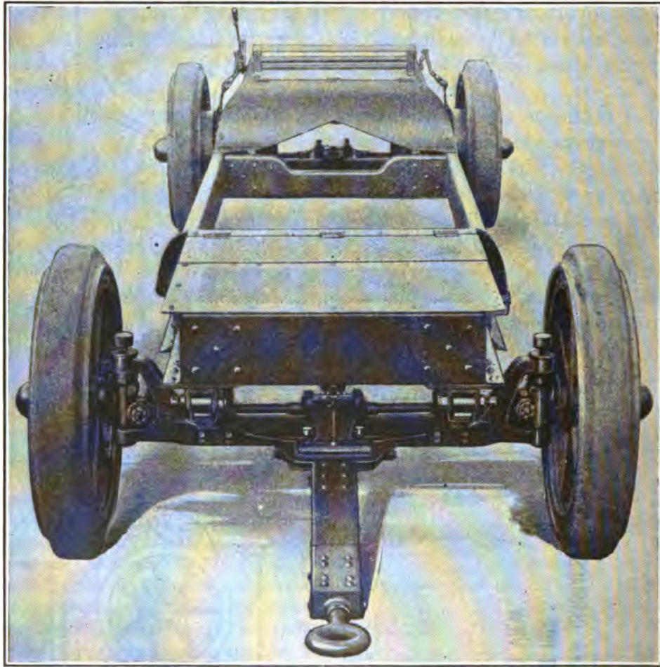
FRONT VIEW OF TRAILER.
