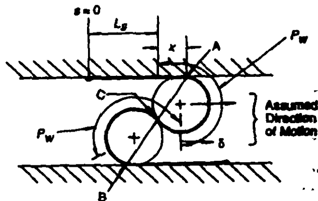
Figure 6-15. Energy Storage in a Rolamite Geometry (Ref. 8)
