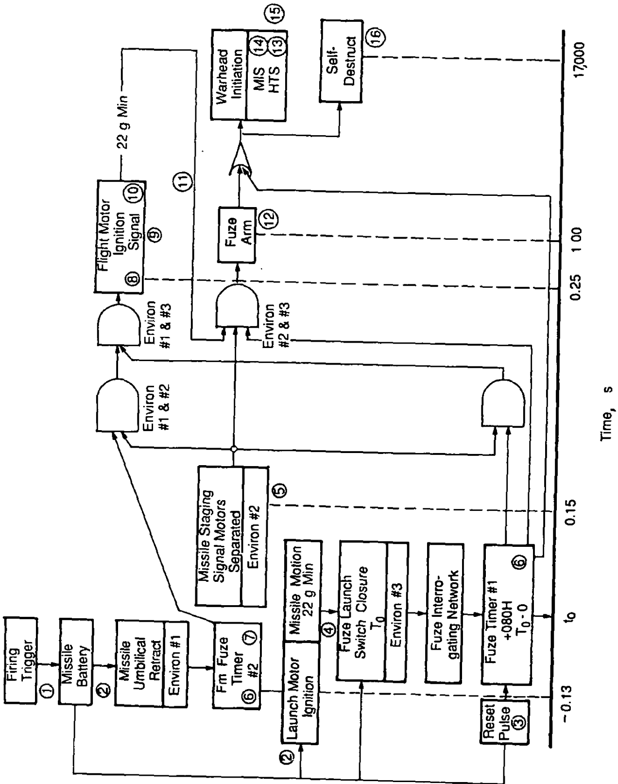
Figure 1-17. Function Diagram for STINGER Missile
