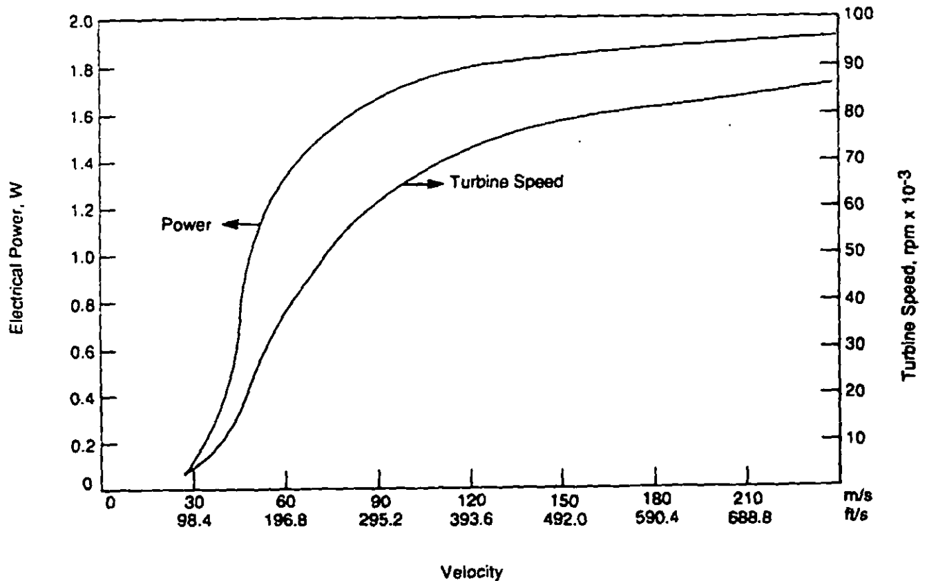
Figure 3-25. Performance Characteristics of Turboalternator
