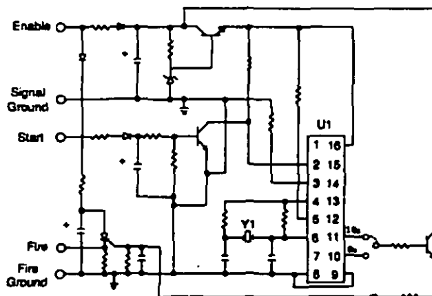
Figure 7-19. 16-Second Precision Ordnance Timer
