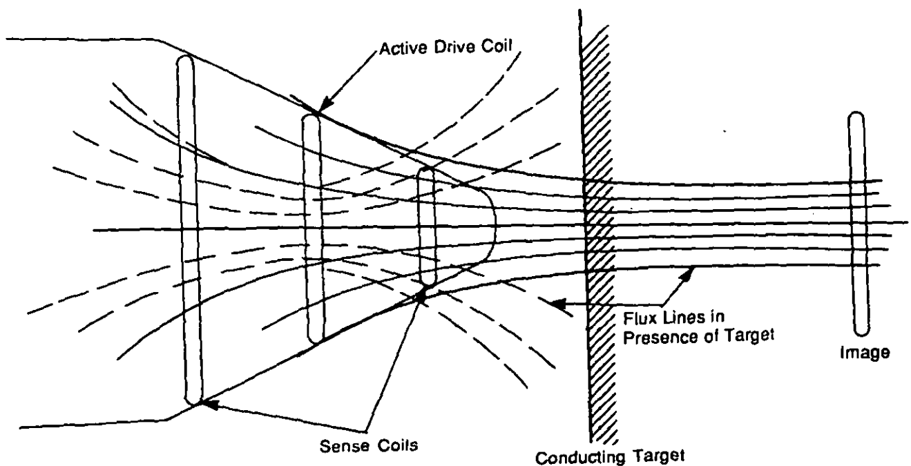
Figure 3-7. Inductive Sensing
