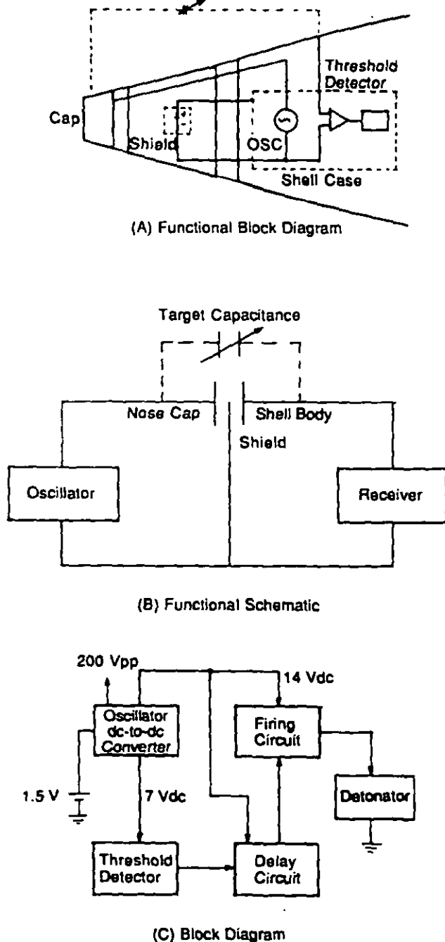
Figure 3-12. Schematics of Circuitry of Fuze XM588
