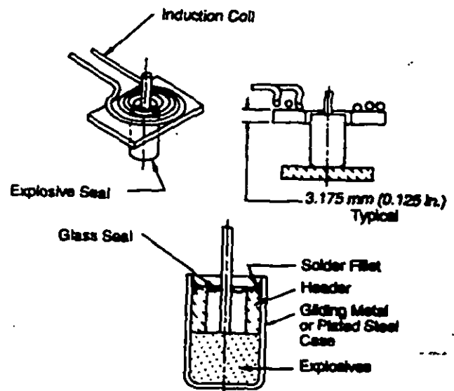
Figure 4-11. Induction Soldering (Ref. 19)
