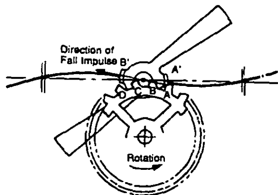
(A) Pallet Tooth Sliding Along Escape Wheel Tooth Face
