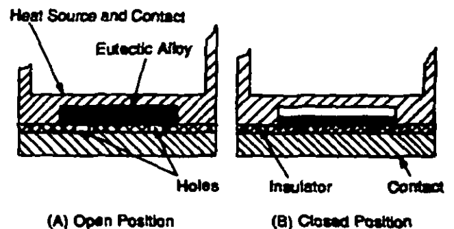
Figure 7-5. Thermal Delay Arming Switch (Ref. 2)
