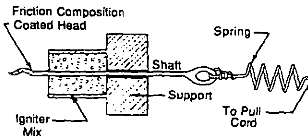
Figure 3-17. Firing Device, M2
