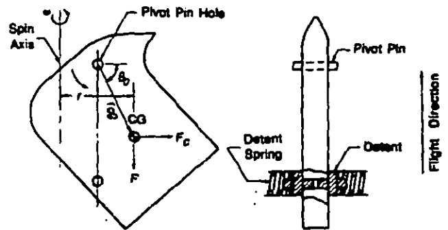
Figure 6-22. Sample Firing Pin
