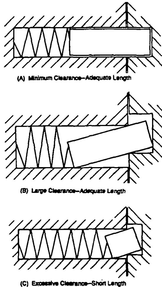
Figure 6-10. Detent Actions
