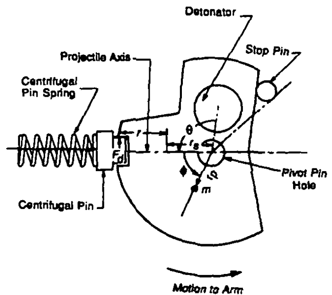
Figure 6-26. Rotary Shutter
