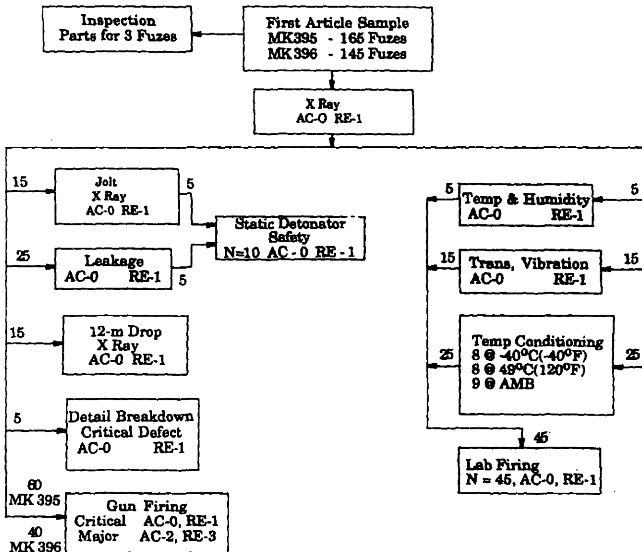
Figure 14-10. First Article Tests for MK 395 MODS 0 and 1 and MK 396 Mode Auxiliary Detonating Fuzes (Ref. 23)
