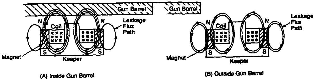
Figure 5-12. Sensor Inside and Outside Gun Barrel
