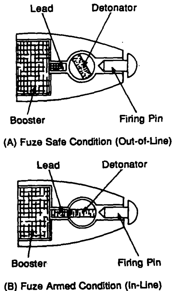
Figure 5-1. Simple Arming Device
