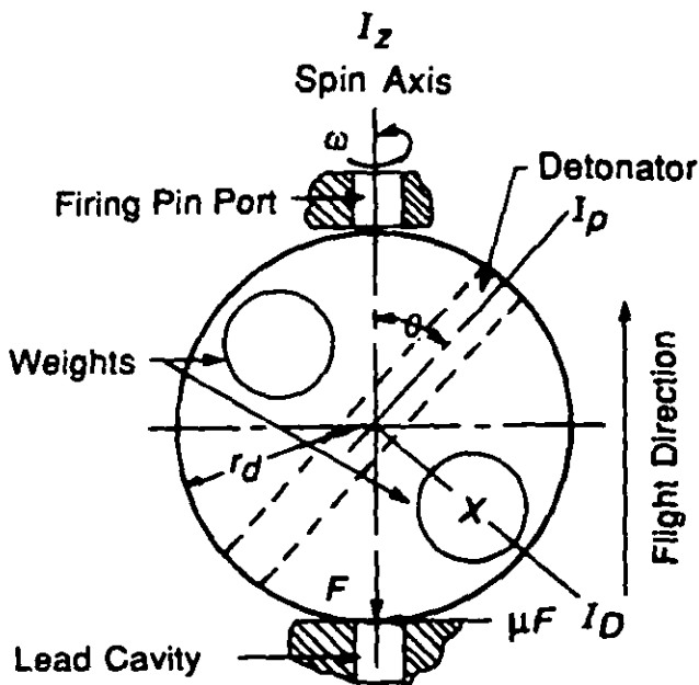
Figure 6-19. Disk Rotor
