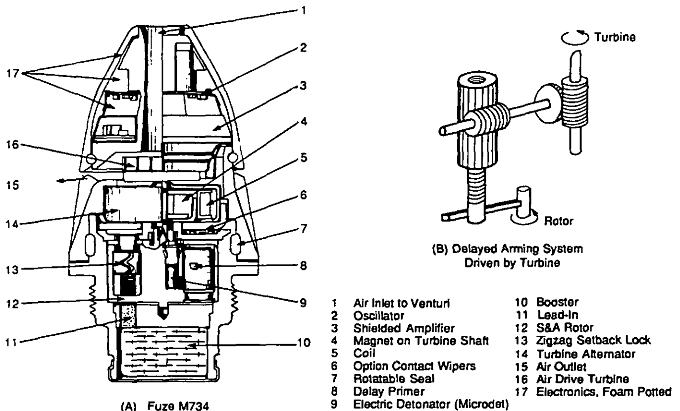
Figure 1-38. Fuze, Multioption, M734 (Ref. 22)
