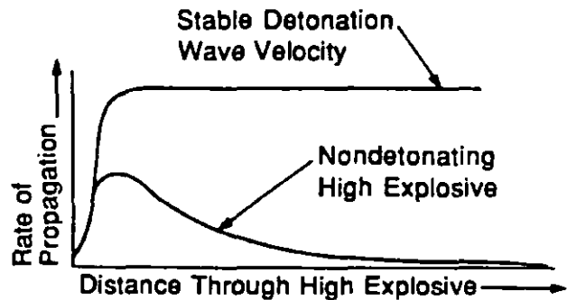
Figure 4-3. Examples of Good and Poor Detonations
