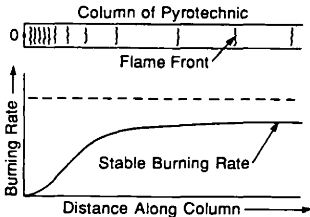
Figure 4-1. Burning Pyrotechnic
