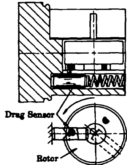
(D) Condition Following Release of Rotor Without Drag Signature (Rotor Locked in Fail-Safe Position)
