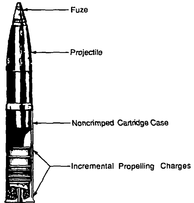
Figure 1-3. Semifixed Ammunition
