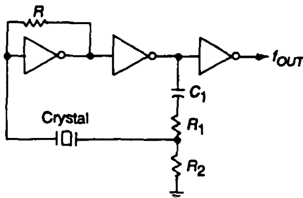
(A) Series Oscillator, 1/2 CD 4069
