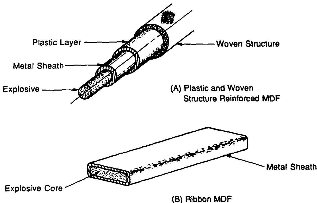
Figure 4-17. Types of Detonating Fuses
