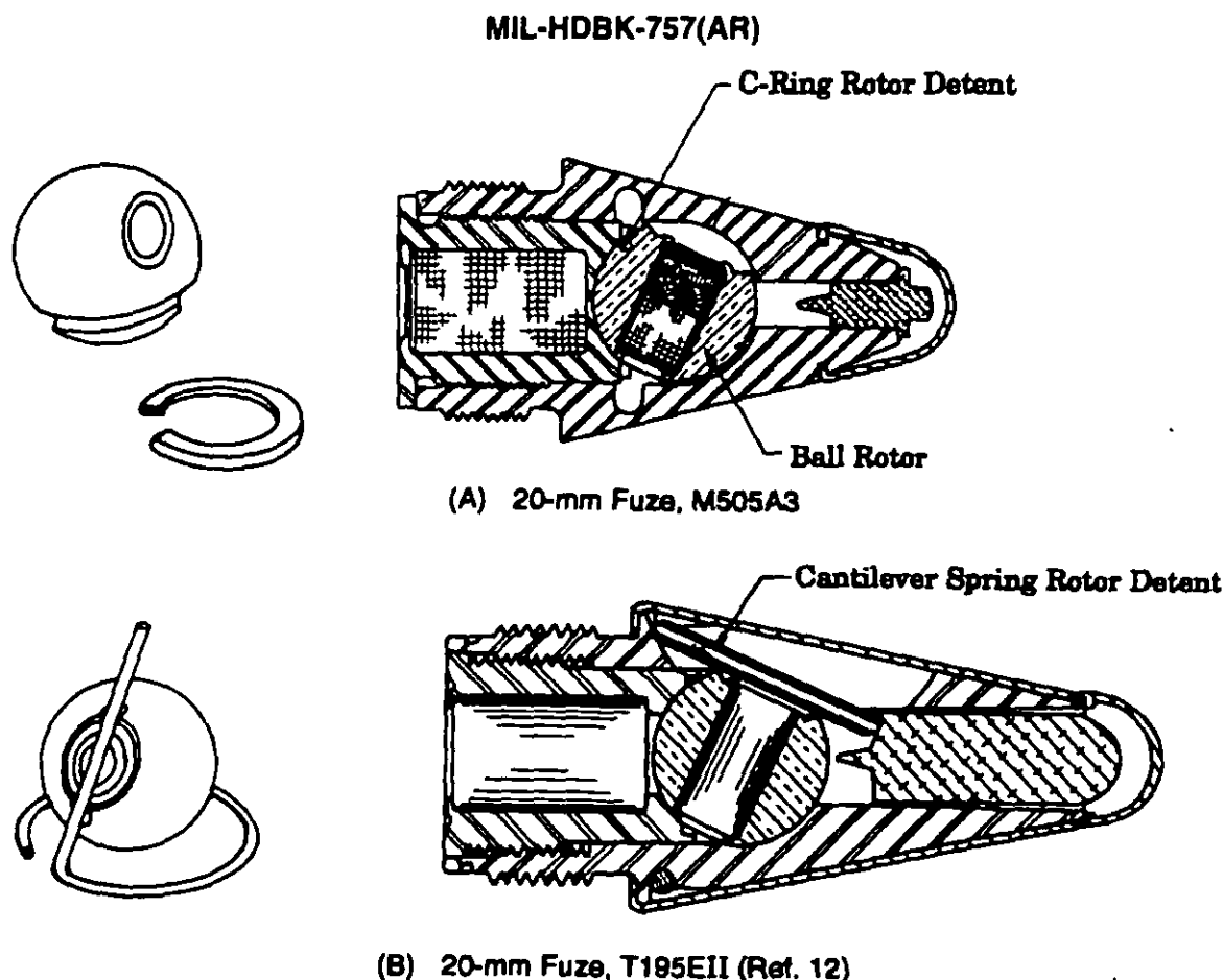
Figure 6-29. C-Ring and Cantilever Spring Methods of Holding Ball Rotor
