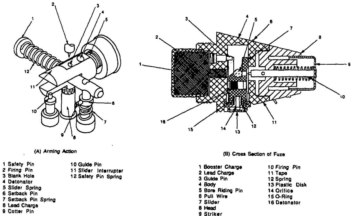
Figure 2-9. Arming Action for Fuze, PD M717
