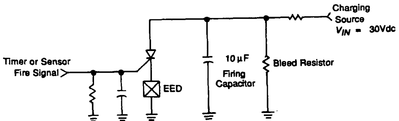
Figure 7-33. High- and Low-Energy Capacitive Discharge Firing Circuits
