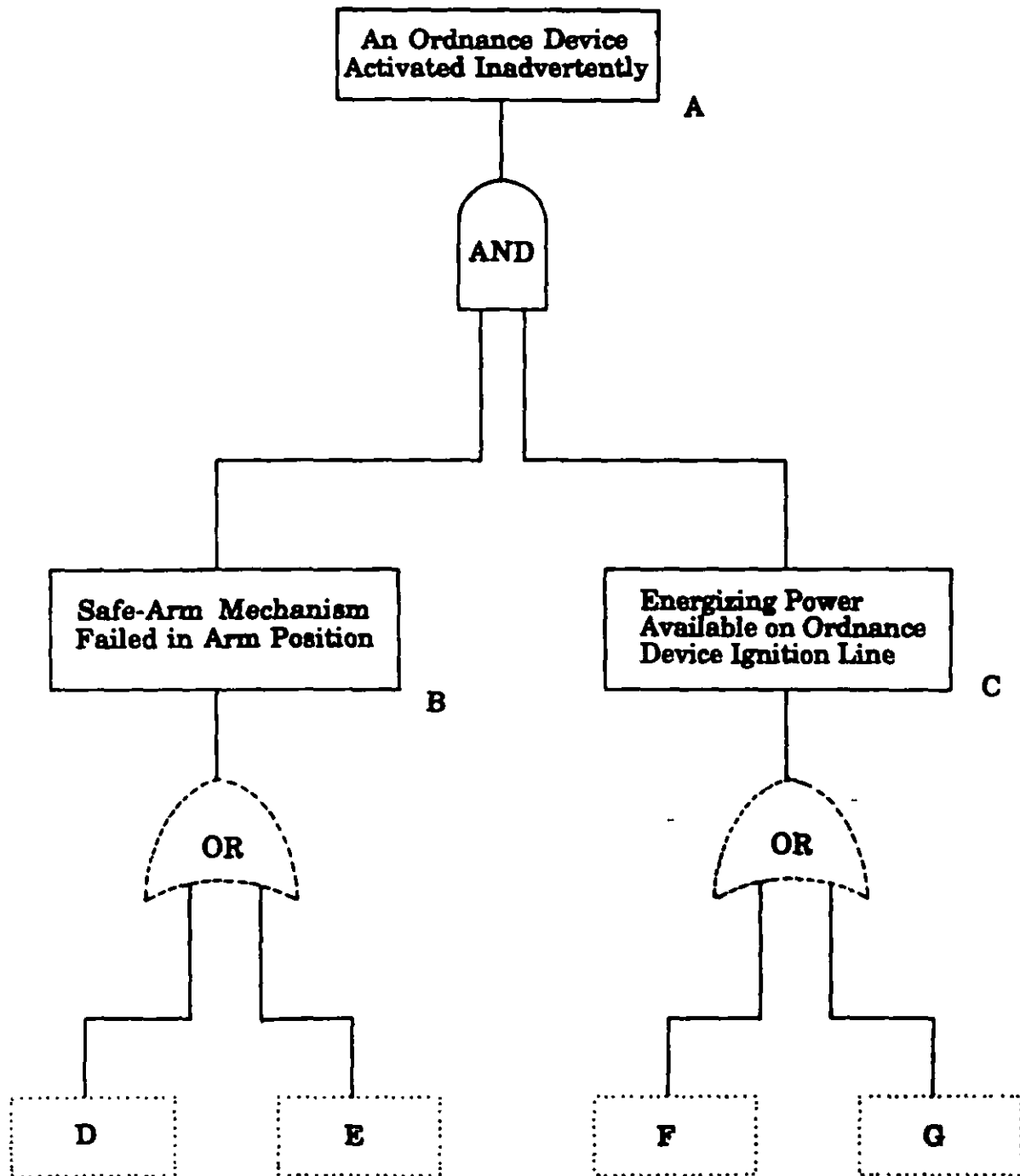
Figure 13-9. Simplified Fault Tree Analysis for Hypothetical Weapon System
