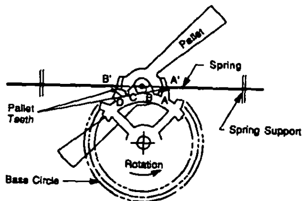
(B) Pallet at Equilibrium
