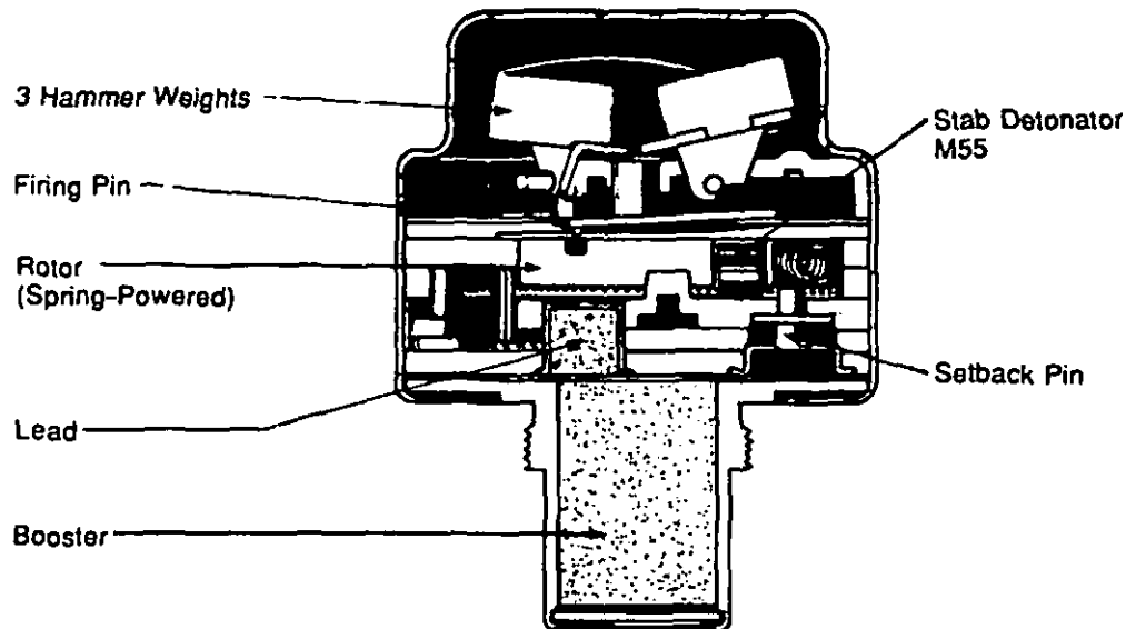
(B) Fuze Firing Mechanism and Explosive Train
