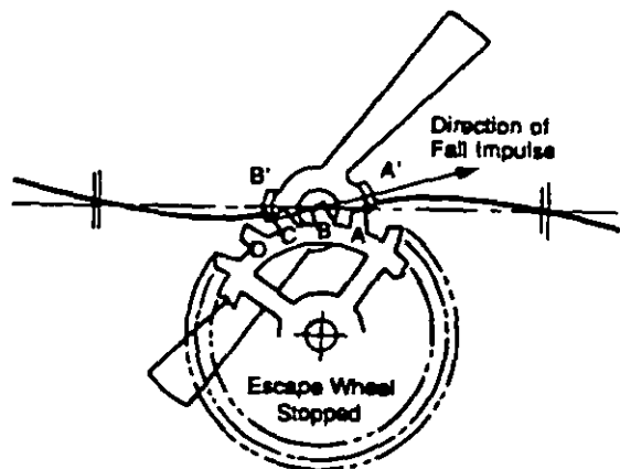
(C) Escape Wheel Tooth Falling on Pallet Tooth
