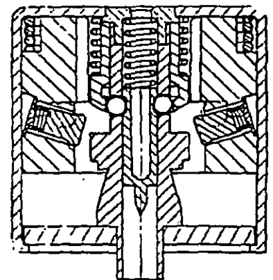
(C) At Target Impact
