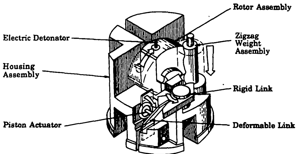
(B) Armed Position
