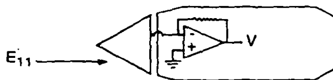
Figure 3-8. Short-Circuit Longitudinal Probe Configuration for Electrostatic Fuze
