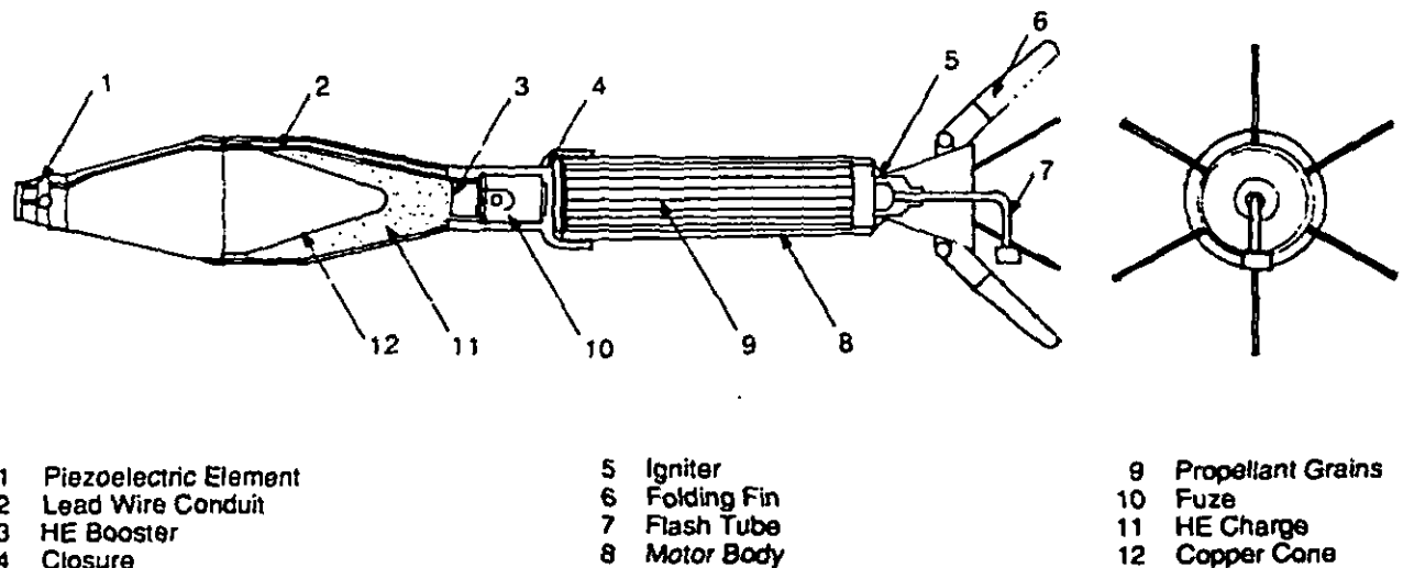
Figure 1-14. 66-mm (2.60-in.) Light Antitank Weapon Rocket
