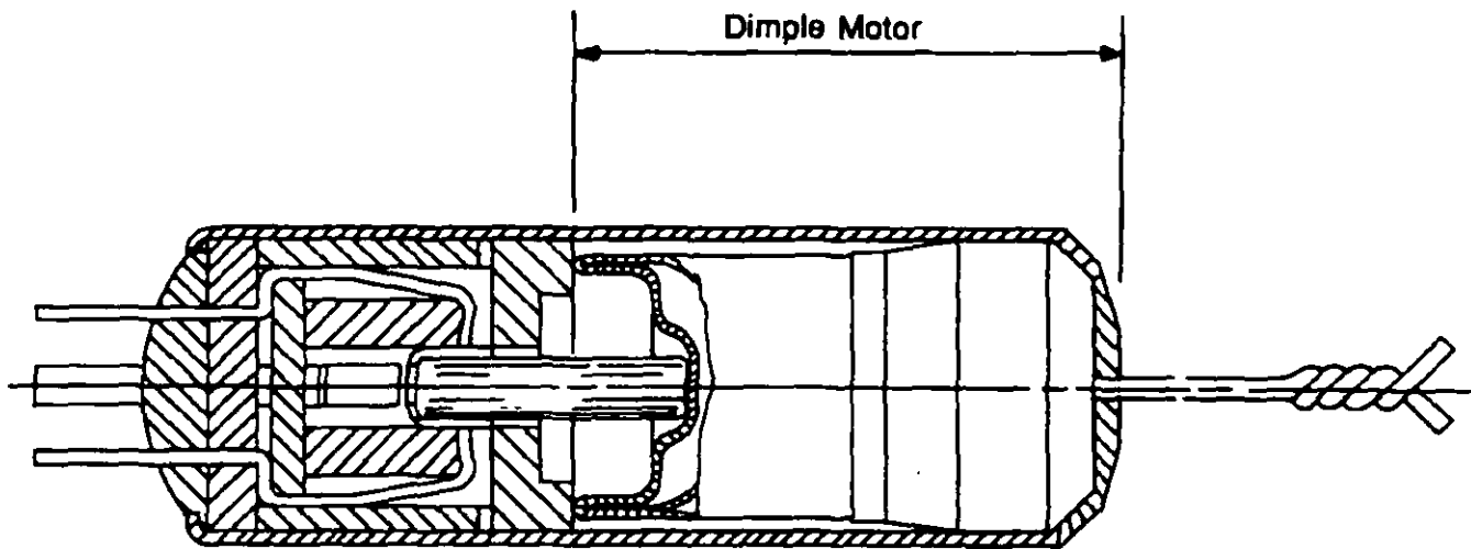
Figure 7-10. Switch, Electroexplosive, MK 127 MOD 0 (Ref. 4)
