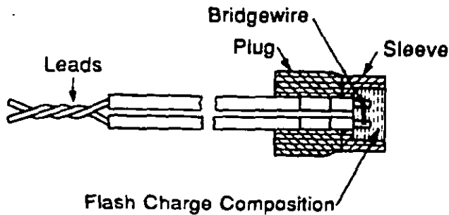
Figure 4-6. Electrical Initiator, Squib M2
