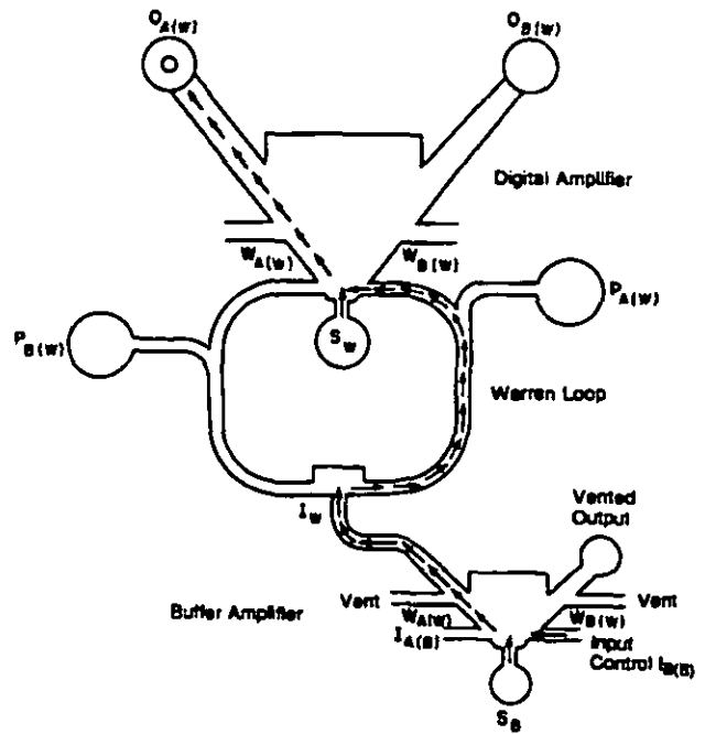
Figure 8-2. Schematic of Fluoric Counter Stage (Ref. 4)
