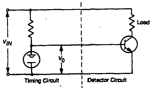
Figure 7-39. Bissett-Berman E-Cell (Ref. 18)
