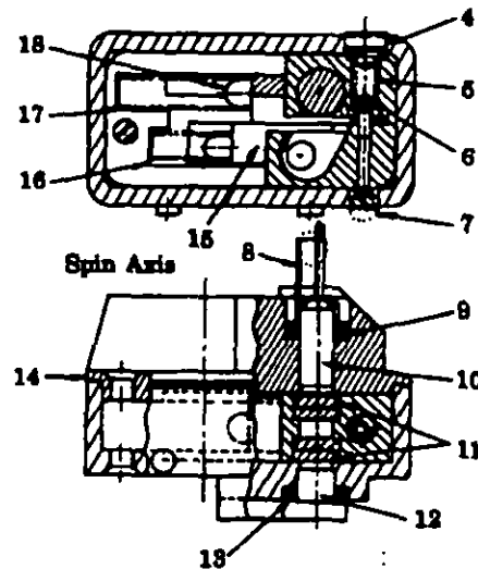
(B) ADAM Fuze
