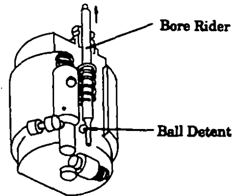
(B) Release of Bore Rider by Pyrotechnic Delay
