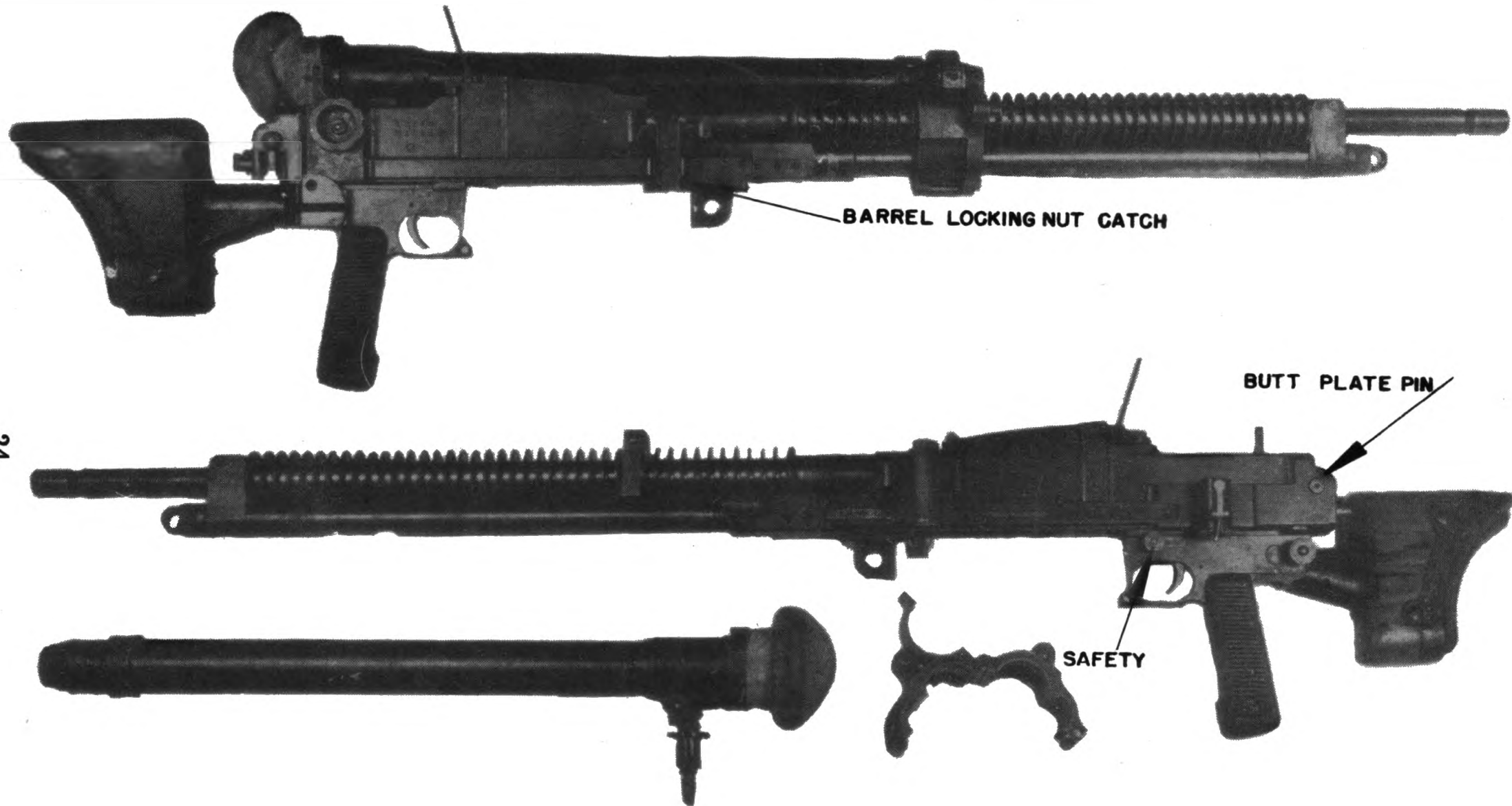
At the lower left hand side are shown the telescopic sight unmounted and the sight bracket. In the upper picture the sight is shown as mounted on the machine gun.
