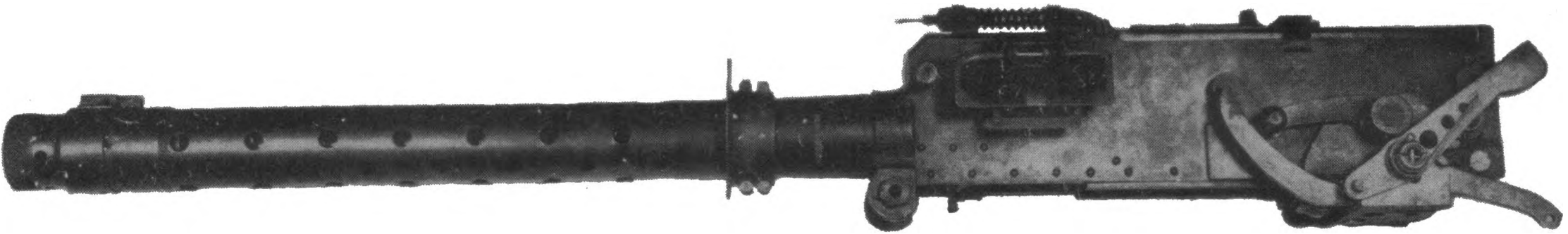
MACHINE GUN, 7.7 MM, AIRCRAFT, TYPE 89 (1929)
