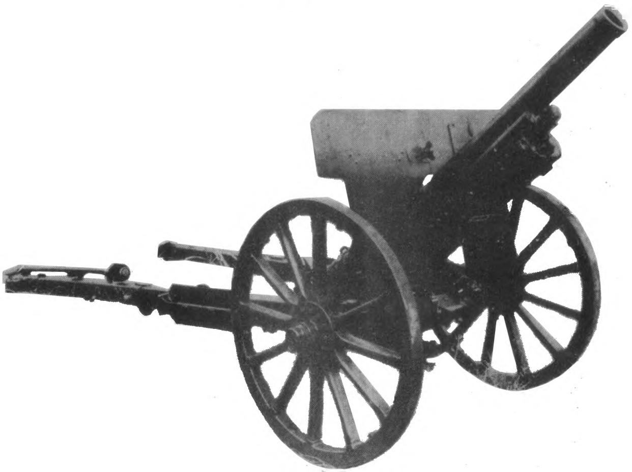
75 MM MOUNTAIN GUN, TYPE 94 (1934) Shown above with trails closed and below with trails spread and in position for high angle fire.
