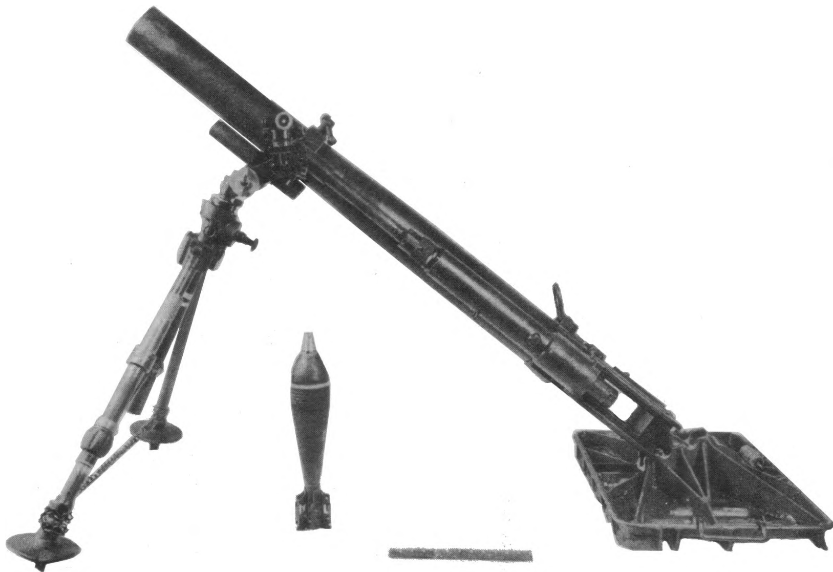
90 MM MORTAR, TYPE 94 (1934) Shown with a standard high explosive shell.
