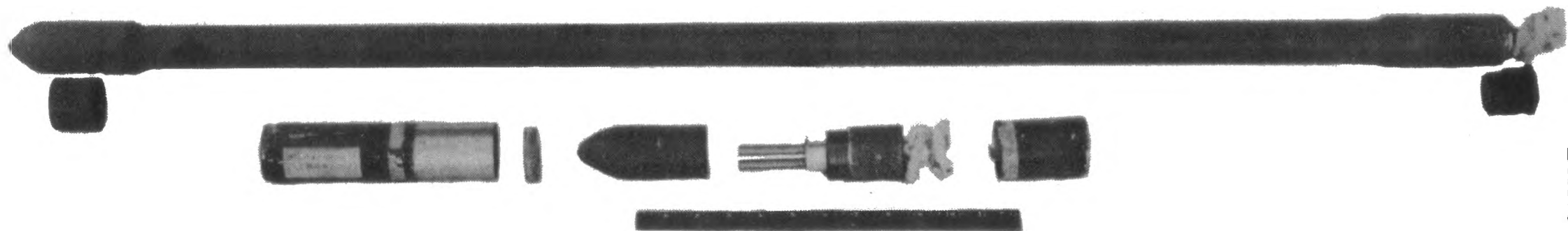
BANGALORE TORPEDO, TYPE 99 (1939) Shown at the top with fuze in place on the right and the pointed head in place at the left. Fuze shown at the bottom.
