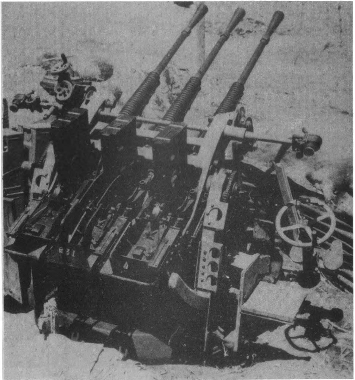
AUTOMATIC CANNON, 25 MM, ANTI-AIRCRAFT, TRIPLE MOUNT, 3/4 rear view
