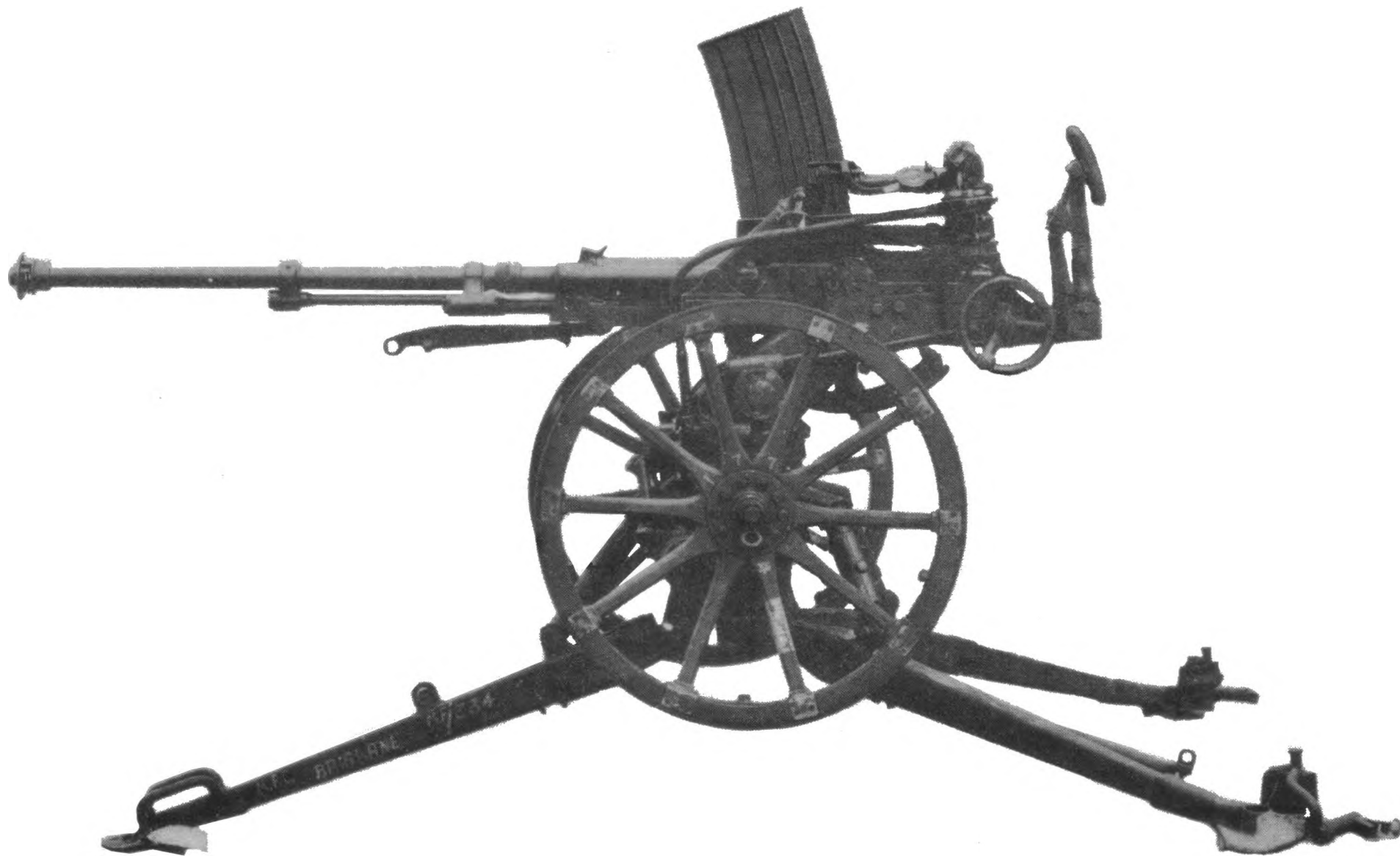
AUTOMATIC CANNON, 20 MM, AA/AT, TYPE 98 (1938) Shown in position for firing at a low elevation.
