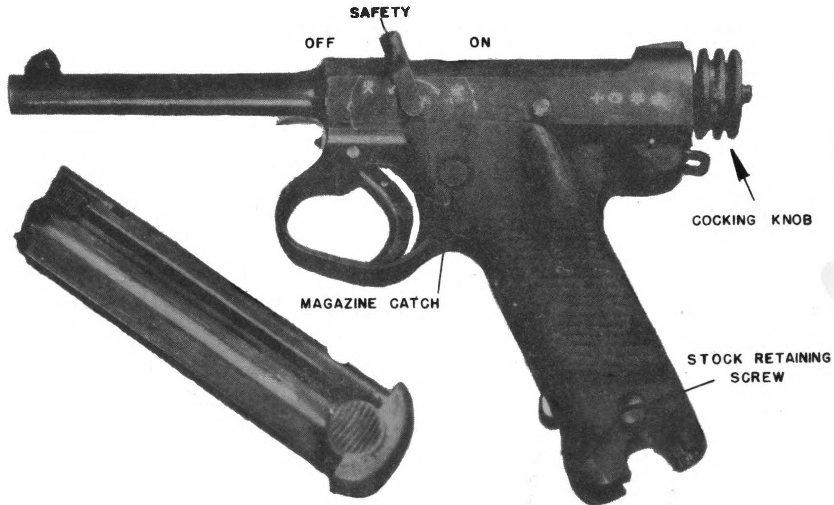
PISTOL, AUTOMATIC, 8 MM, TYPE 14 (1925) Empty Magazine is shown in the lower left hand corner
