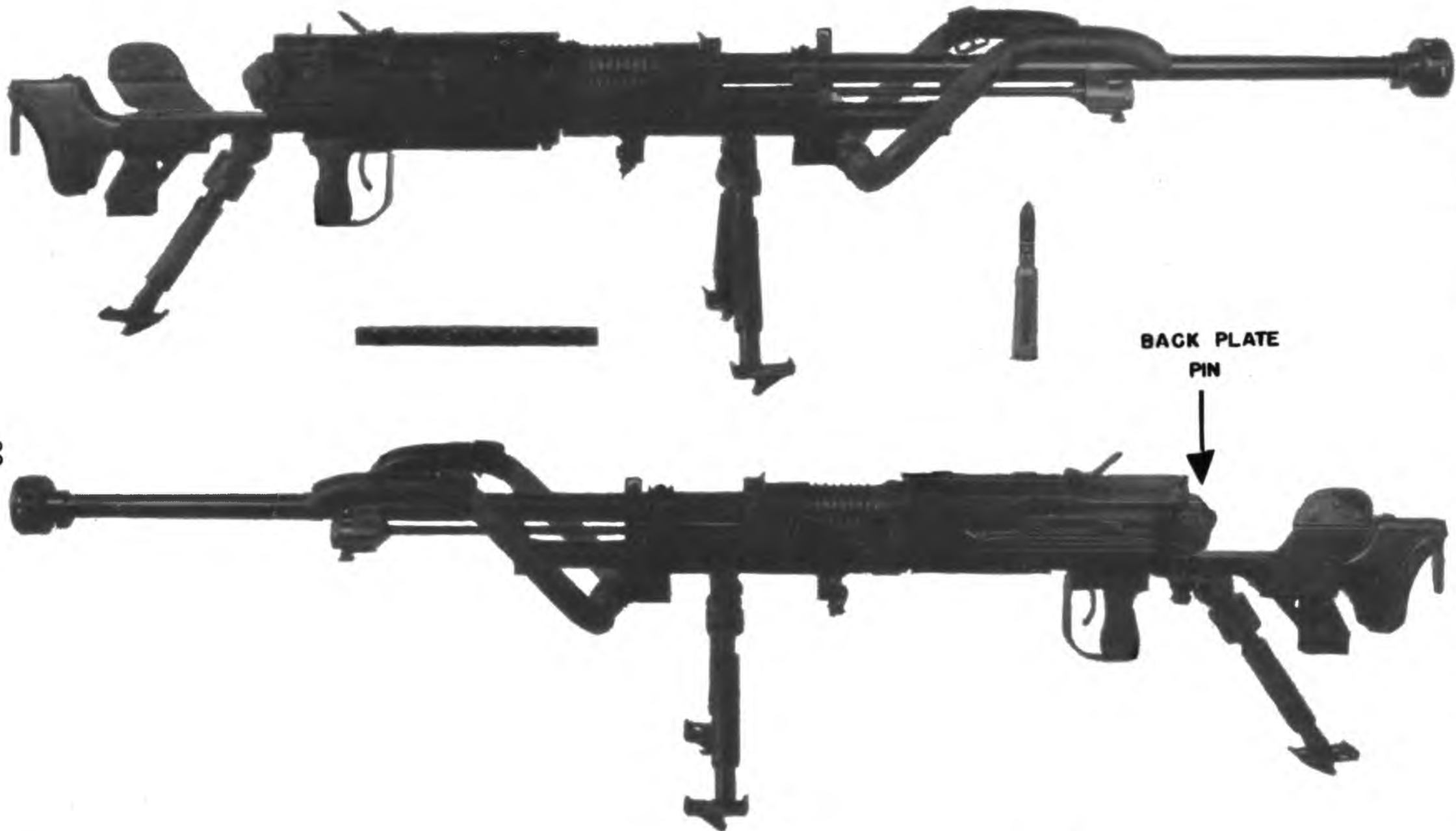
AUTOMATIC CANNON, 20 MM, ANTI-TANK, TYPE 97 Shown above are right and left hand views of this weapon.
