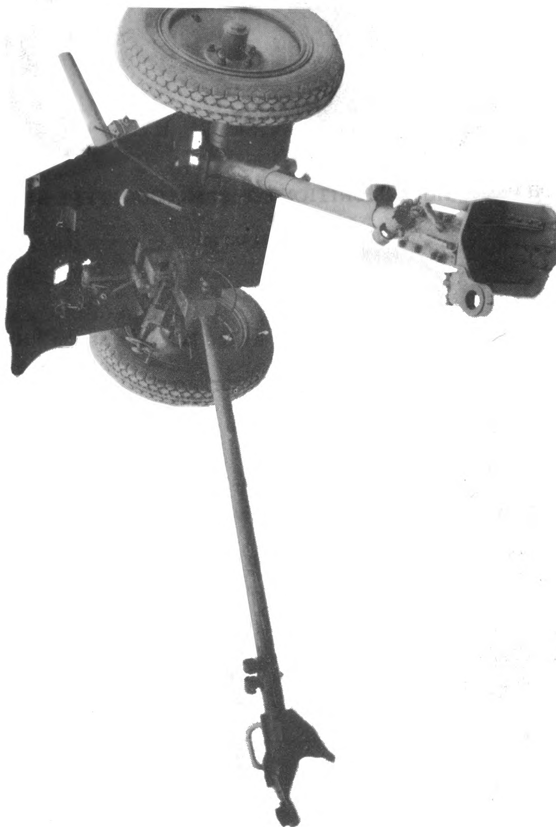
37 MM GUN, ANTI-TANK, TYPE 97 (1937)
