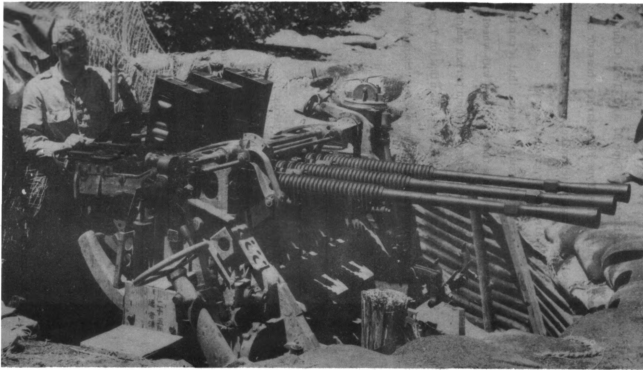
AUTOMATIC CANNON, 25 MM, ANTI-AIRCRAFT, TRIPLE MOUNT, 3/4 front view.
