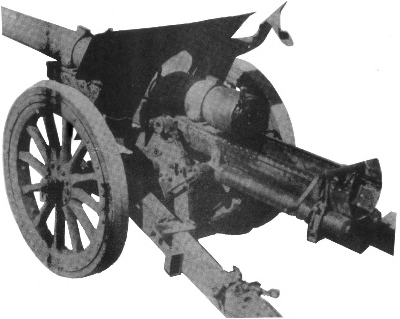
105 MM GUN, TYPE 92 (1932)
