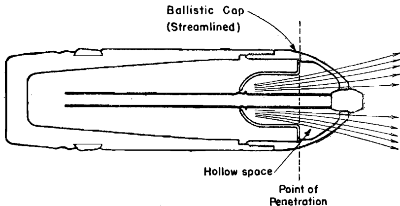
Figure 3.—Hollow-charge Principle.
