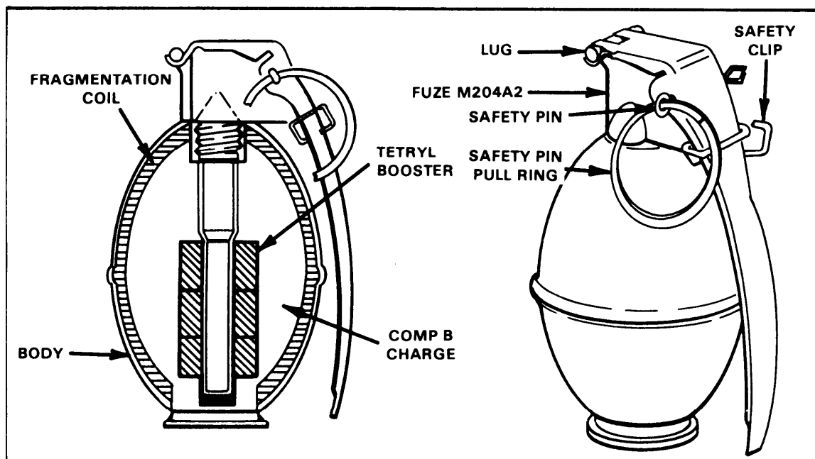
Figure 1-9. M61 fragmentation grenade.
