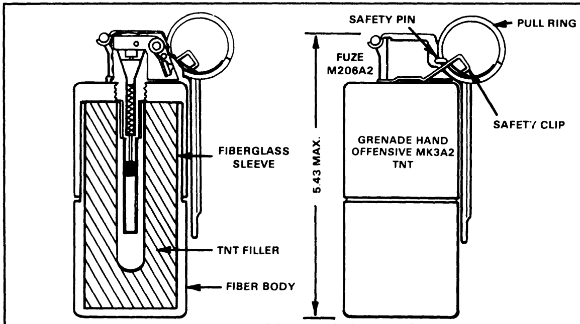
Figure 1-17. MK3A2 offensive grenade.
