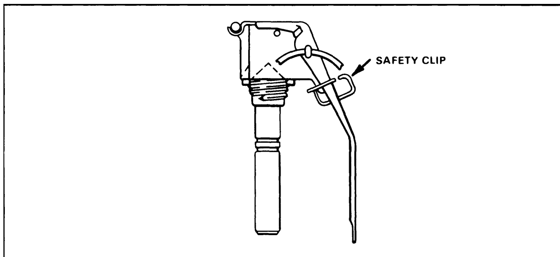
Figure 1-5. M213 fuze.
