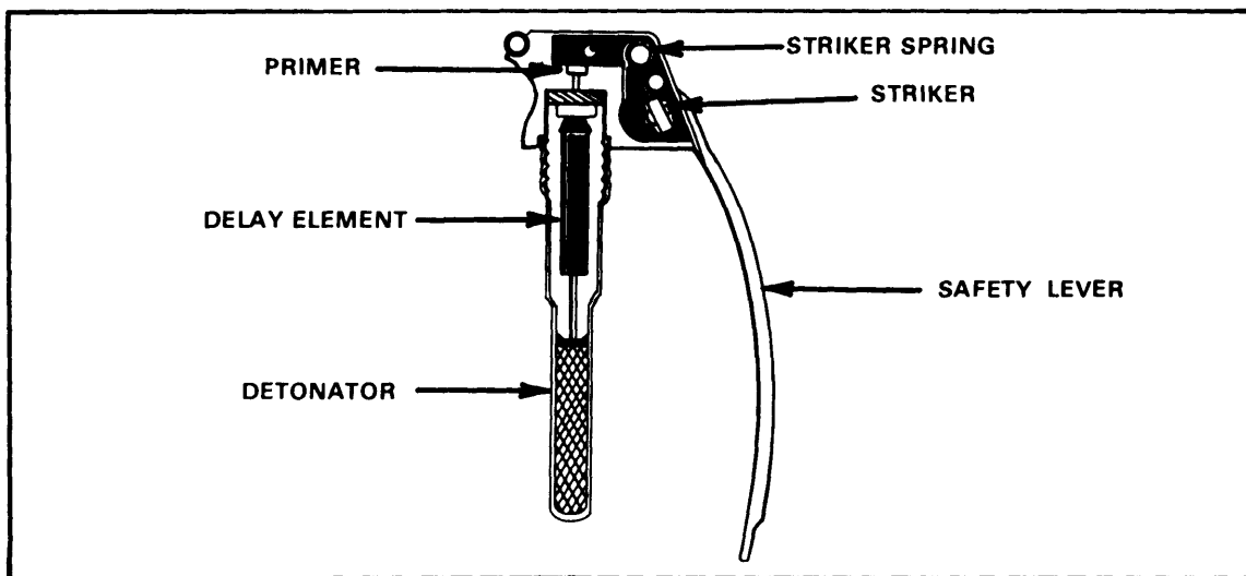
Figure 1-3. M204A2 fuze.
