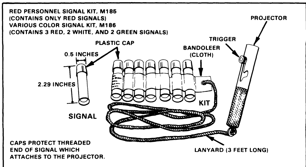
Figure 5-8. Signal kit 1.
