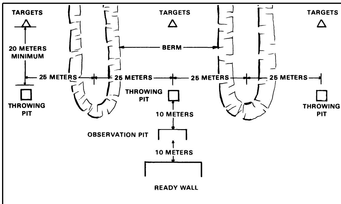
Figure E-1. Range layout.
