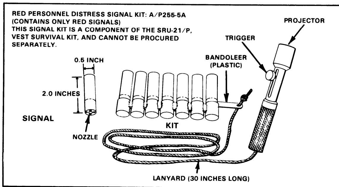
Figure 5-9. Signal kit 2.
