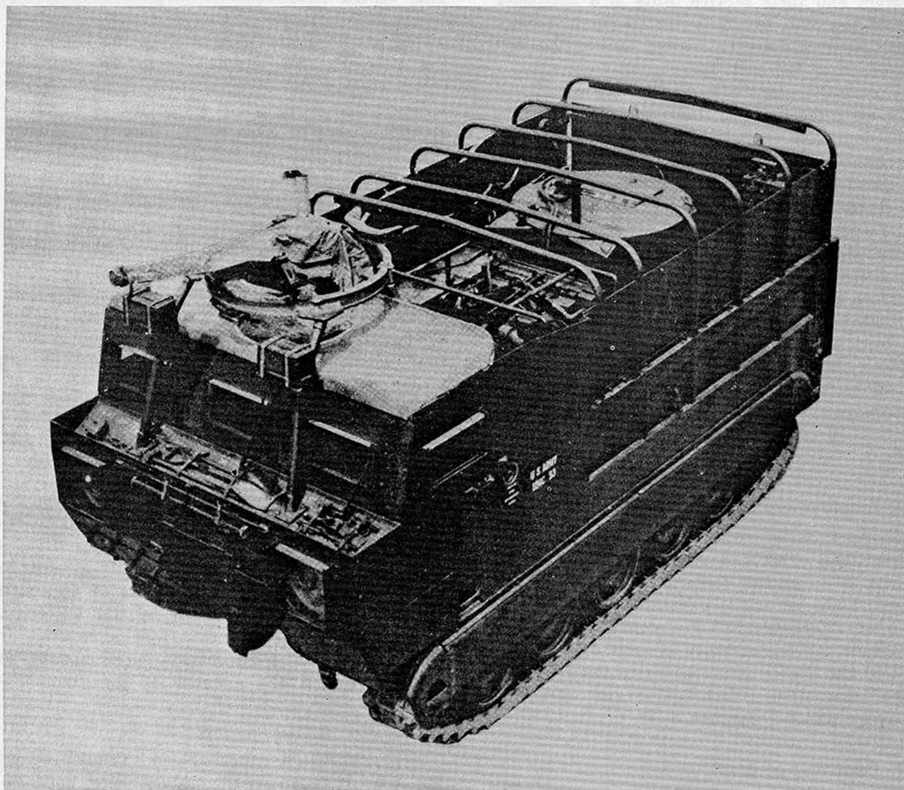
Figure 4-5. XM45E1 tracked-vehicle mounted flamethrower service unit.
