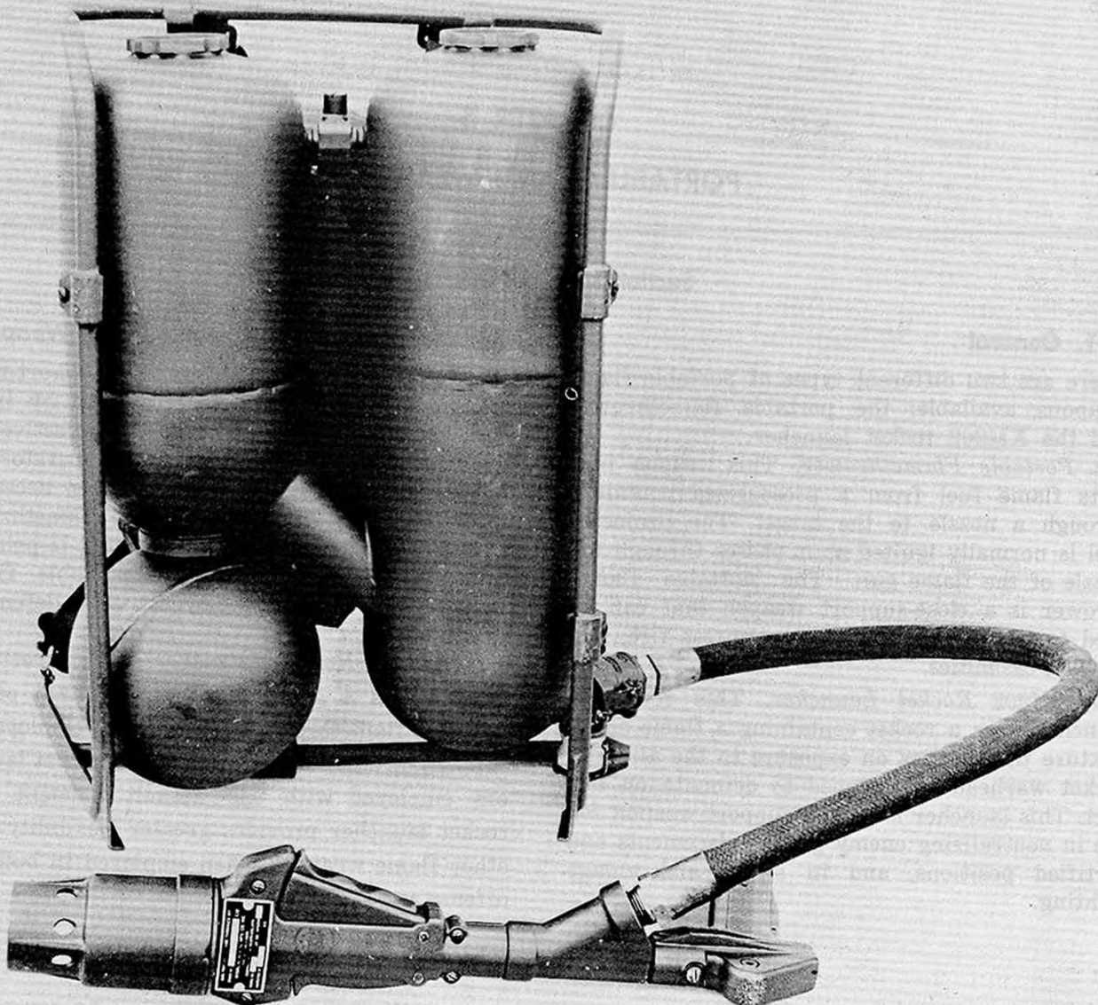
Figure 5-1. ABC-M9-7 portable flamethrower.
