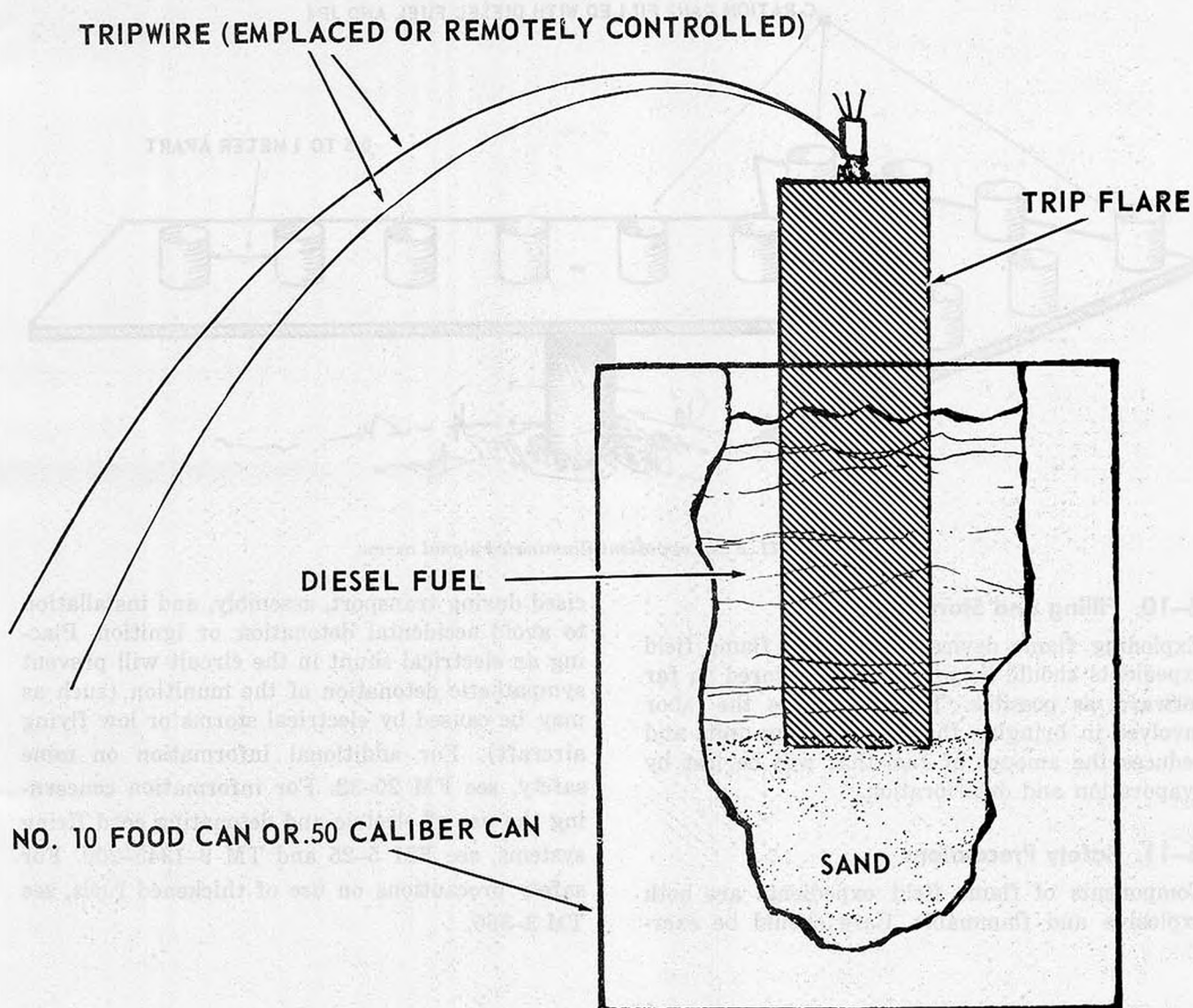
Figure 6-10. Field expedient illuminator.
