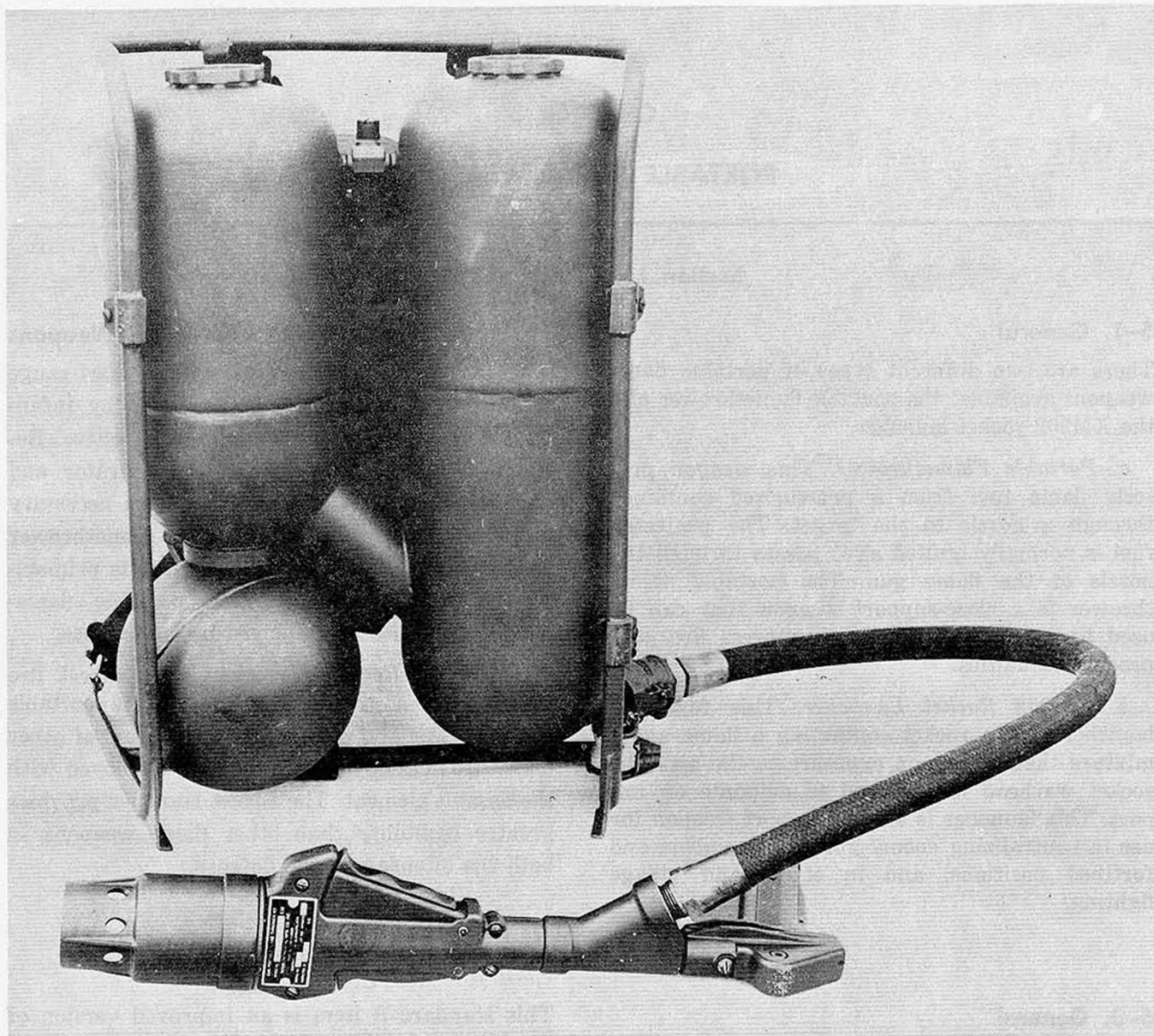
Figure 5-1. ABC-M9-7 portable flamethrower.
