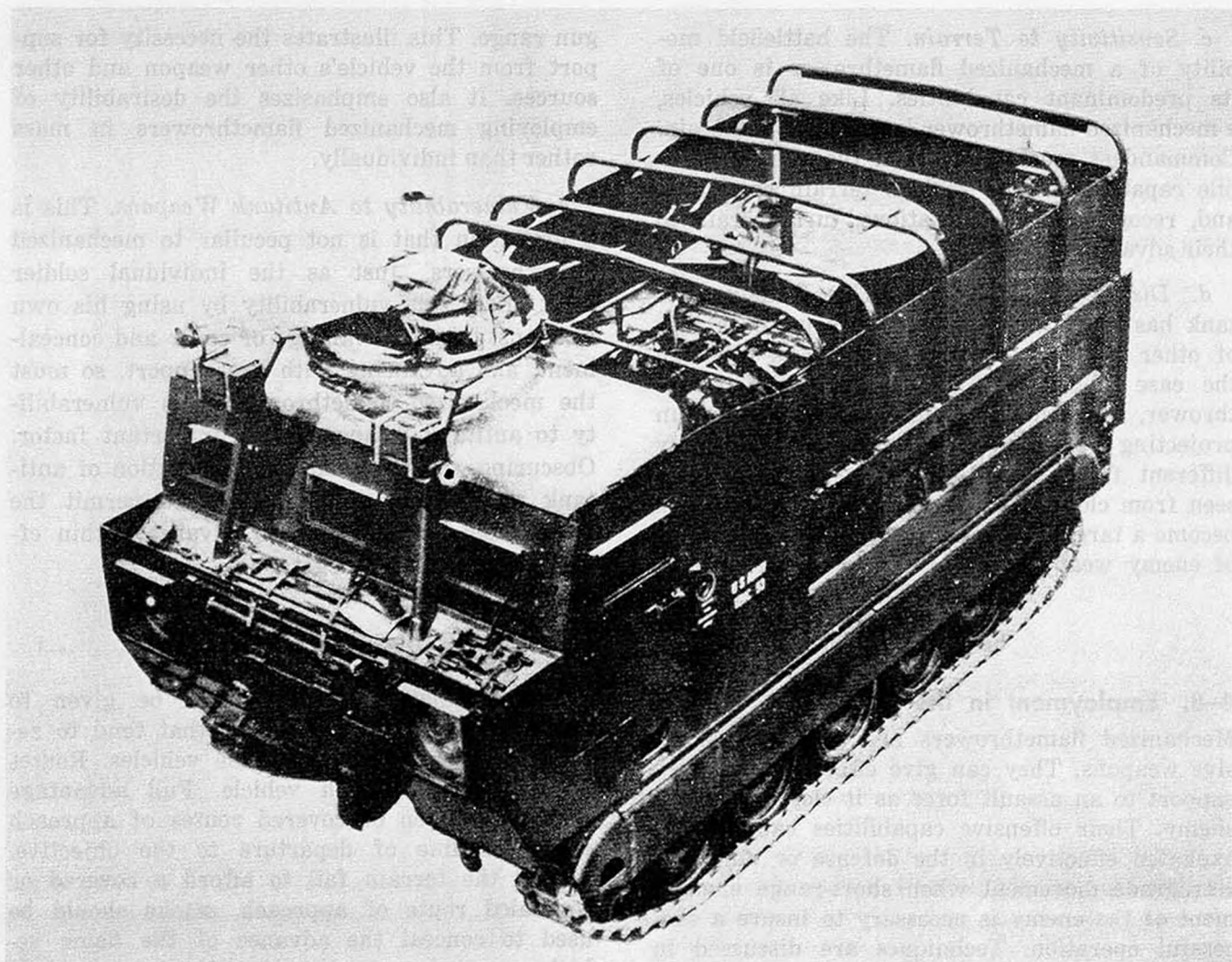
★Figure 4-5. M45 tracked-vehicle mounted flamethrower service unit.
