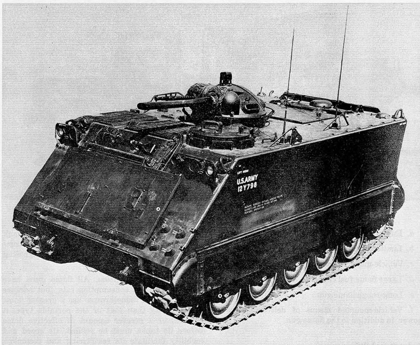
Figure 4-3. M132A1 self-propelled flamethrower.
