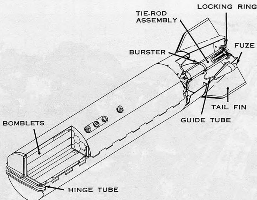
Figure 7-8. M74-type incendiary bombs, 57 10-pound bomblets in M35 cluster.
