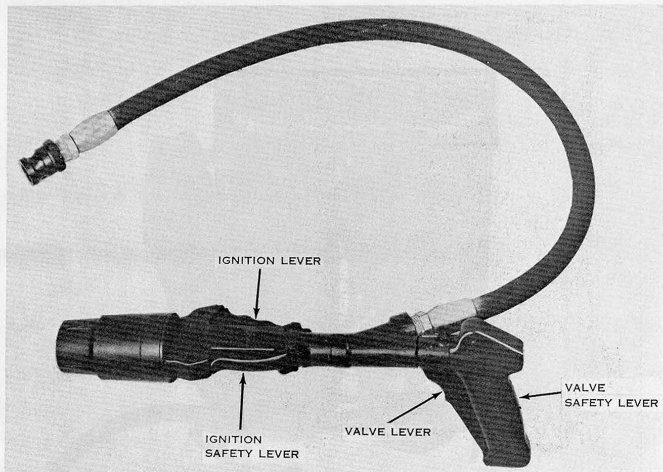
Figure 5-2. M7 flame gun group.
