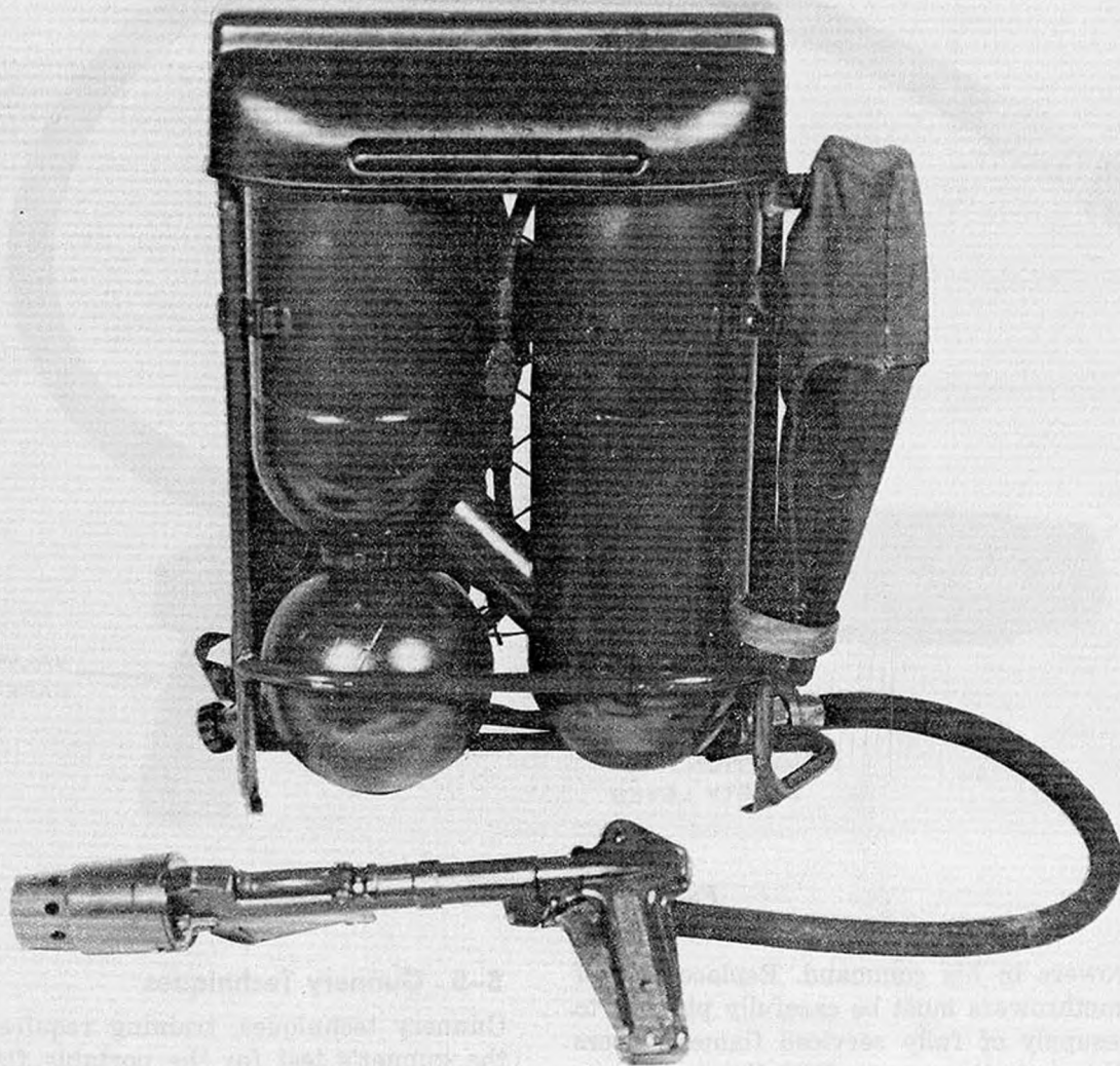
Figure 5-3. M9E1-7 portable flamethrower.
