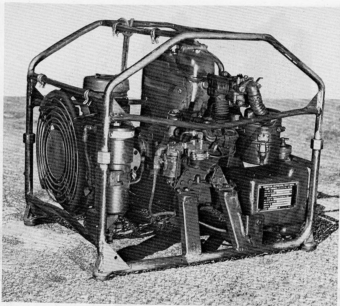
Figure 5-5. AN-M4 3 1/2 CFM flamethrower power-driven reciprocating compressor.
