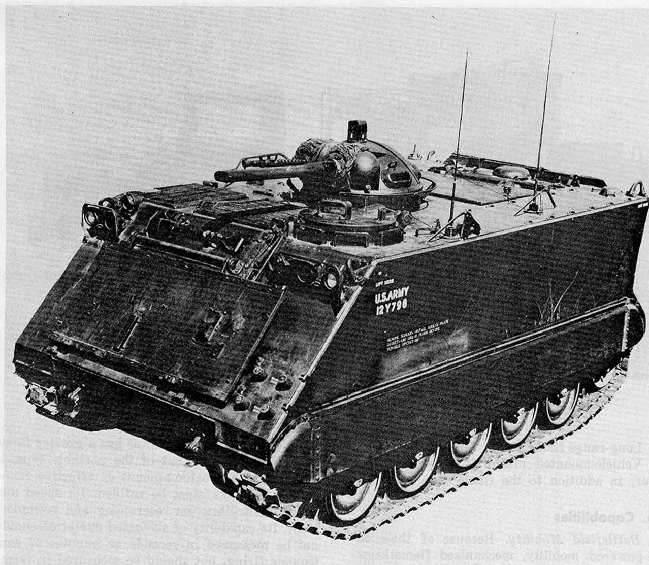
Figure 4-3. M132A1 self-propelled flamethrower.
