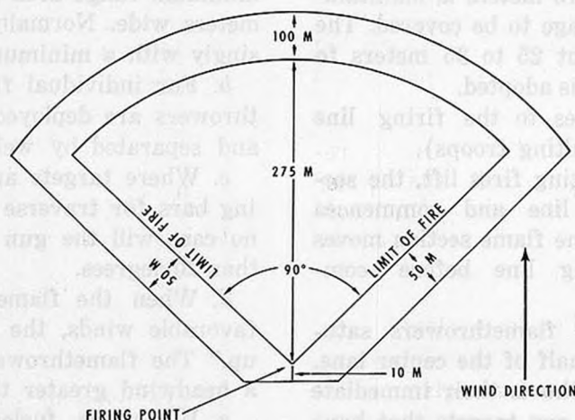
Figure C-4. Surface danger zones when firing the mechanized flamethrower.
