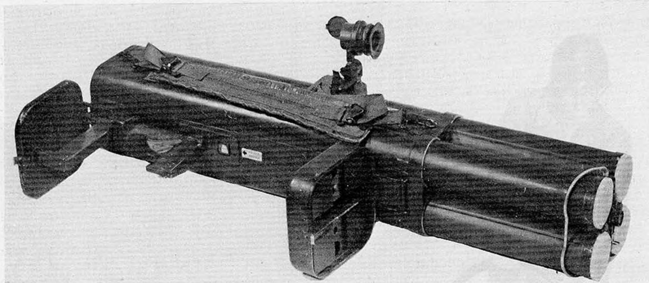
Figure 5-9. XM202 rocket launcher with rocket clip.
