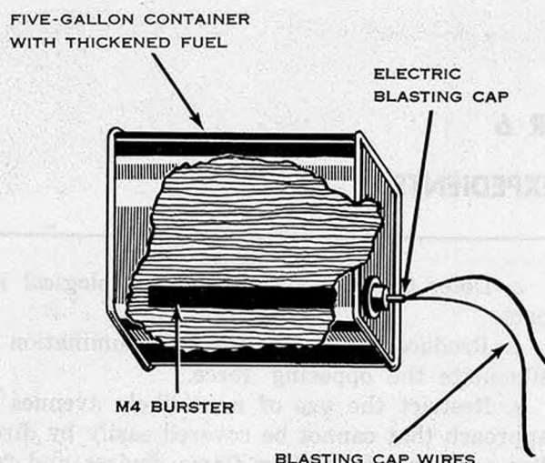
Figure 6-1. Exploding 5-gallon flame device with M4 burster.
