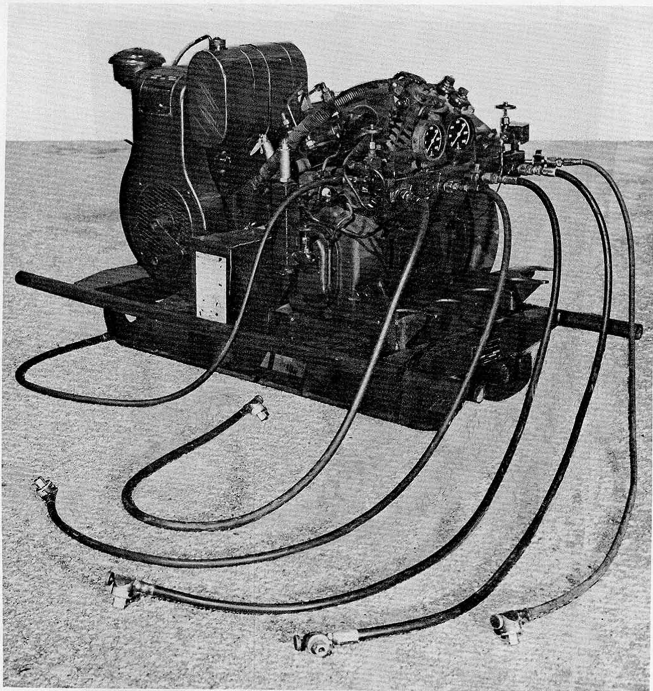
Figure 5-6. M1A1 7 CFM power-driven reciprocating compressor.
