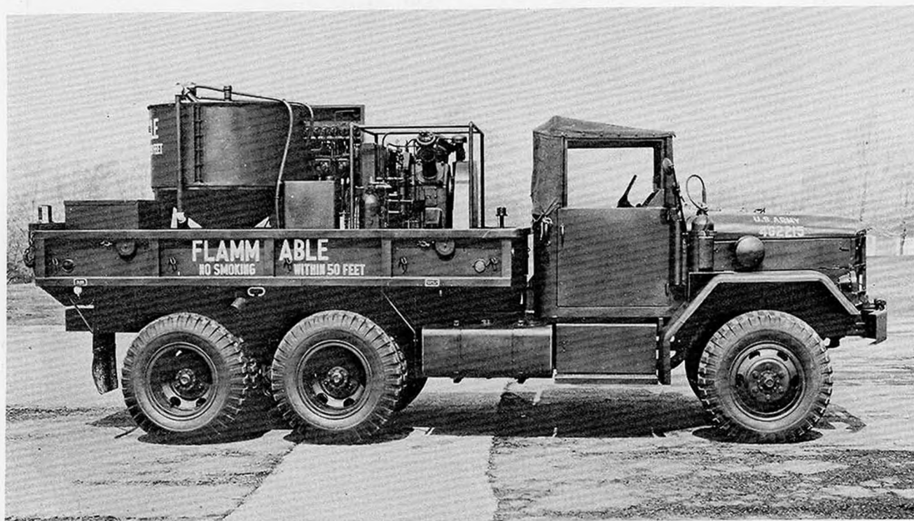
Figure 4-4. M4A2 truck-mounted flamethrower service unit.
