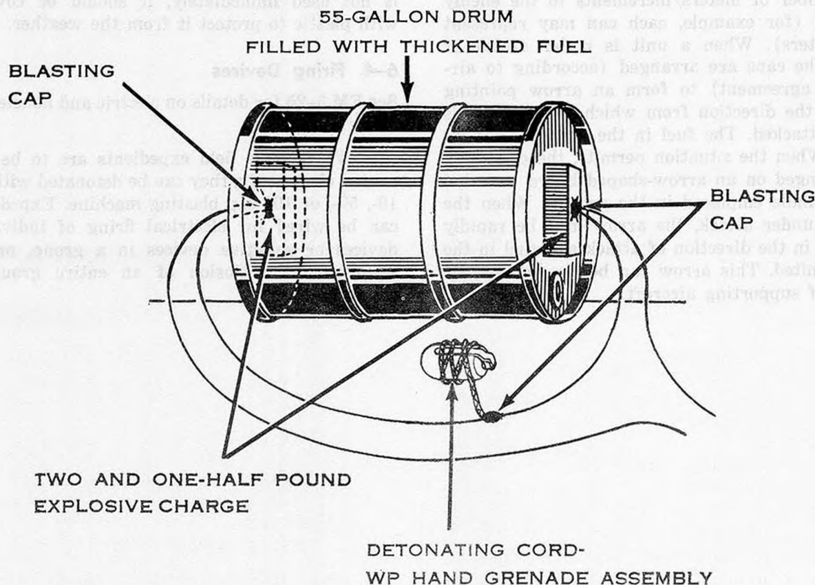
Figure 6-3. Exploding 55-gallon flame device (explosive charge).
