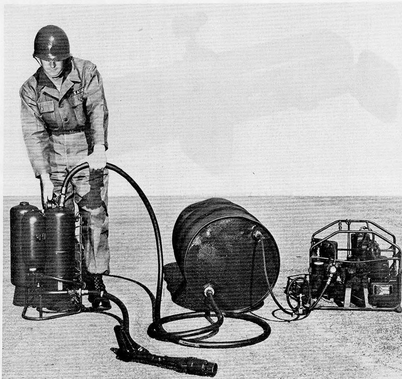
Figure 5-8. M27 service kit and AN-M4 compressor (3 1/2 CFM) used to fill a portable flamethrower from a 55-gallon drum of thickened fuel.
