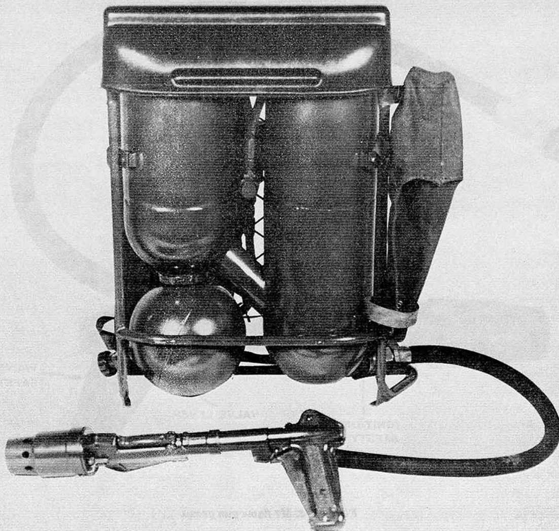
★Figure 5-3. M9A1-7 portable flamethrower.
