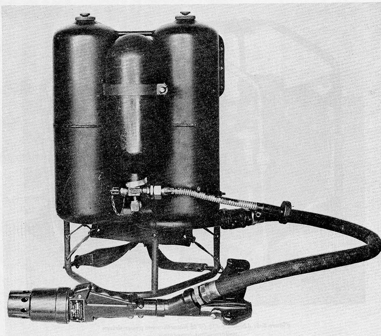
Figure 5-4. M2A1-7 portable flamethrower.
