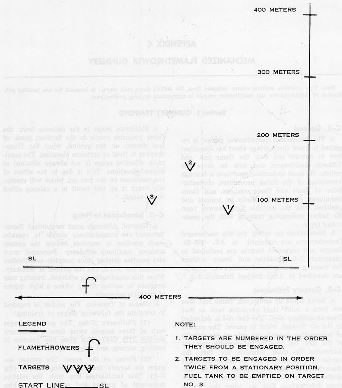
Figure C-1. Suggested layout for flame range, stationary firing.
