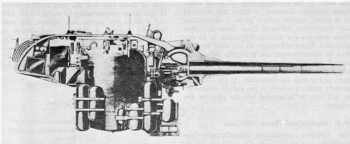
Figure 4-2. M7A1-6 mechanized flamethrower.
