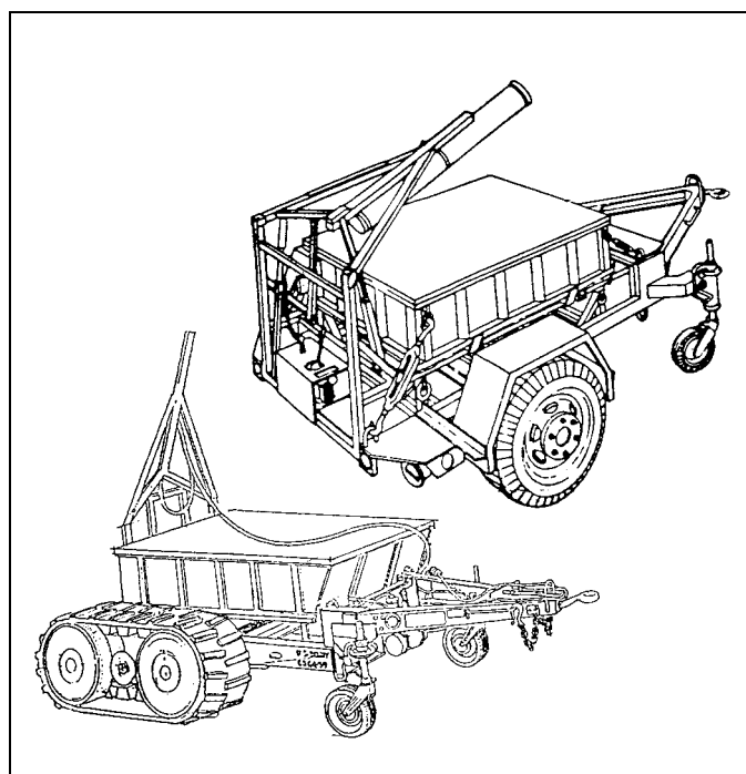
Figure 10-4. MICLIC
