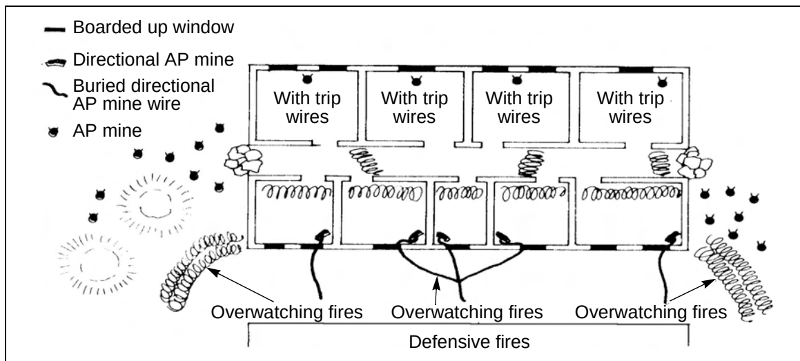
Figure 12-8. Building obstacles
