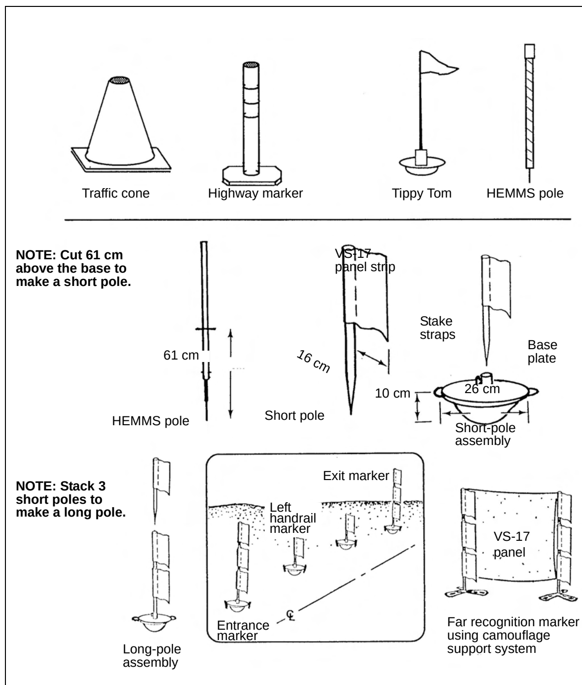
Figure 10-24. Marking devices
