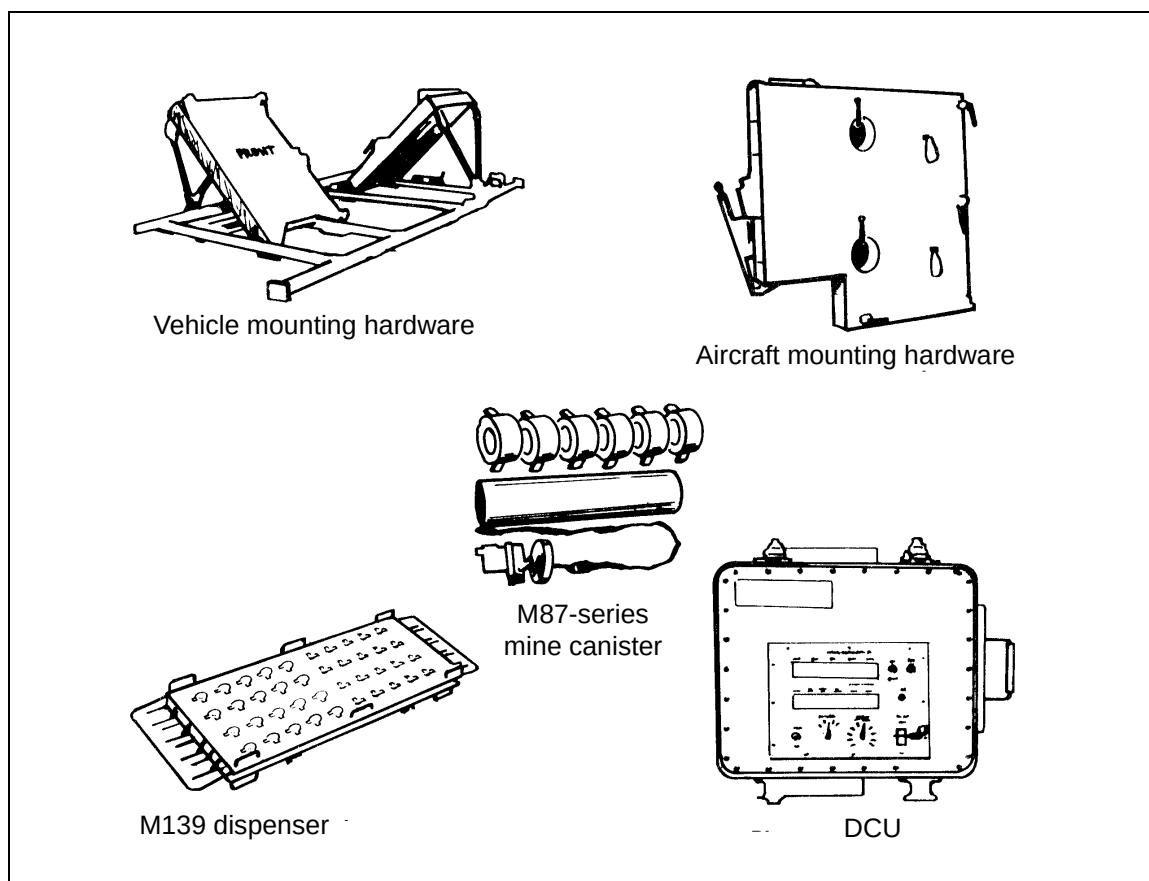
Figure 3-7. Volcano components
