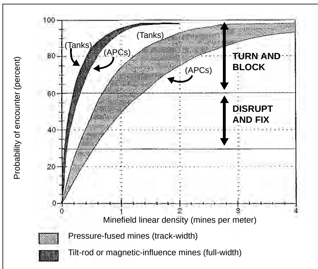
Figure 2-4. Vehicle mine encounter probability versus minefield density
