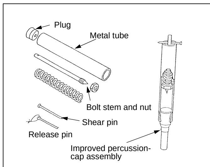
Figure 13-8. Improvised nonelectric FDs (spring-operated)
