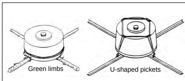
Figure 12-1. Outrigger techniques
