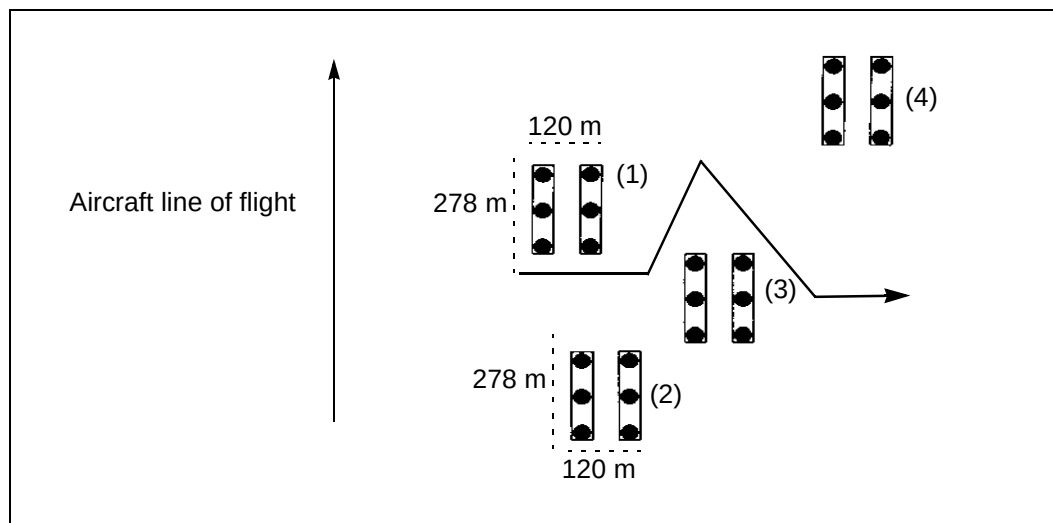
Figure D-5. Fix obstacle
