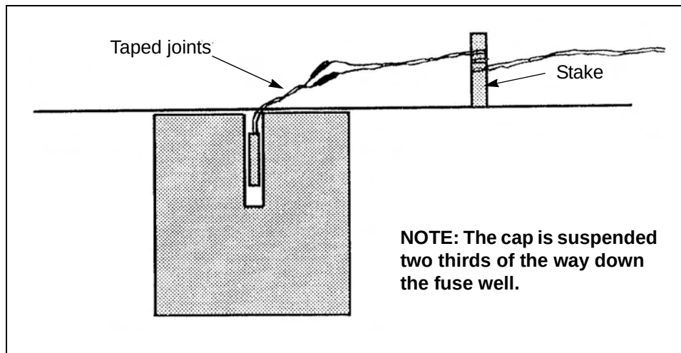
Figure E-1. M16 AP mine
