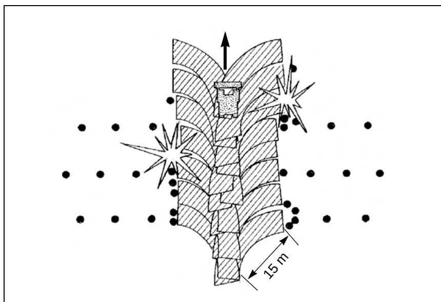
Figure 10-11. Skim technique
