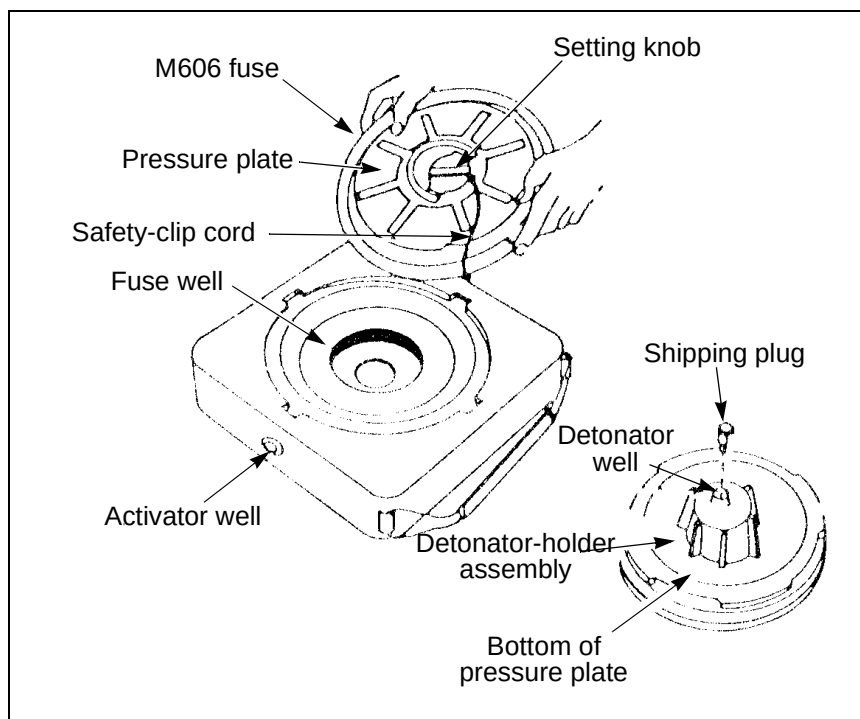
Figure A-27. Removal of the pressure plate
