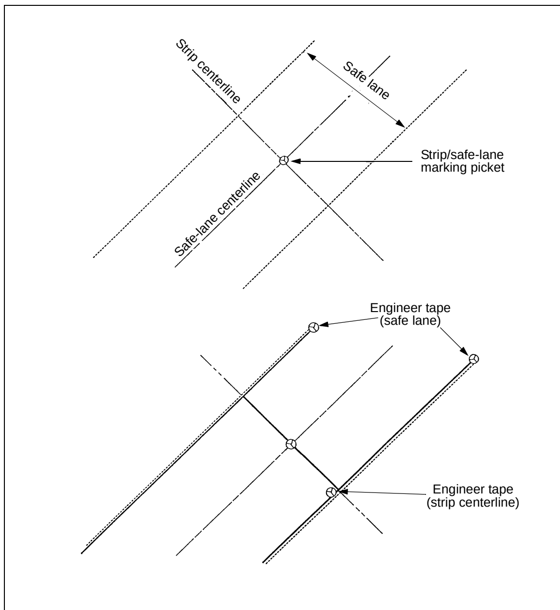
Figure 7-9. Lane closure
