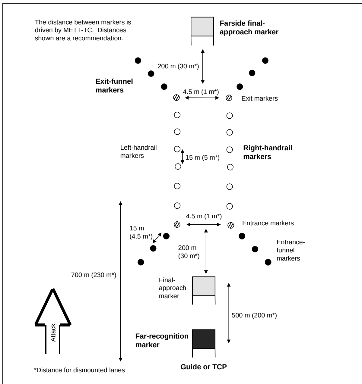
Figure 10-22. Intermediate lane marking
