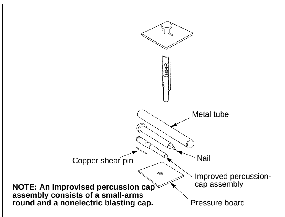
Figure 13-7. Improvised nonelectric FDs (shear-pin operated)
