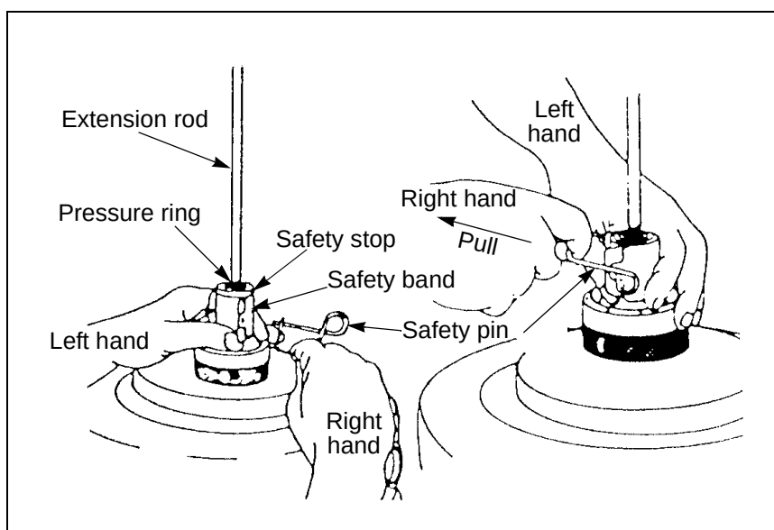
Figure A-20. Removal of safety pin
