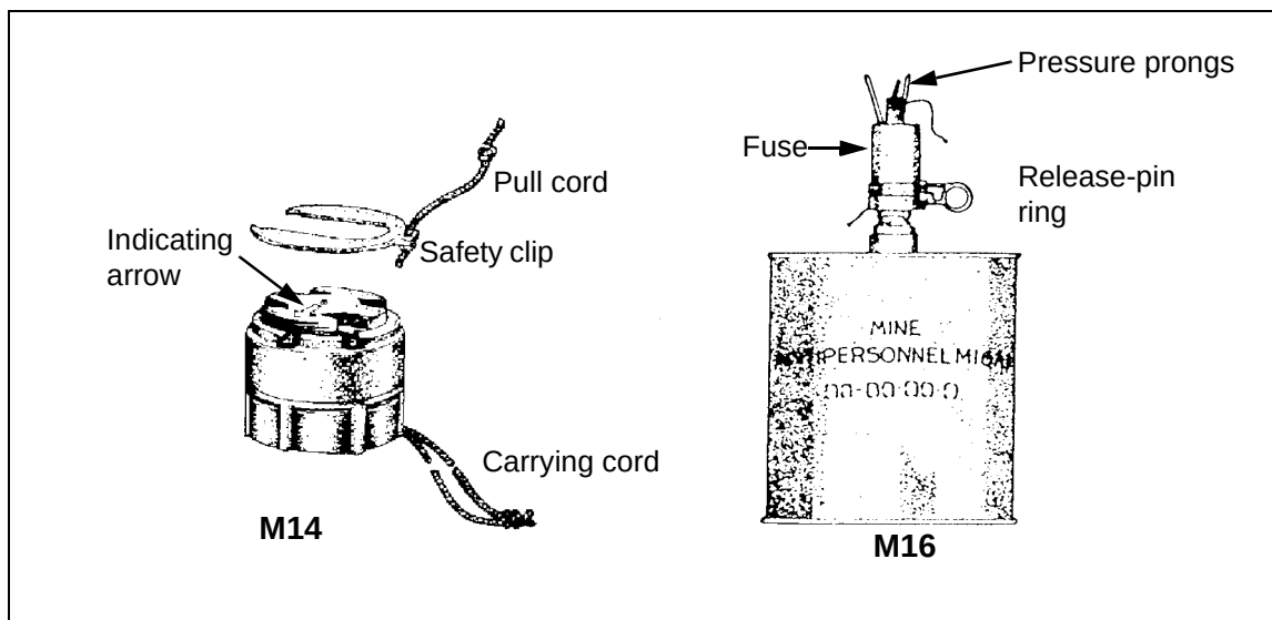
Figure 5-2. AP mines
