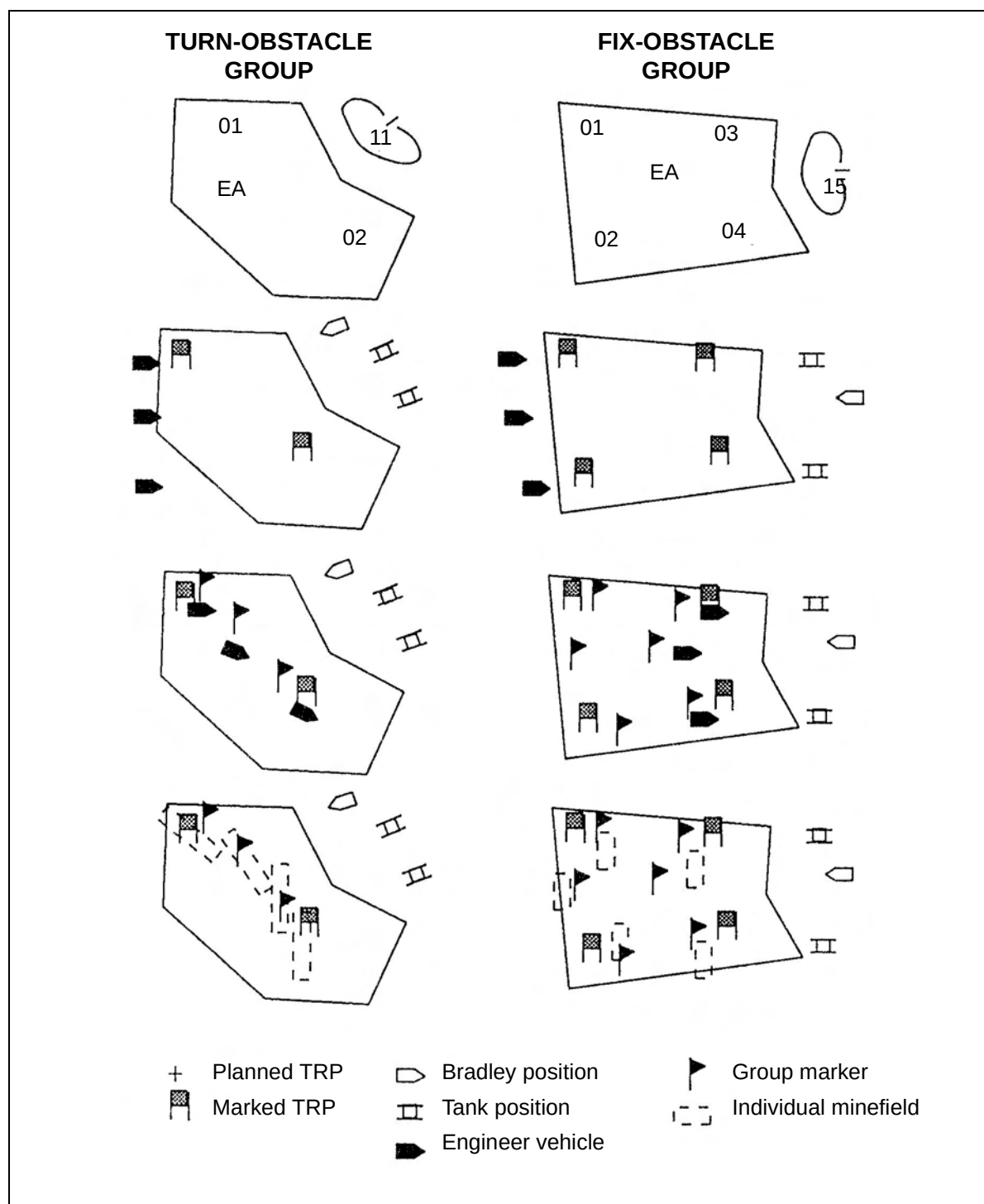
Figure 2-18. Minefield siting
