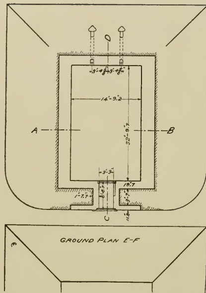
FIG. 141. Magazine of Carbonite Explosives Co., Schlebusch (From Bureau of Mines Technical Paper, No. 18)
