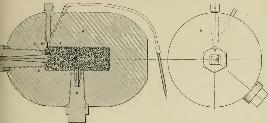
FIG. 84. Noble and Abel's Bomb
