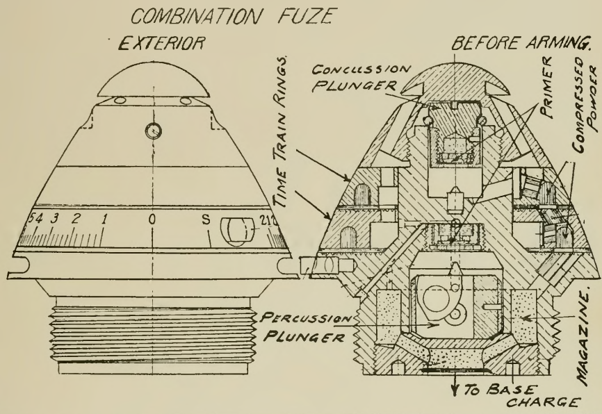
FIG. 119. Time and Percussion Fuze
