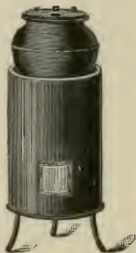
FIG. 143. Heat Test Bath (from Baird and Tallock's Catalogue )
