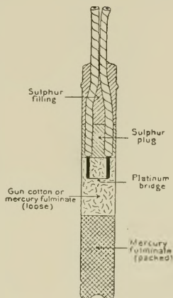
FIG. 117. Electric Detonator
