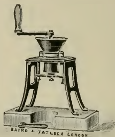
FIG. 145. Mill for Cordite
