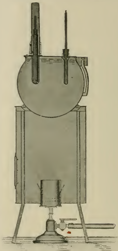
FIG. 14s. Heat Test Bath Assembled (From First Report of Heat Test Committee, by permission of the Controller of H.M. Stationery Office)
