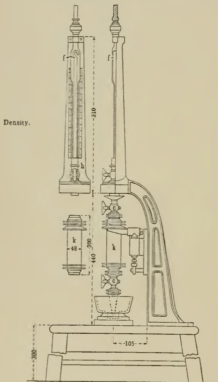
FIG. 79. Bianchi's Densimeter
