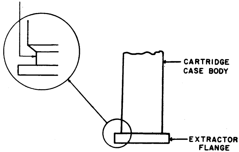
Figure 2. Rimmed Cartridge Case
