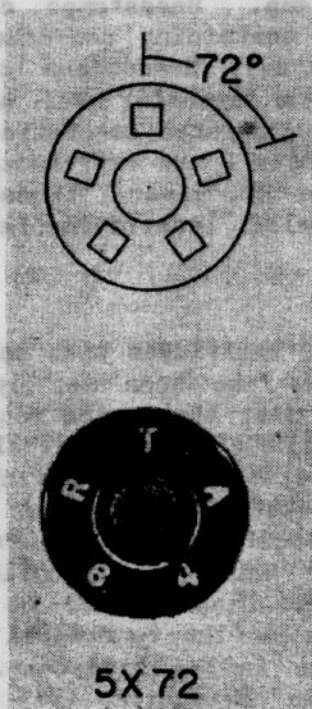
Figure 13. Five-Element Headstamp
