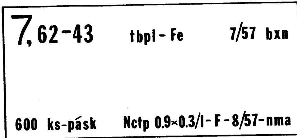
Figure 22. Czechoslovak Sheet-Metal Container Markings, 7.62x39 Ball Cartridges in Clips
