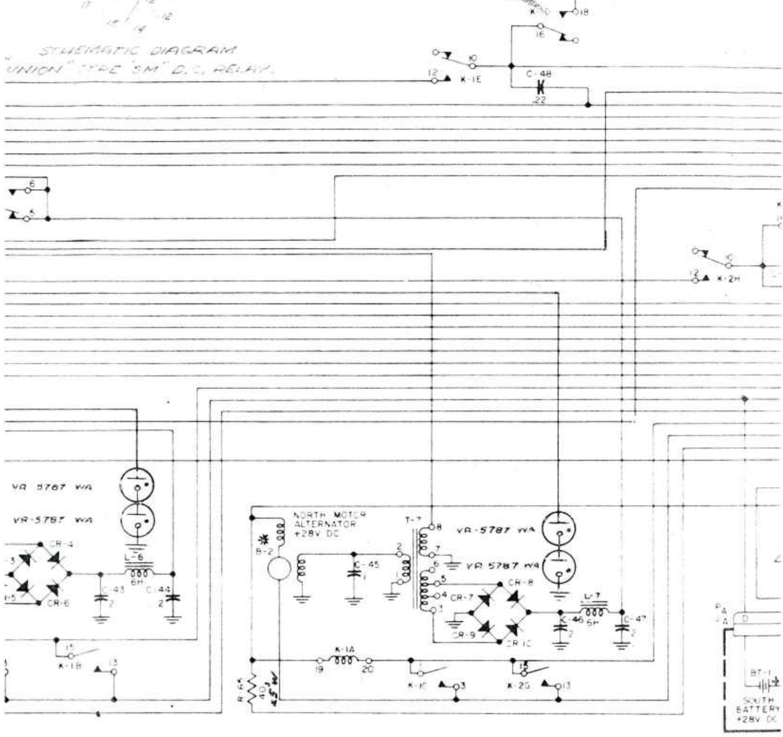
Figure 34. T3008E5
