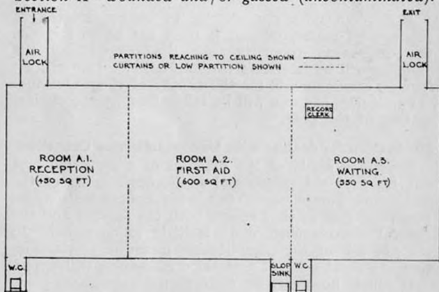
FIG. 1.—Lay-out of Section A—First Aid (Uncontaminated Casualties) for one sex. 1 Sizes are given for a large Post.
