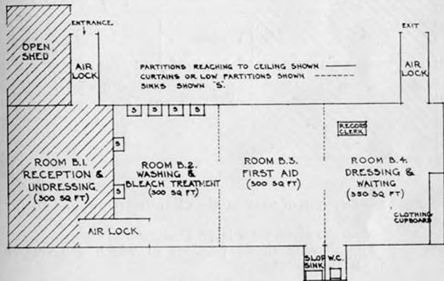
FIG. 2.—Lay-out of Section B—First Aid (Contaminated Casualties) for one sex. Sizes are given for large Post. The shading shows portions in which gas vapour might collect.
