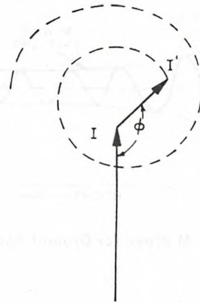
Figure 3-4 (U). Vector Diagram for Changes in Antenna Current
