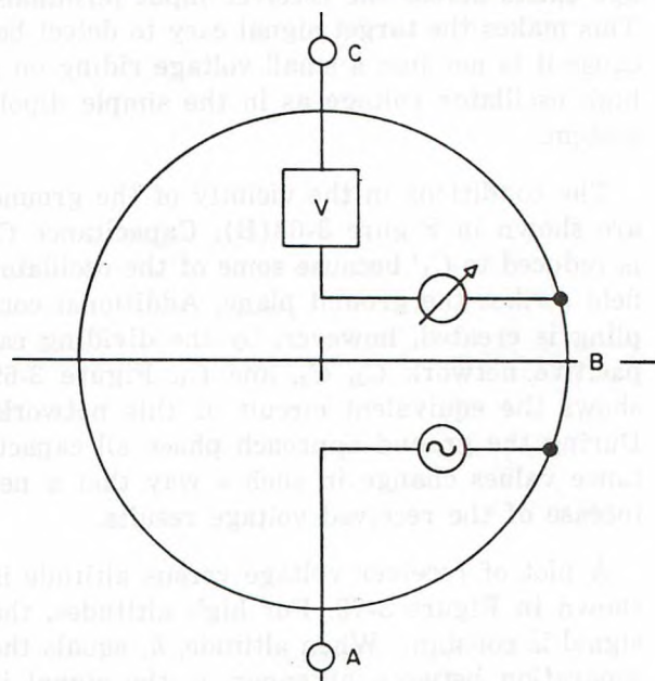
Figure 3-67 (C). Vertical Antenna Configuration for Fuze (U)
