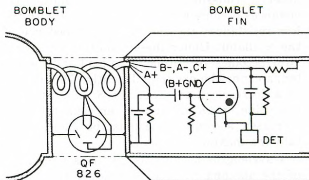
Figure 3-66 (U). Radio Induction Field Fuze
