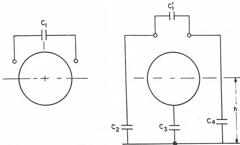
Figure 3-73 (C). Horizontal Antenna Configuration, Rear Mounted (U)
