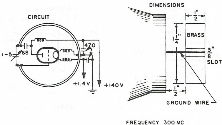
Figure 3-23 (S). Transverse Loop Oscillator with Small Diameter Cylindrical Resonant Circuit (U)
