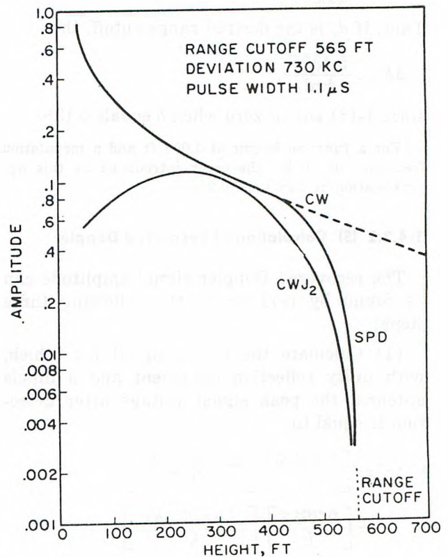
Figure 3-62 (C). Comparison of CWJ 2 and SPD Signal Return from Ground Target (565-ft Range Cutoff) (U)
