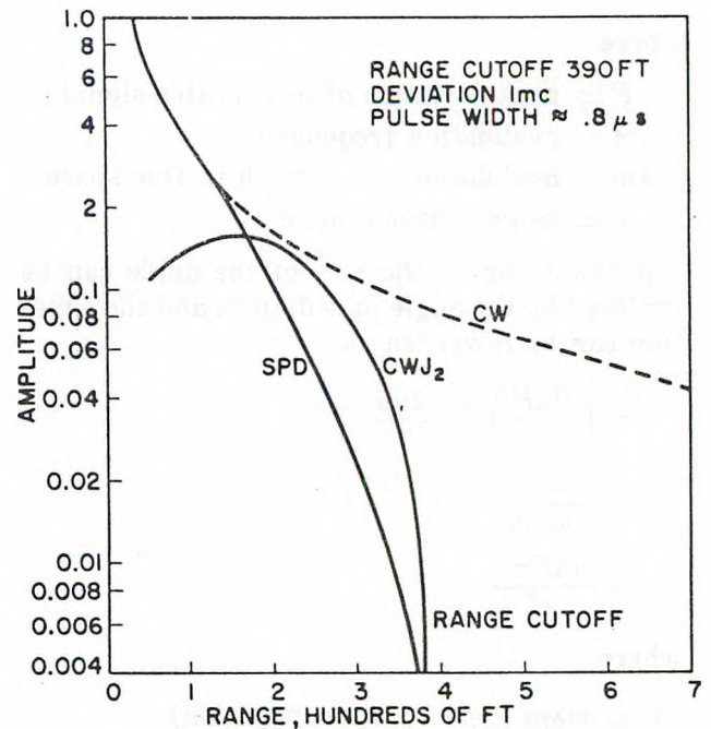
Figure 3-61 (C). Comparison of CWJ 2 and SPD Signal Return from Ground Target (390-ft Range Cutoff) (U)
