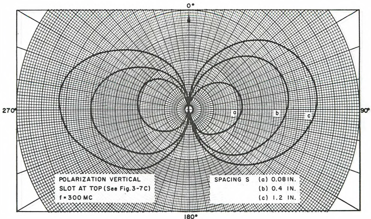
Figure 3-17 (S). Radiation Patterns for Transverse Loop Antenna (Oscillator, Figure 3-16) as Spacing Between Loop and Body is Changed (U)
