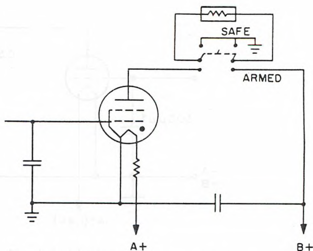
Figure 3-46 (U). Basic Firing Circuit
