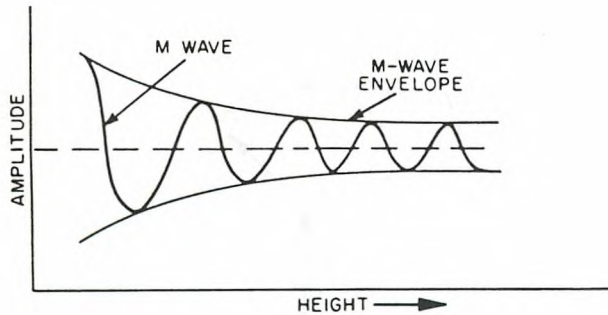
Figure 3-5 (U). M Wave for Ground Approach Case
