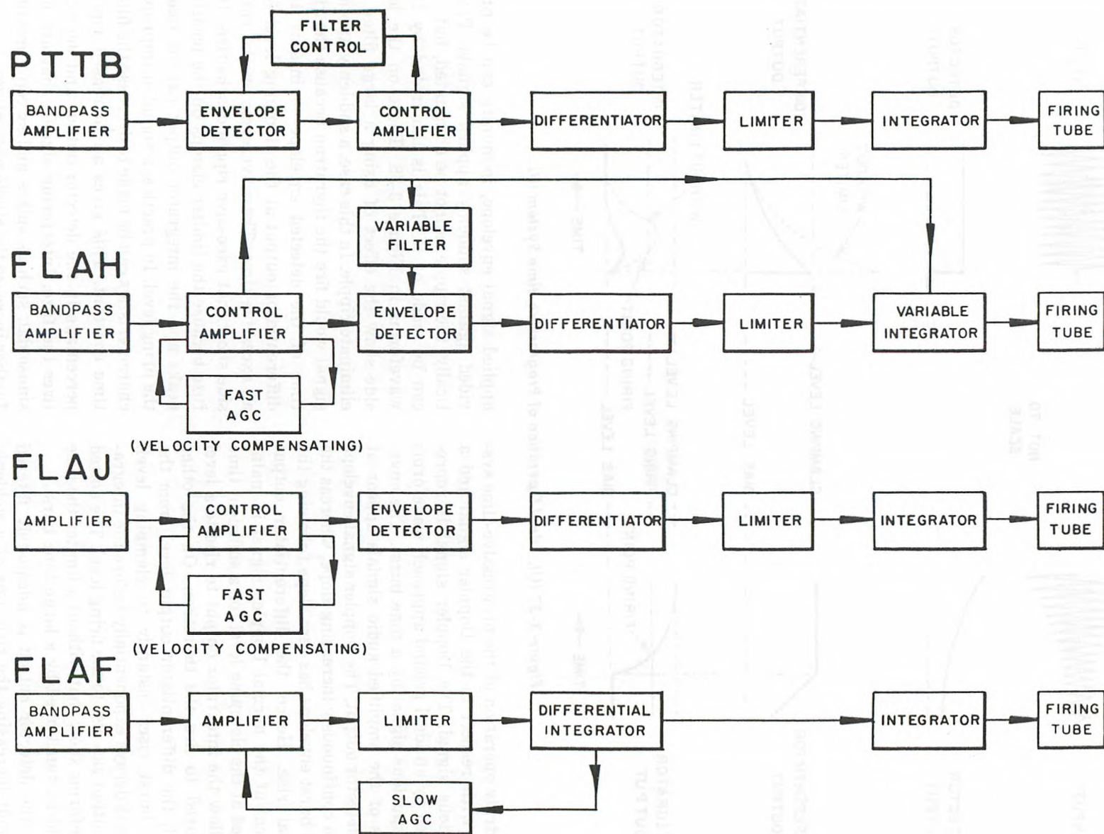
Figure 3-36 (S). Block Diagrams of PTTB, FLAH, FLAJ, and FLAF Integrating Amplifiers (U)
