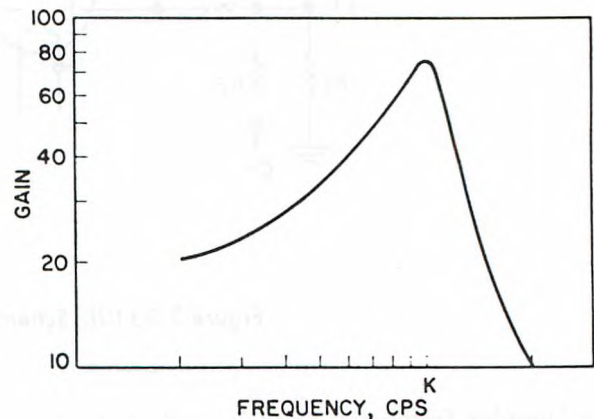
Figure 3-32 (U). Response Curve of Peaked Amplifier
