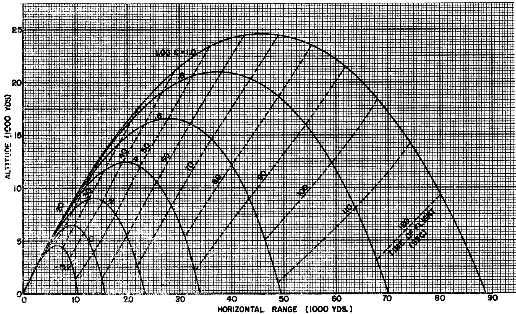
Figure 6 (4 of 12). Trajectories for Projectile Type 2, 45° elevation, 3600 fps muzzle velocity
