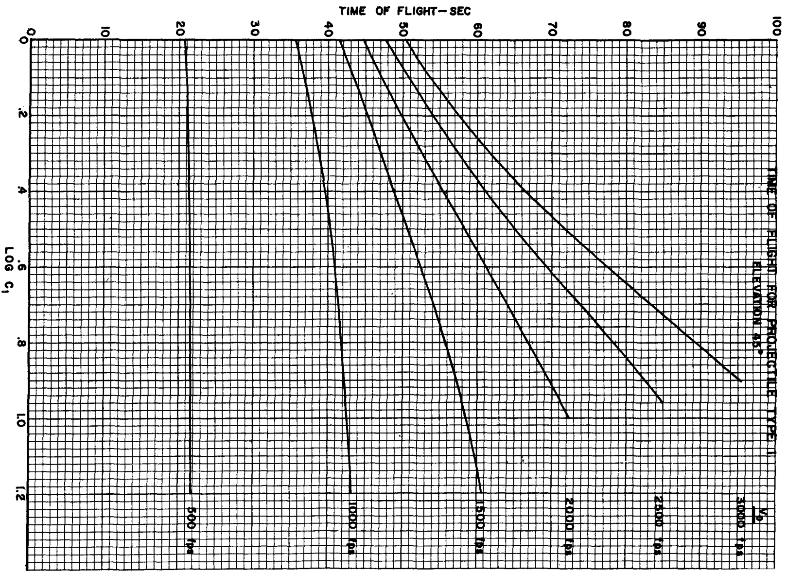
Figure 3. Time of Flight for Projectile Type I
