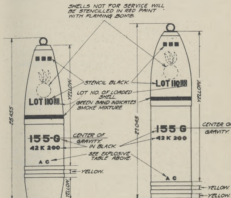
155 MM. C.S. SHELL MARK V
