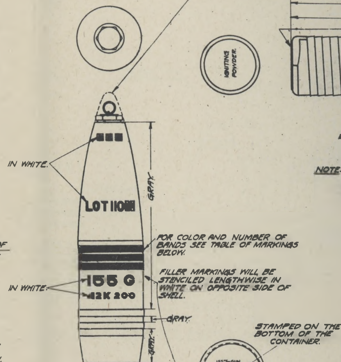
155MM.C.S. SHELL MARK
