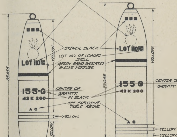
155 MM C.S. SHELL MARK III
