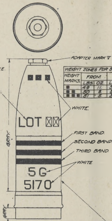
5 IN. COMMON STEEL SHELL MARK II
