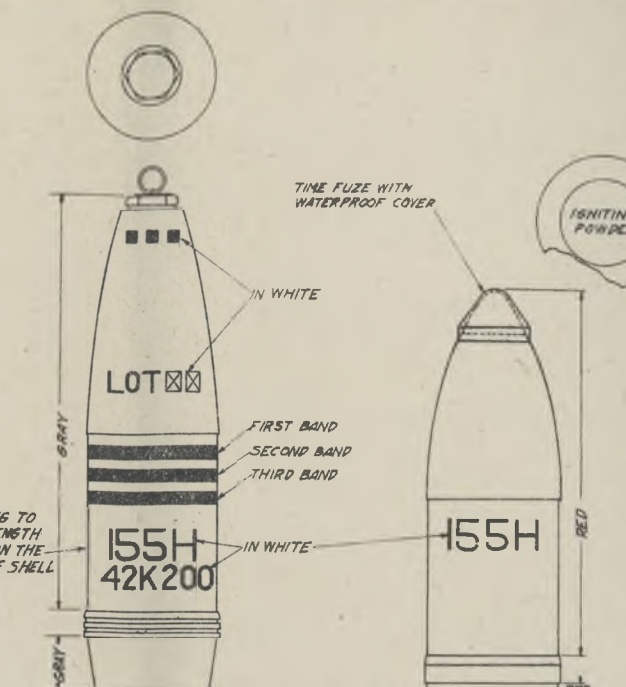
155mm COM. STEEL SHELL MARK II GAS
