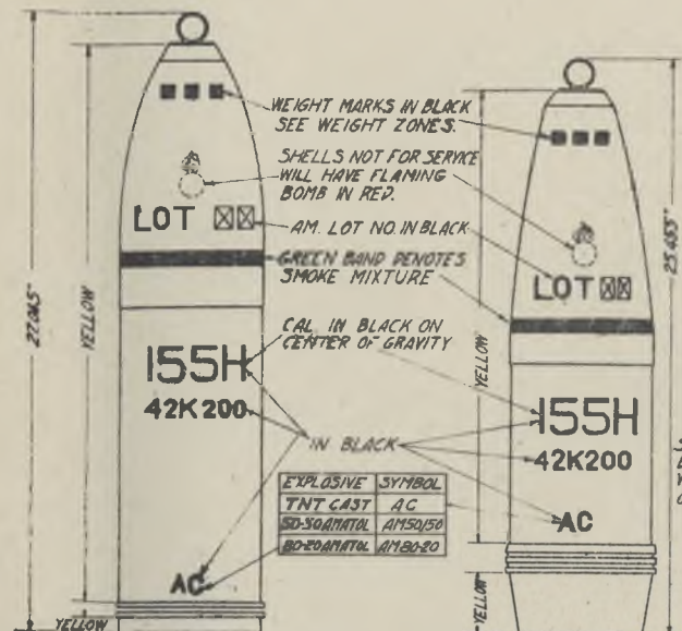
155mm COM. STEEL SHELL MARK II
