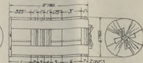
CARTRIDGE BAG FOR 155mm HOW (SCHNEIDER) MOD '17.
