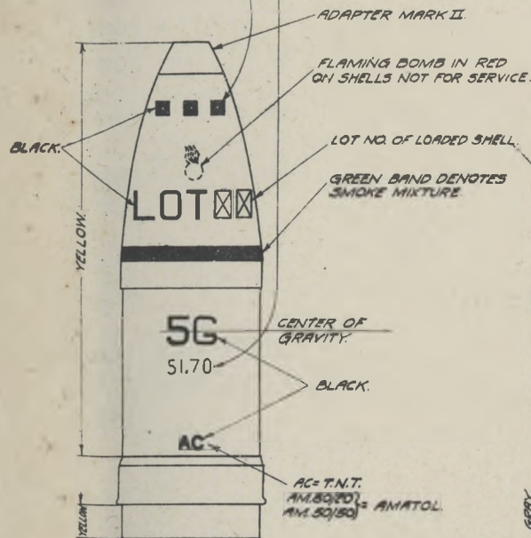
5 IN. COMMON STEEL SHELL MARK II
