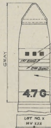
4.7* COMMON STEEL SHELL MARK II (GAS) FIXED
