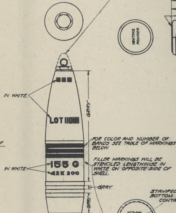
155 MM C.S. SHELL MARK
