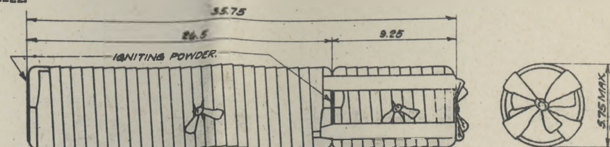
CARTRIDGE BAG FOR 155 MM GUN
