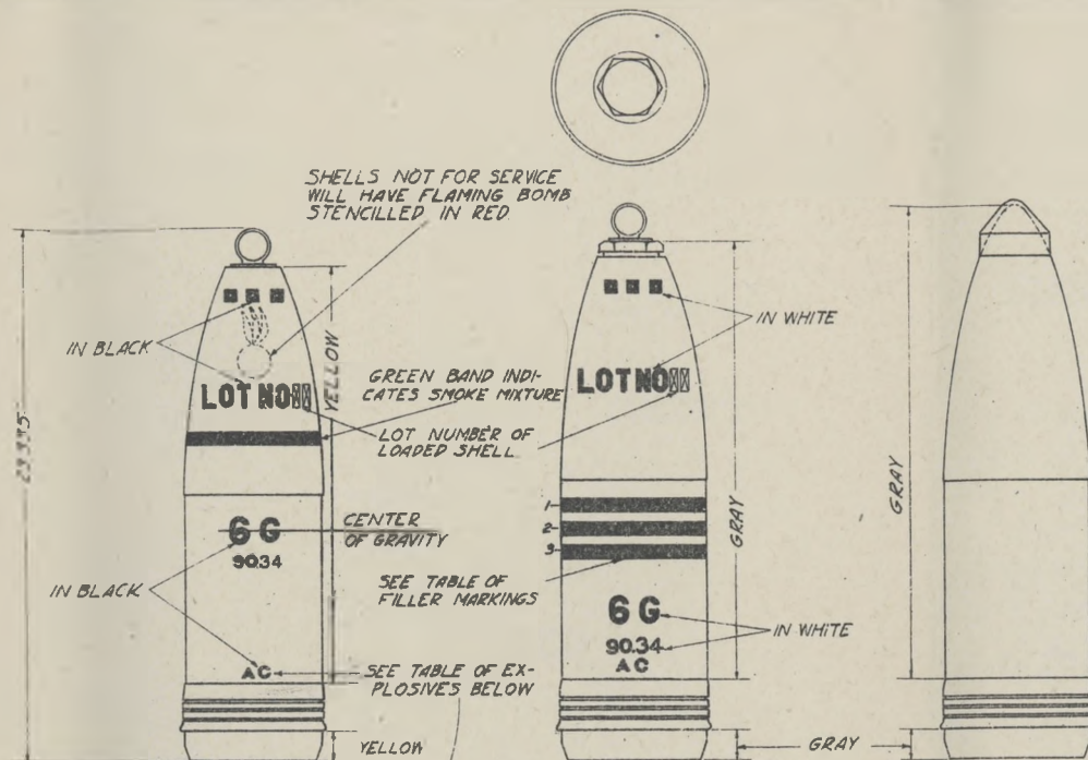
GIN.COM STEEL SHELL MARK II
