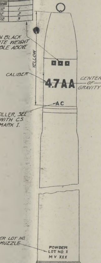
4.7" ANTI-AIRCRAFT SHRAPNEL MARK I FIXED
