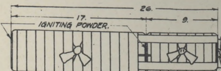
CARTRIDGE FOR 5 IN. S.C. GUN MODEL 1897. MAXIMUM CHARGE 18 LBS. 6 BASE SECTION 12 LBS. INCREMENT SECTION 6 LBS. MINIMUM CHARGE 9 LBS. BASE SECTION 6 LBS. INCREMENT SECTION 3 LBS.
