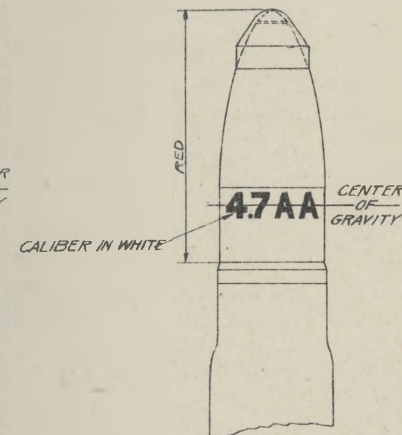
4.7" ANTI-AIRCRAFT SHRAPNEL MARK I FIXED
