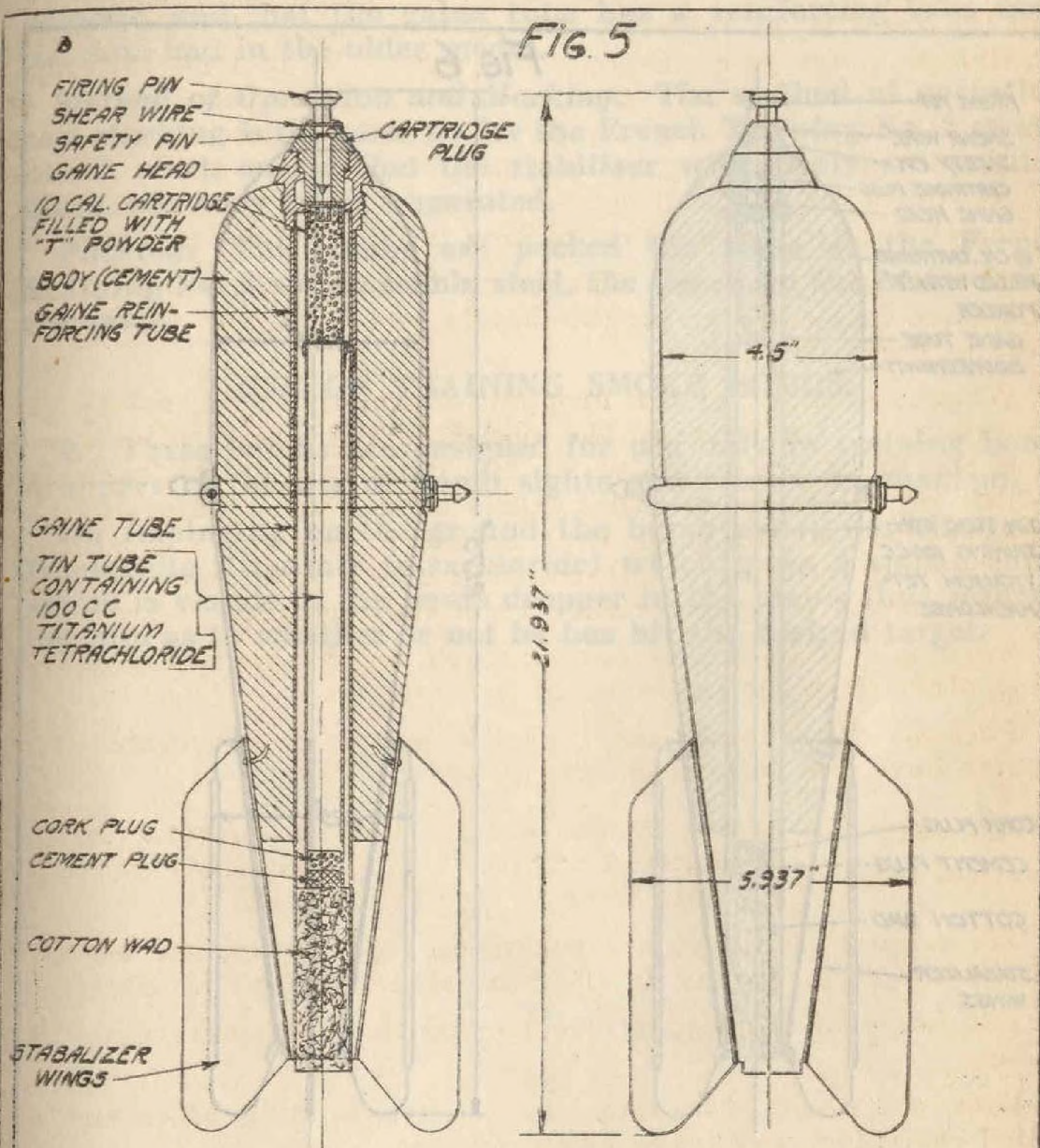
FRENCH TRAINING SMOKE BOMB - CEMENT (BOMBE A' FUMEE' EN CIMENT)
