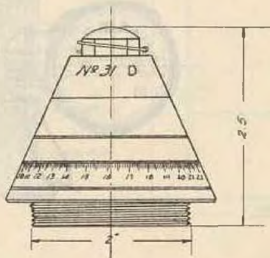
FUSE 31-D FOR STOKES MORTAR BOMB
