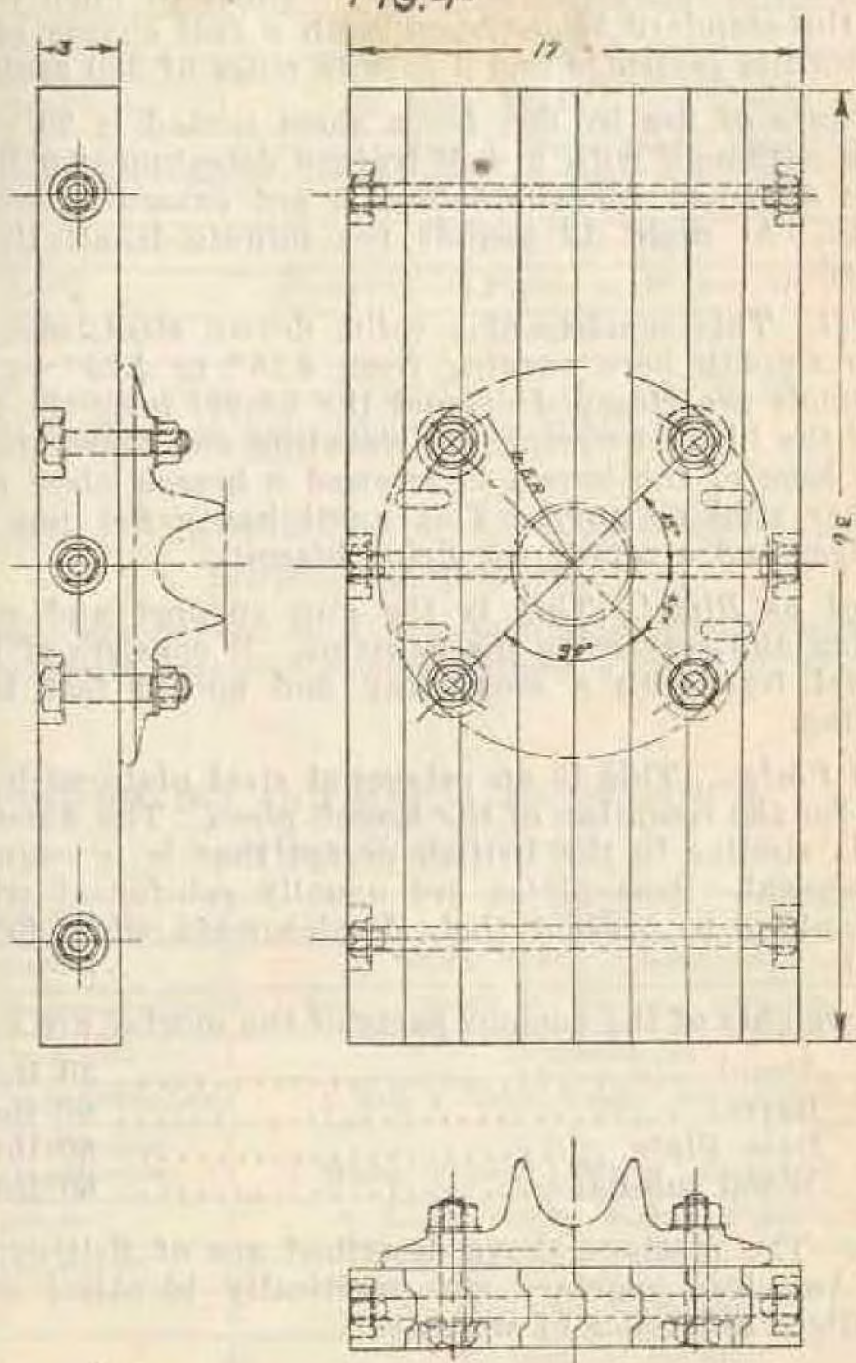
AMERICAN 4" Stokes MORTAR - MARK I - SUB BASE DEB OFFENSE DIVISION ENG SEC G.W.S. 5580
