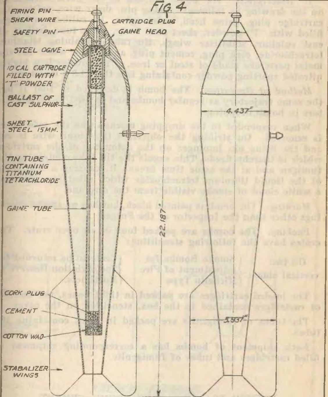
FRENCH TRAINING No 2 SMOKE BOMB STEEL
