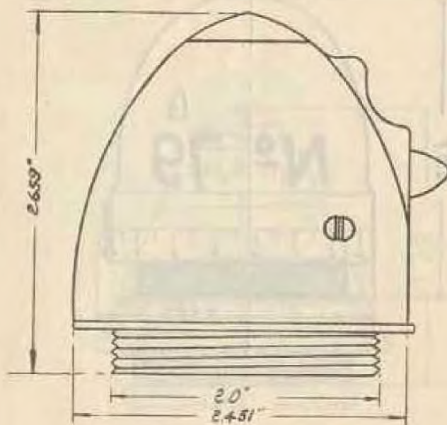
AMERICAN TRENCH MORTAR FUSE MARK XI
