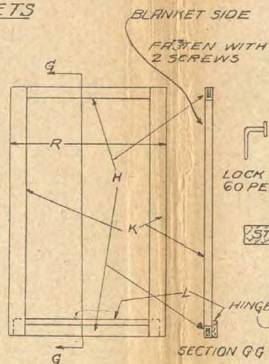
N°5 EXTERIOR BLANKET FRAME USED AS IN N°2 H=1x4 BLANKET COVERED. K=1x6 BLANKET COVERED L=1x6 PLAIN R=4' FOR DRESSING STATIONS
