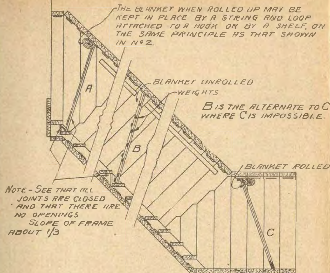
N°1 ARRANGEMENT OF GAS BLANKETS
