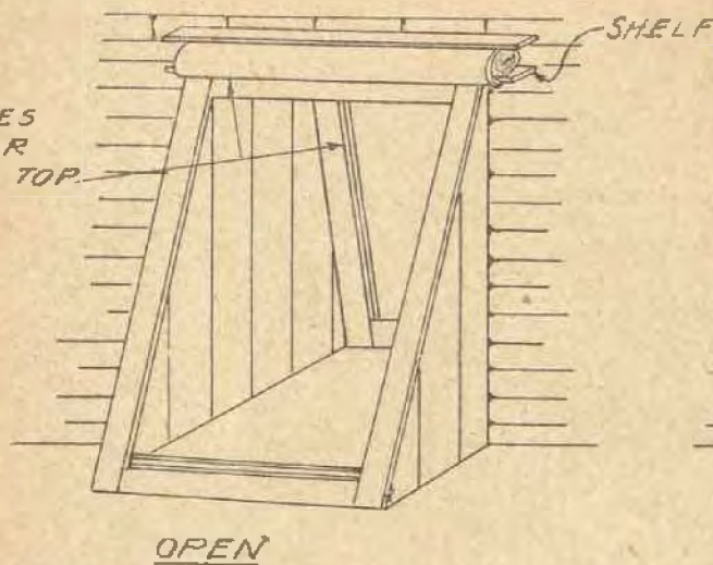
N°2 PROJECTING ENTRANCE USED SOMETIMES IN DRESSING STATIONS TO AVOID NARROWING PASSAGE
