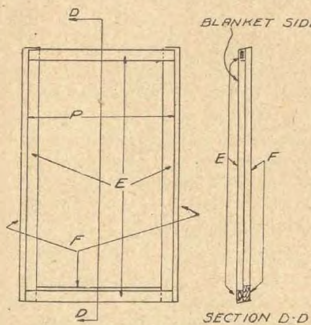
N°4 INTERIOR BLANKET FRAME USED AS IN "C" OF N°1 AND IN N°3 E=1x4 BLANKET COVERED. F=1x6 PLAIN. P=2'-8" TO 3'-8"
