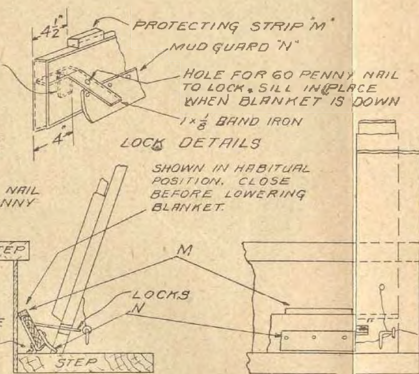
N°6 (OPTIONAL) DETAIL OF INTERIOR FRAME BOTTOM WHEN FRAME IS USED AS IN "A+B" OF N°1 M=1x2 PLAIN, PROTECTING STRIP N=LEATHER OR RUBBER MUD GUARD
