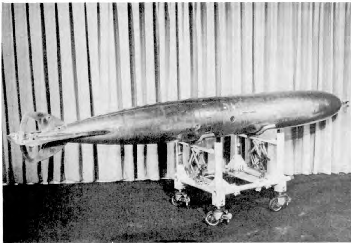
Figure 11. Howell Torpedo
