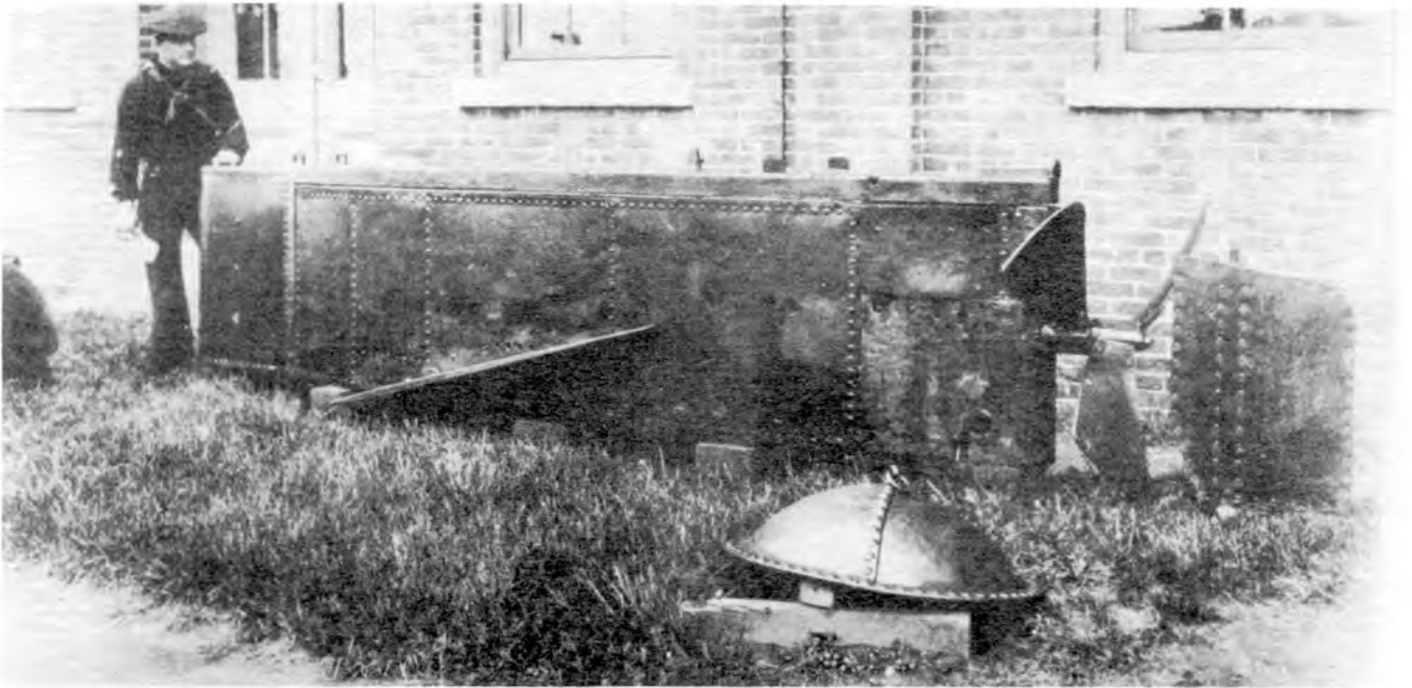
Figure 7. Ericsson Torpedo
