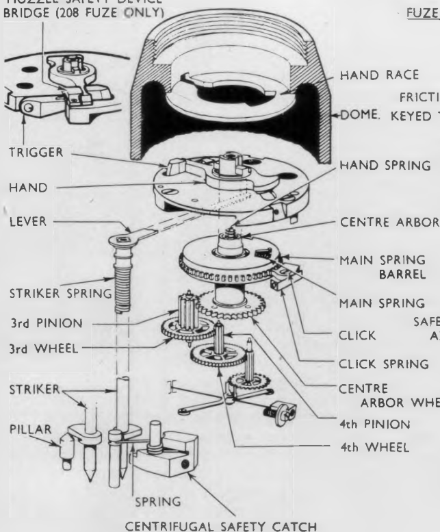
CLOCKWORK MECHANISMS OF TIME FUZZES
