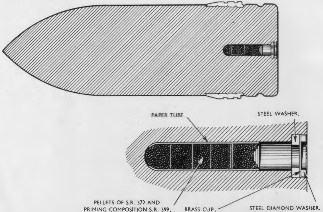
METHOD OF FILLING TRACER CAVITY TYPE L.54.
